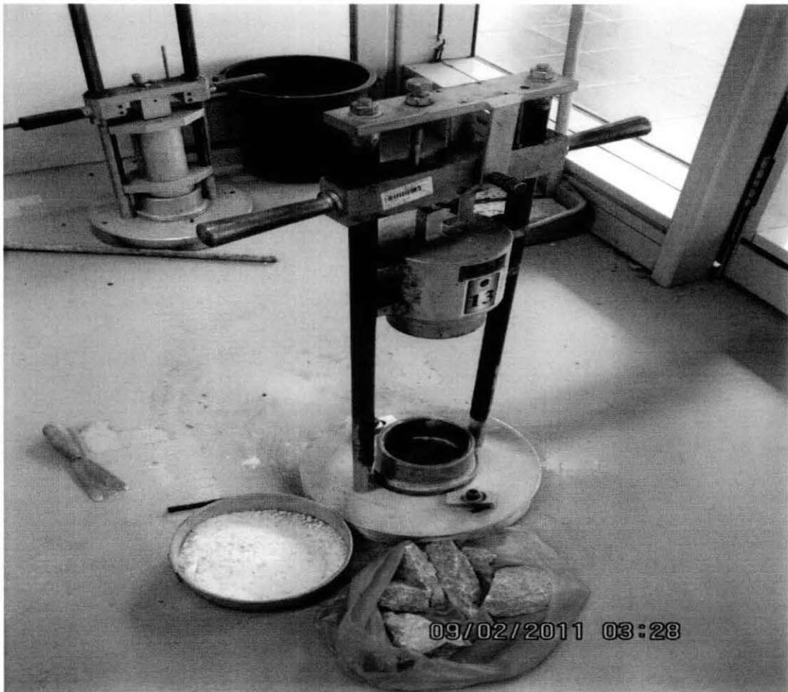
Figure 3: Aggregate Impact Value Test machine (AIV), civil engineering lab, blocks13.
