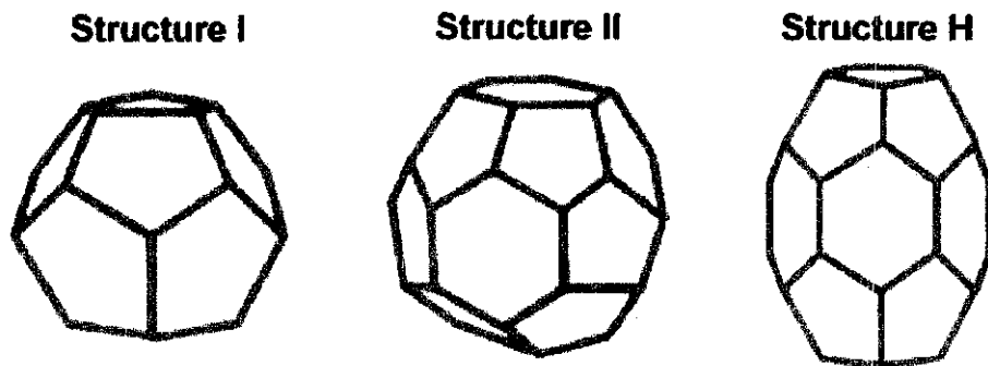
Figure 2.2: Schematic of structure I, II, and H hydrates
