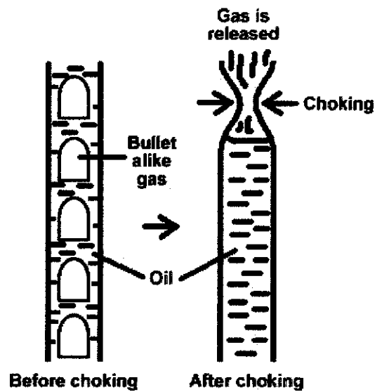
Figure 2.9: Choking at riser top
