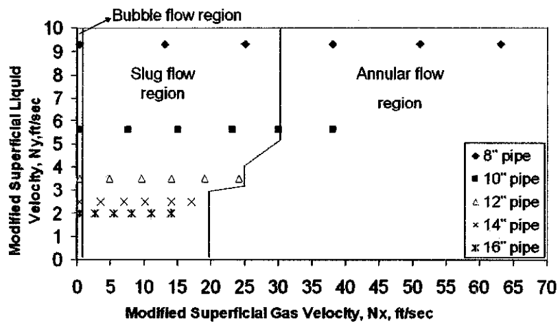
Figure 4.1h: Vertical flow for different internal pipeline diameters at 13,000 bpd
