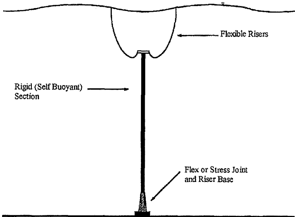
Figure 7.2: Hybrid riser
