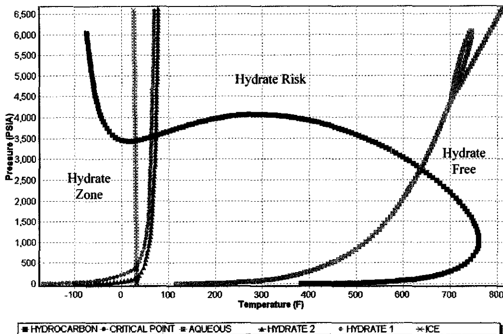
Figure 4.2d: Phase envelope plot with 50% bbl/bbl of water fraction
