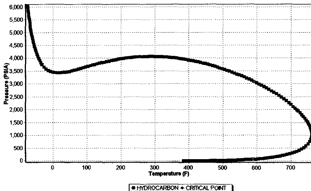
Figure 4.2a: Phase envelope plot with 0% bbl/bbl of water fraction
