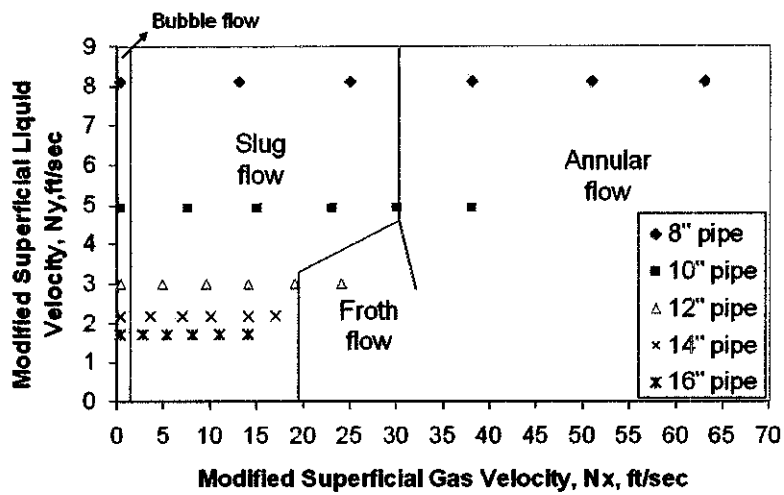
Figure 4.1g: Vertical flow for different internal pipeline diameters at 11,000 bpd
