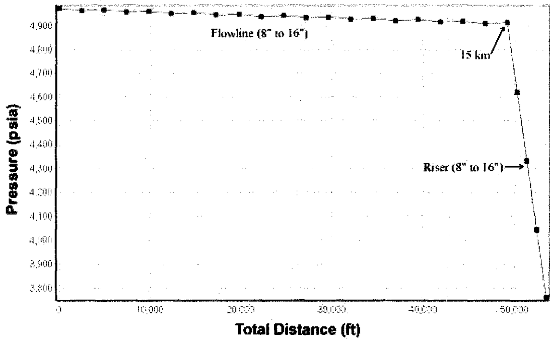
Figure 4.3c: Fluid pressure at different flowline and riser diameters
