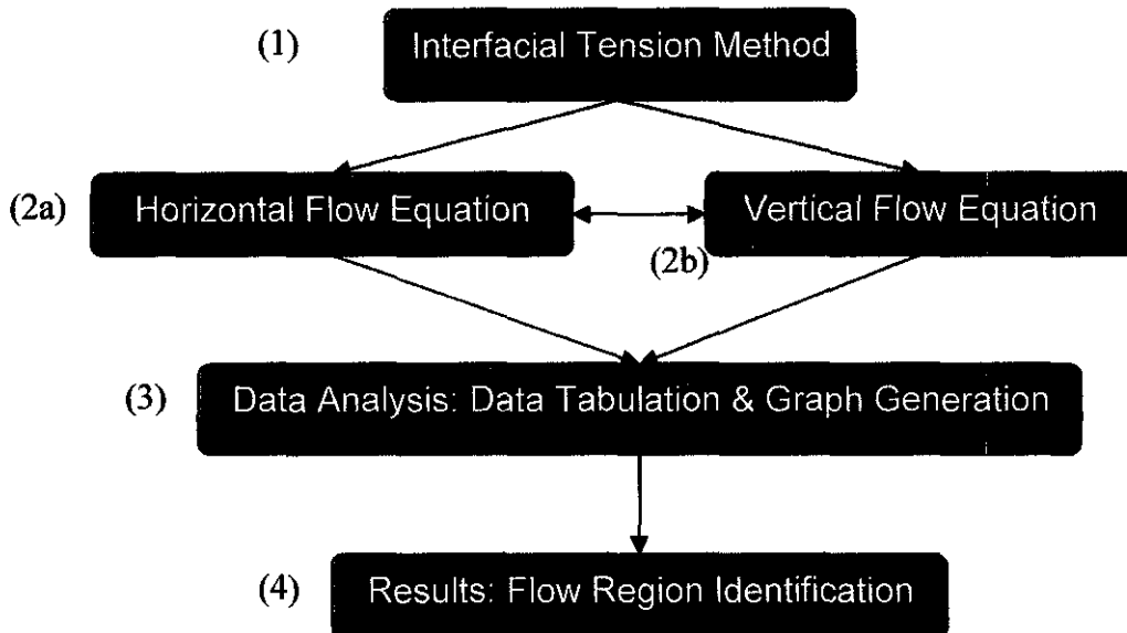
Figure 3.1: Steps of identifying flow patterns
