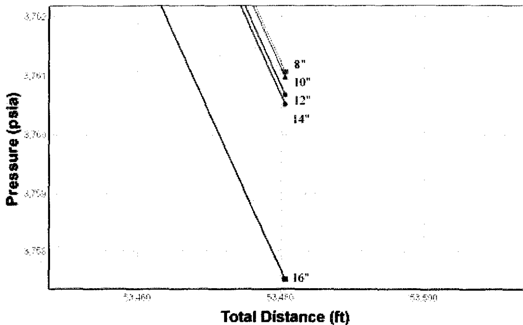
Figure 4.3d: Fluid pressure at different riser diameters
