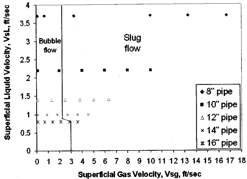
Figure 4.1e: Horizontal flow for different internal pipeline diameters at 17,000 bpd
