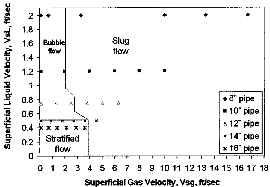
Figure 4.1a: Horizontal flow for different internal pipeline diameters at 9,000 bpd
