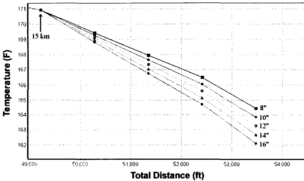
Graph 4.3b: Fluid temperature at different riser diameters
