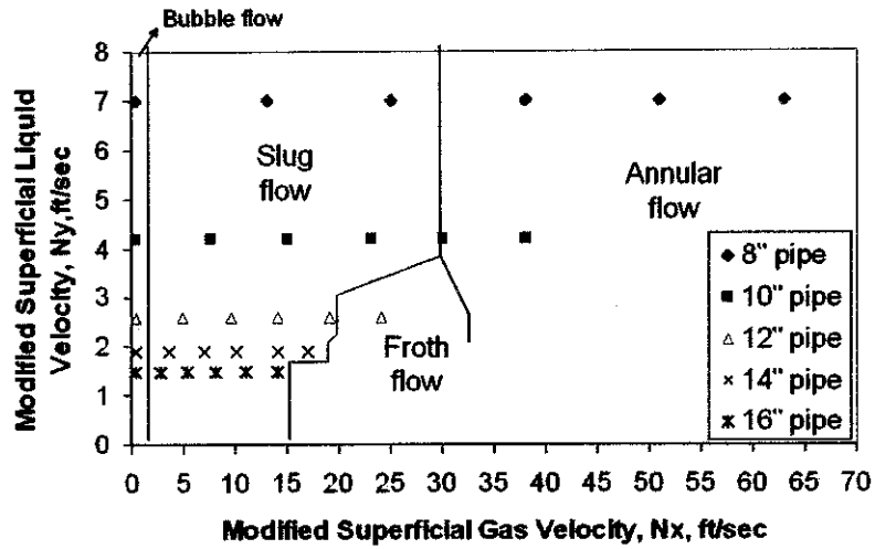
Figure 4.1f: Vertical flow for different internal pipeline diameters at 9,000 bpd
