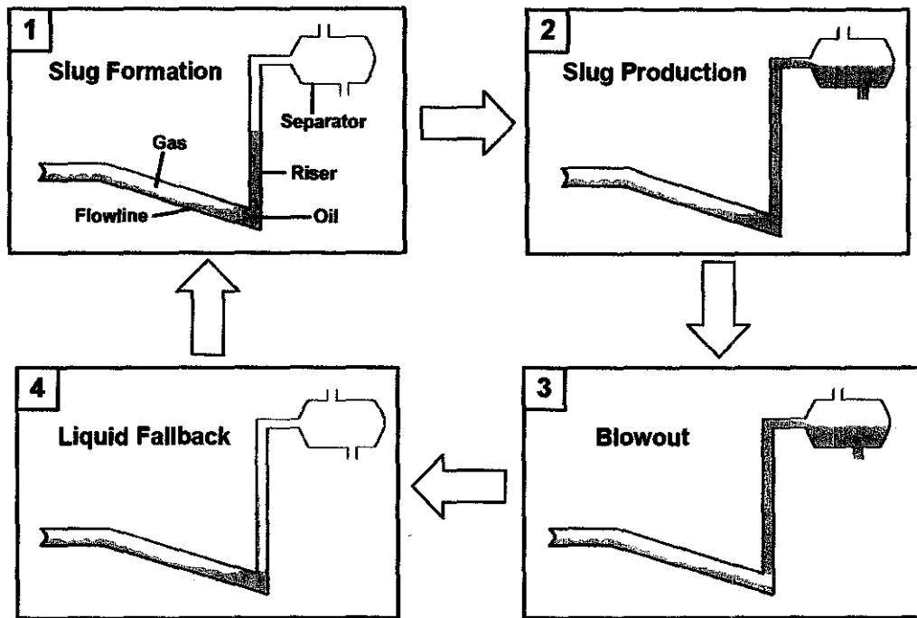
Figure 2.8: Schematic diagram of severe slugging process
