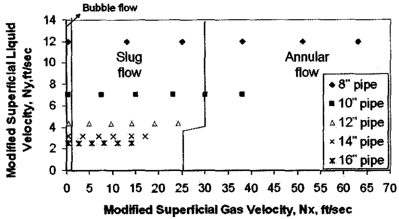
Figure 4.1i: Vertical flow for different internal pipeline diameters at 15,000 bpd
