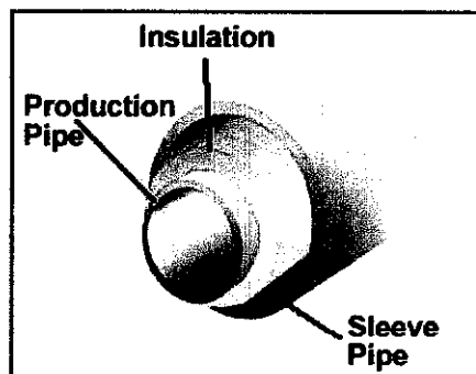
Figure 2.5: Pipe-in-pipe method
