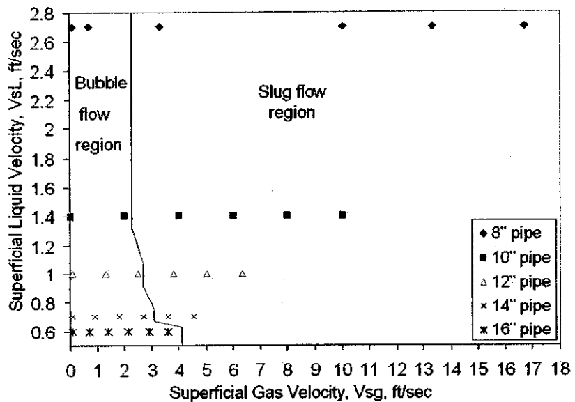
Figure 4.1c: Horizontal flow for different internal pipeline diameters at 13,000 bpd
