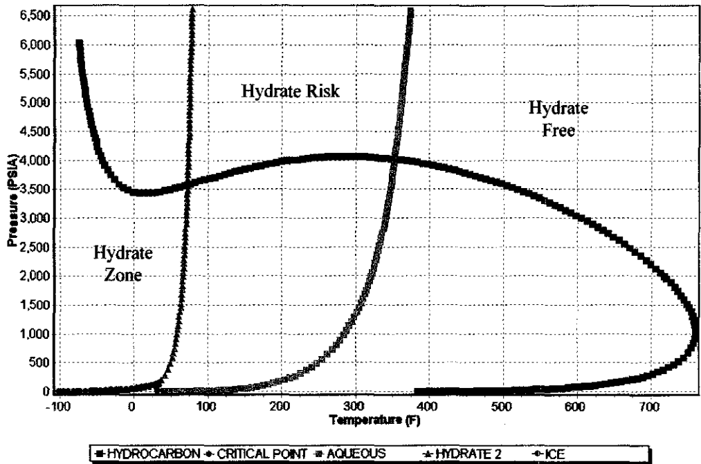
Figure 4.2c: Phase envelope plot with 0.8% bbl/bbl of water fraction
