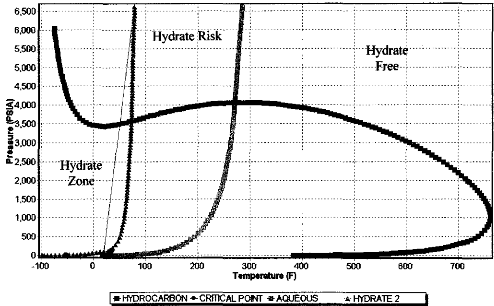
Figure 4.2b: Phase envelope plot with 0.1% bbl/bbl of water fraction
