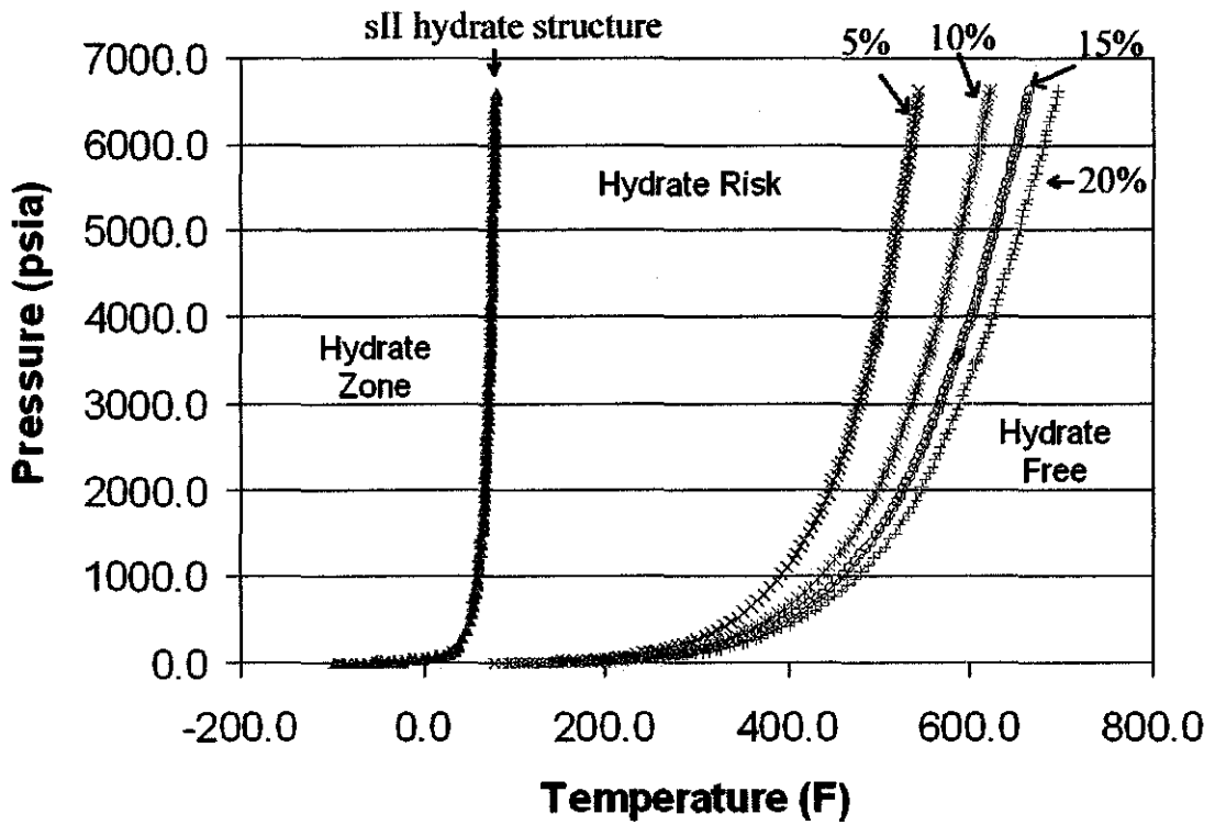
Figure 4.2e: The effect of 'Hydrate Risk' region expansion due to increasing water fraction
