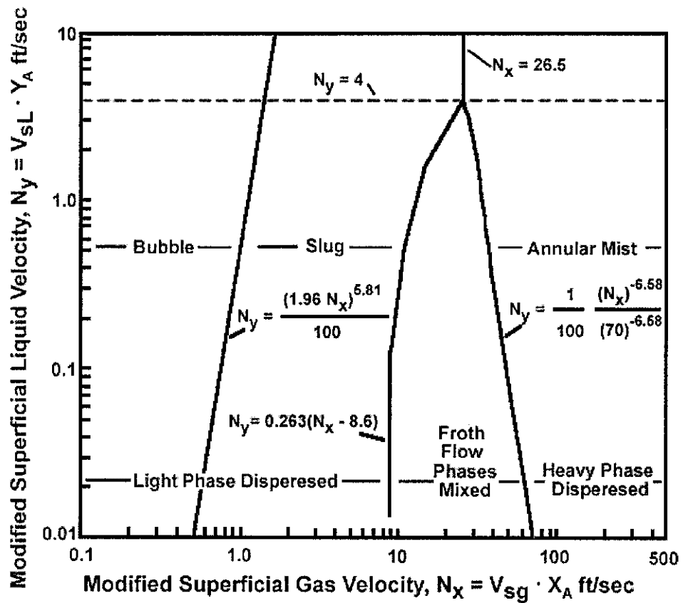
Figure 2.7: Aziz et al. vertical flow regime map
