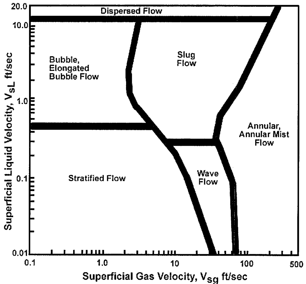
Figure 2.6: Mandhane et al. horizontal flow regime map
