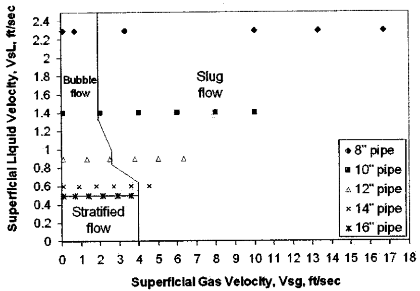
Figure 4.1b: Horizontal flow for different internal pipeline diameters at 11,000 bpd
