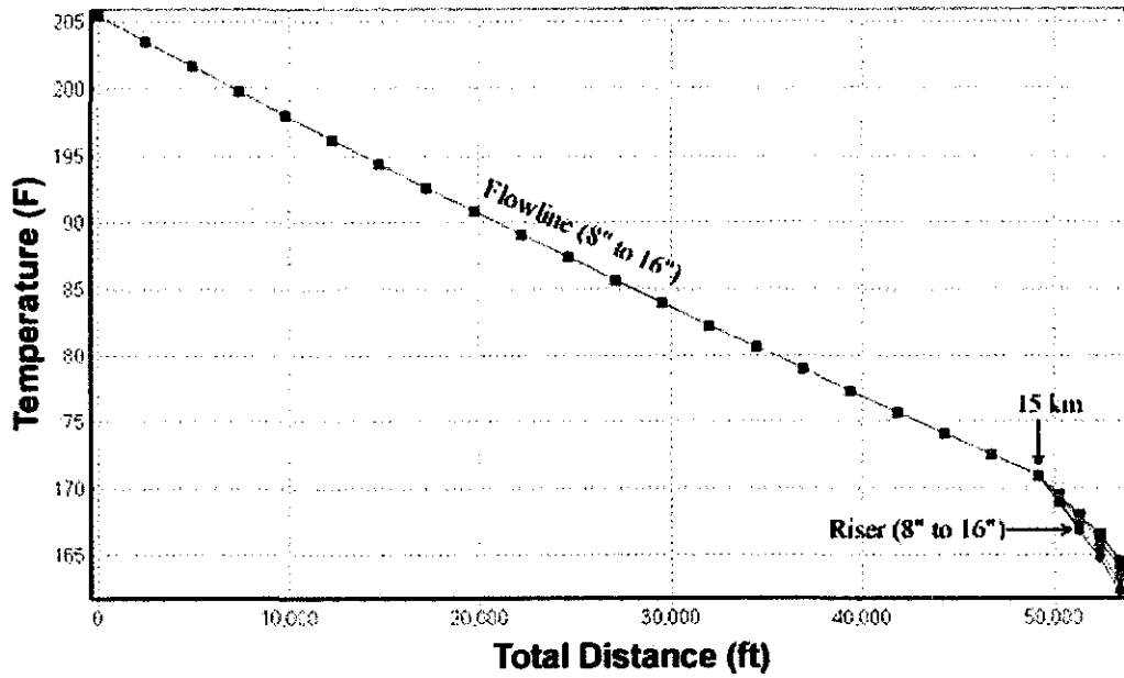
Figure 4.3a: Fluid temperature at different flowline and riser diameters
