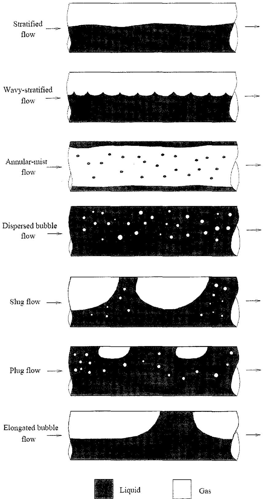
Figure 7.3: Horizontal flow patterns
