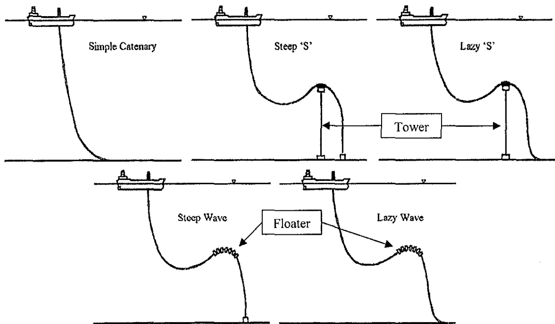
Figure 7.1: Typical flexible riser configurations
