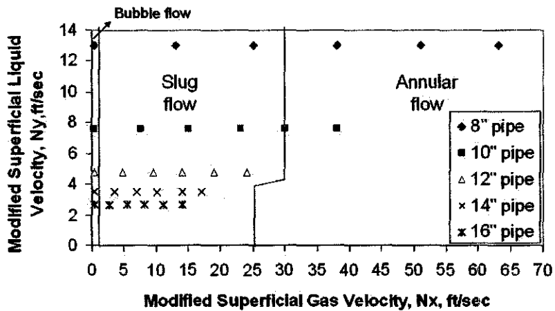
Figure 4.1j: Vertical flow for different internal pipeline diameters at 17,000 bpd
