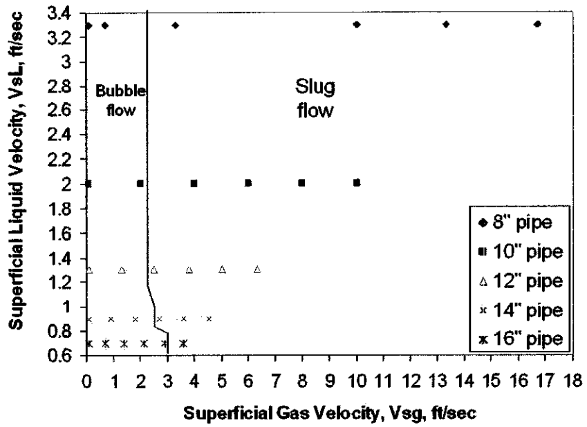
Figure 4.1d: Horizontal flow for different internal pipeline diameters at 15,000 bpd
