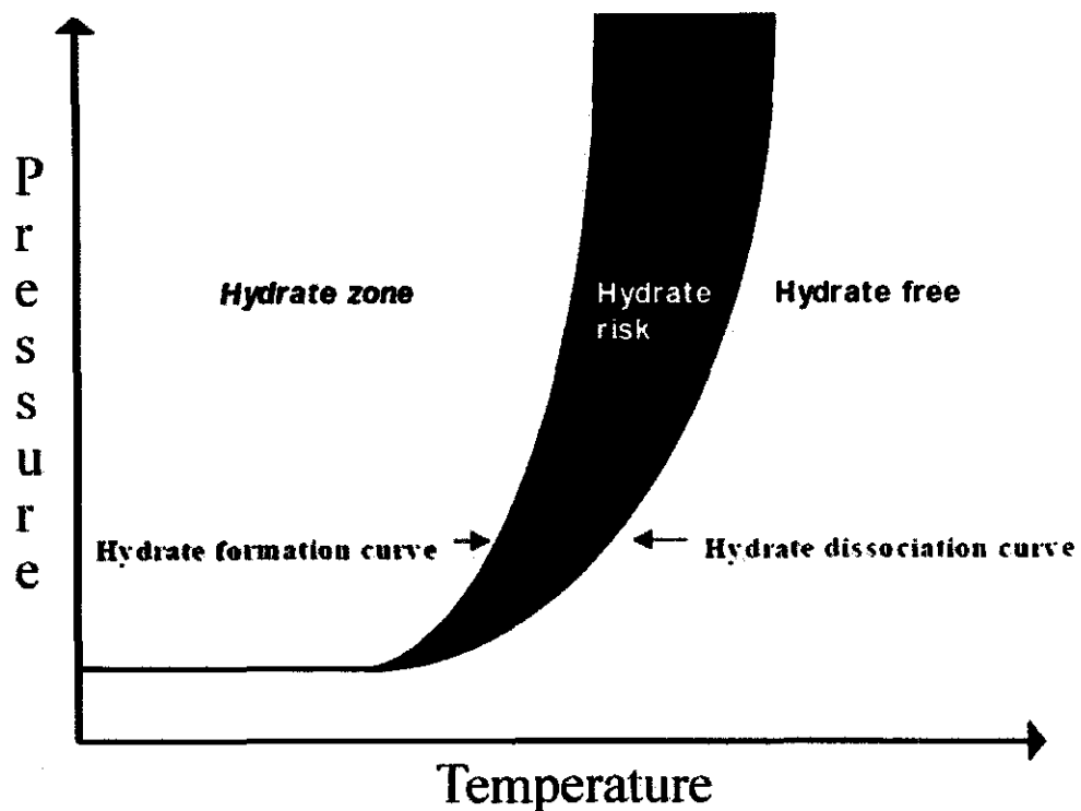
Figure 2.1: Typical hydrate formation diagram [1] .
