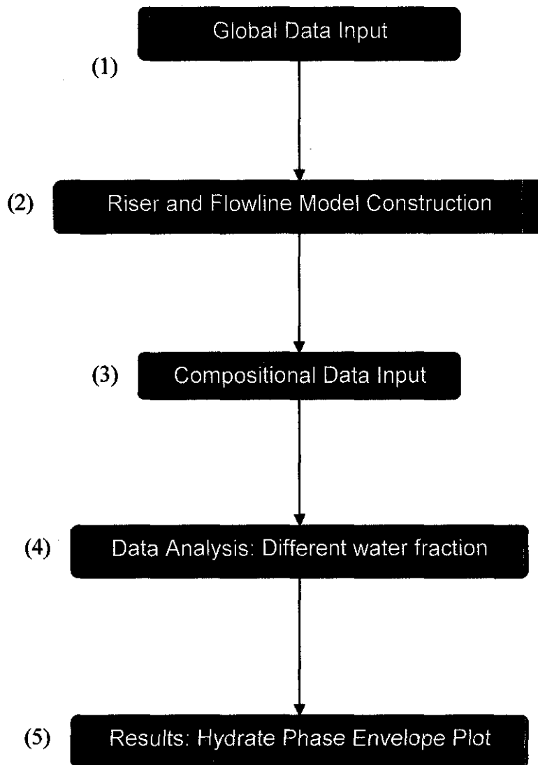
Figure 3.2: Steps of generating hydrate phase envelope using PIPESIM
