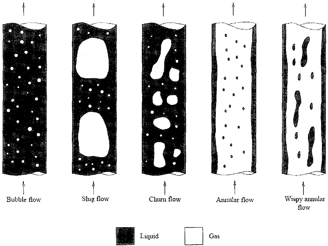
Figure 7.4: Vertical flow patterns
