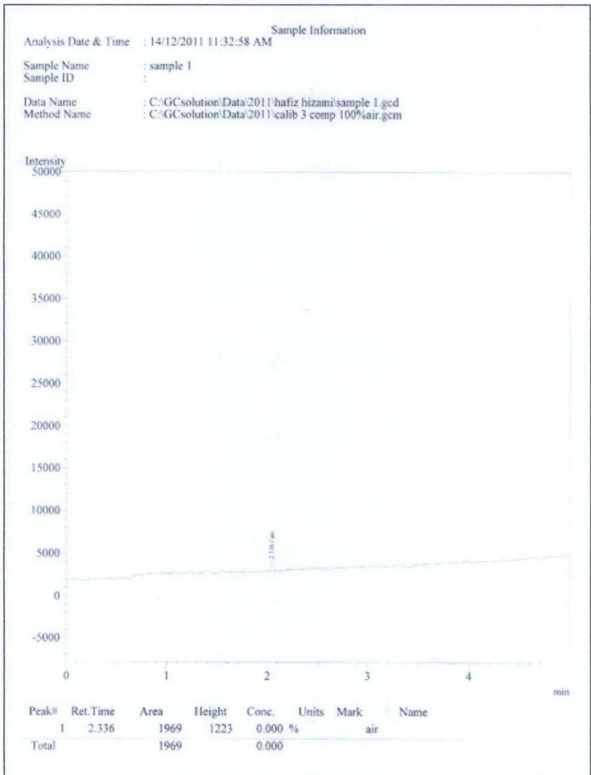
Figure 36: Second Gas Chromatography trial result
