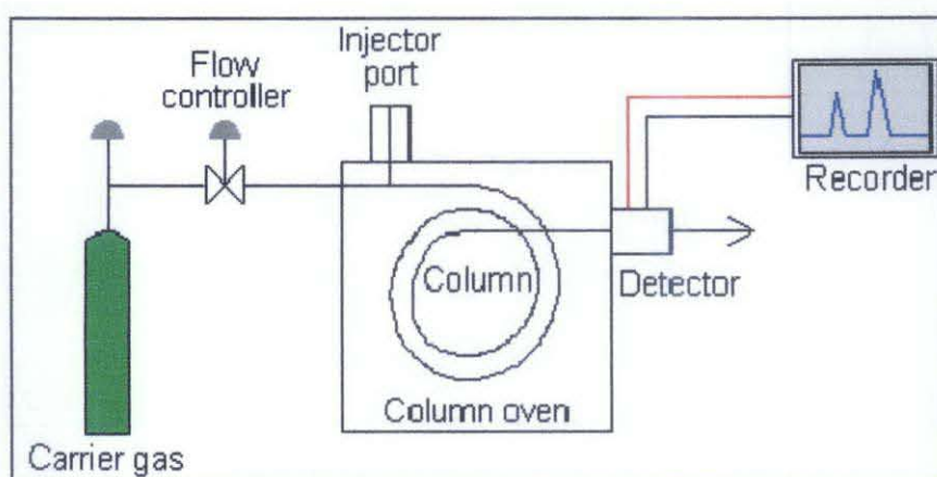
Figure 19: Diagram of gas chromatography machine
