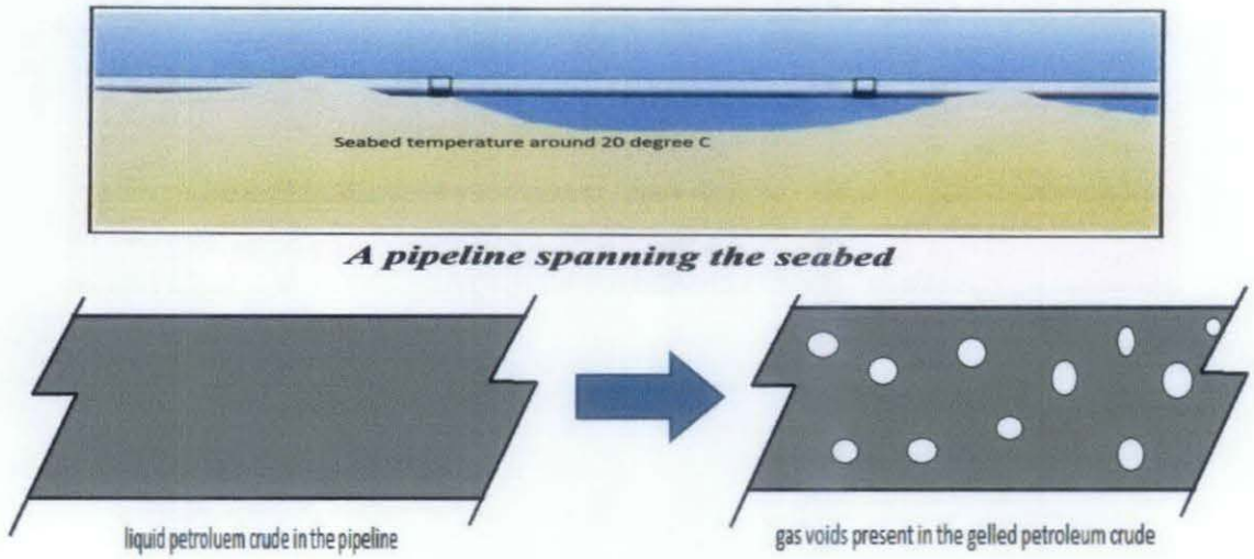
Figure 2: Gas voids formation diagram
