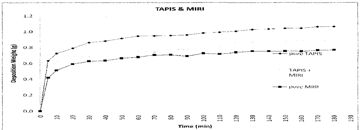
Figure 4.6: Mass of deposit (g) vs time (min) for TAPIS-MIRI blend
