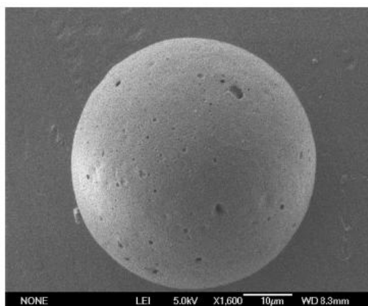
Figure 2-5 SEM micrographs of outer surface of microcapsule
