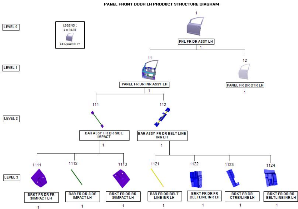
Fig. 1:Bill of material for Panel Front Door Left Hand Side Assembly
