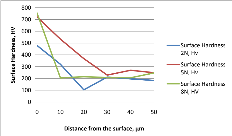
Figure 7: Depth profiles of Microhardness
