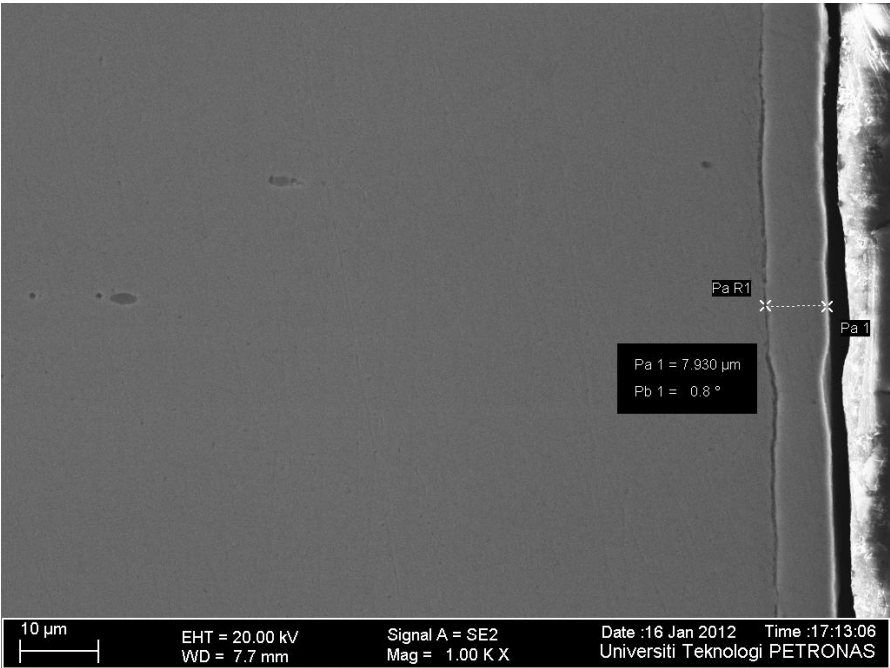
Figure 9: Nitrided layer morphology of 5N samples at 1000 X magnifications
