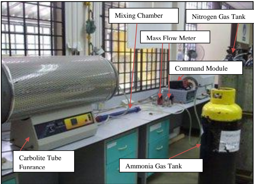
Figure 2 (b): Nitriding equipment setup at laboratory.
