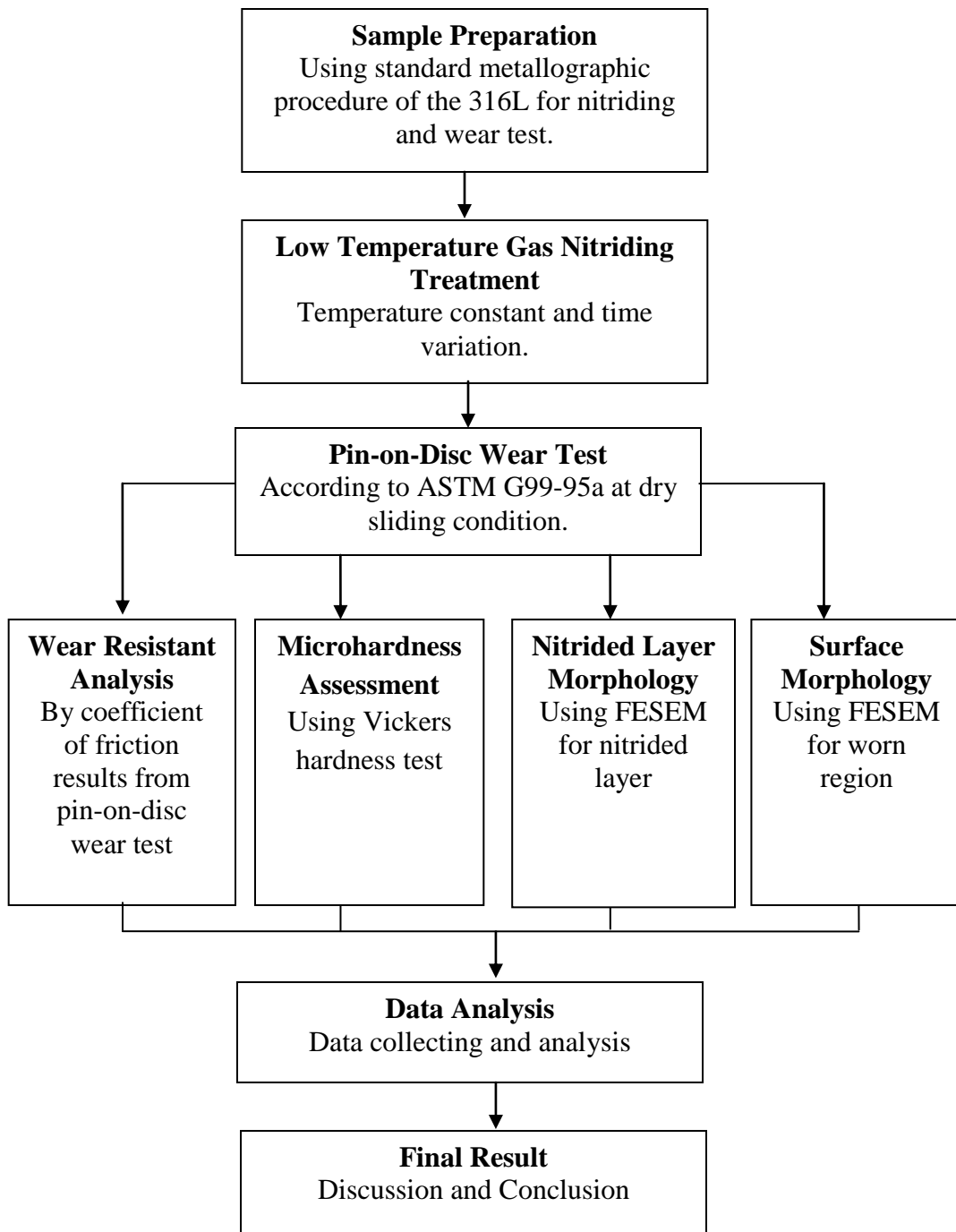
Figure 1: Flowchart of iterative process for experimental work
