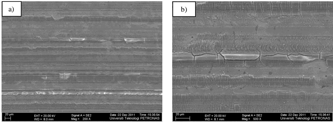
Figure 14: Surface morphology of worn region for 8N sample. (a) 200 X magnification and (b) 500 X magnification
