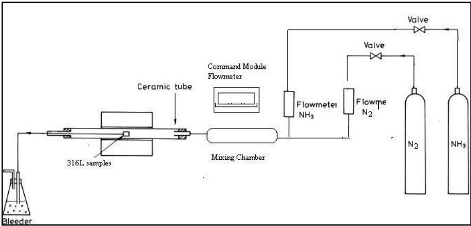
Figure 2 (a): Schematic illustration on nitriding equipment setup
