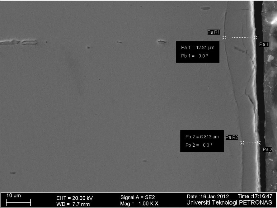
Figure 8: Nitrided layer morphology of 8N samples at 1000 X magnifications
