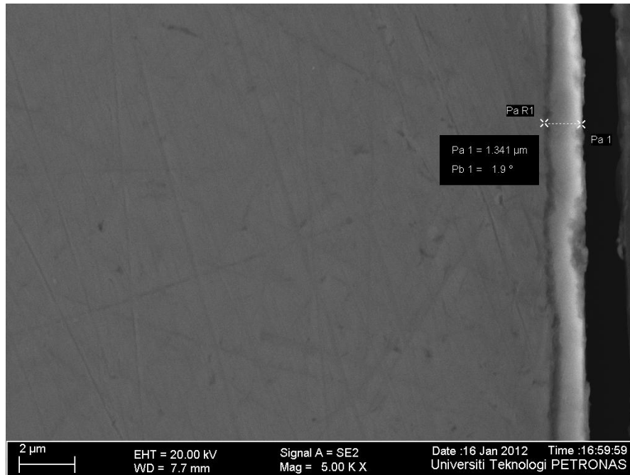
Figure 10: Nitrided layer morphology of 2N samples at 5000 X magnifications
