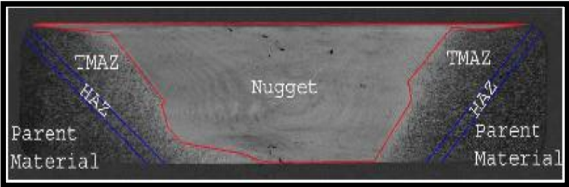
Figure 29: Expected Microstructural Region [10]
