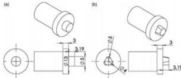
Figure 2: FSW pin profiles: (a) Straight cylindrical pin, (b) Tapered cylindrical pin. The dimensions are in mm [3]
