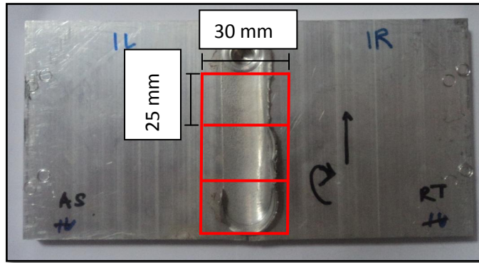
Figure 17: Portion of FSW plates cut
