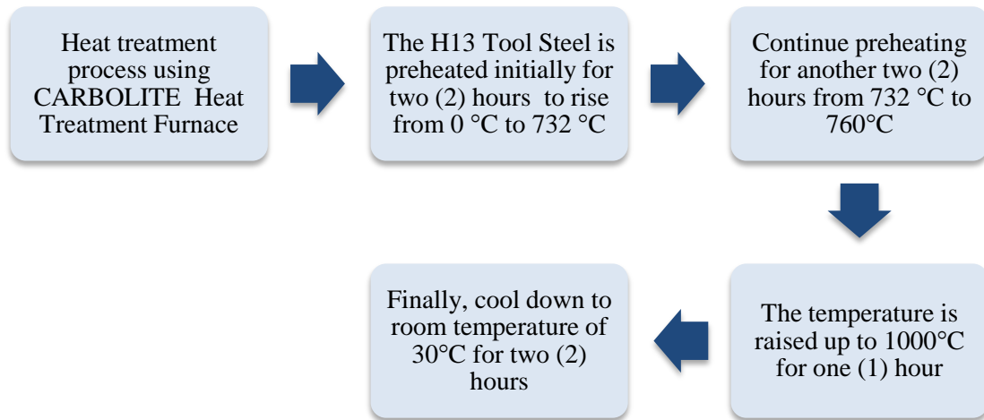
Figure 11: H13 Tool Steel Heat Treatment Process
