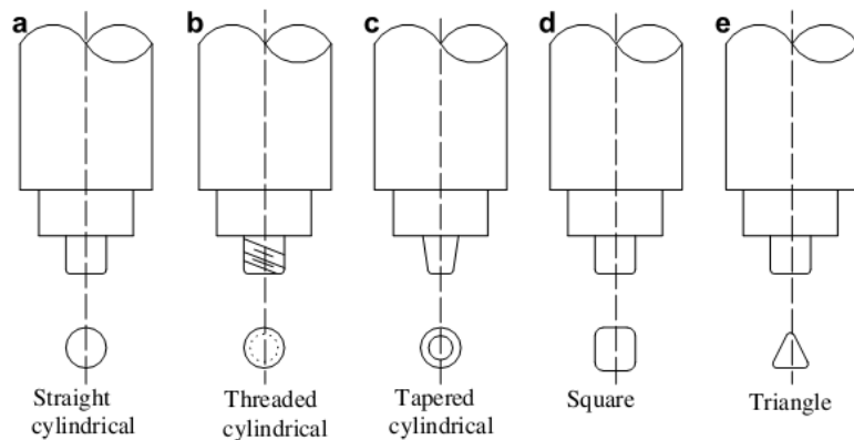
Figure 3: FSW tool pin profiles [4]
