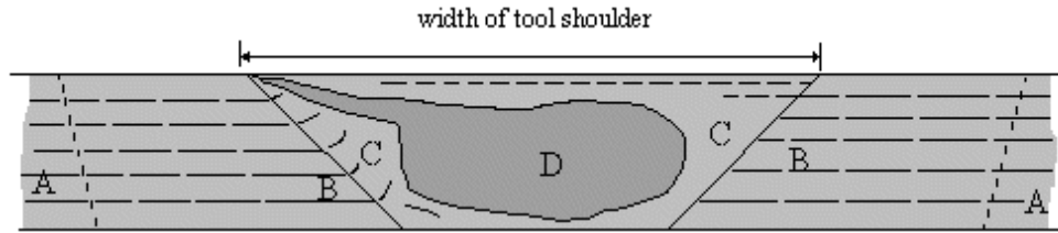
Figure 1: Microstructural regions of a friction stir welded material [2]
