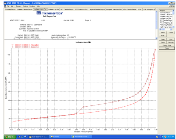
Figure A3: BET isotherm for MA 3
