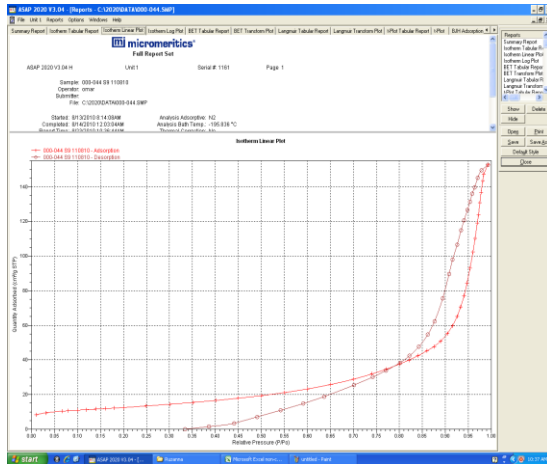
Figure A2: BET isotherm for MA 2 – 450
