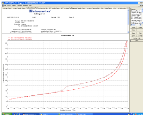
Figure A7: BET isotherm for NiMA 2:1:1
