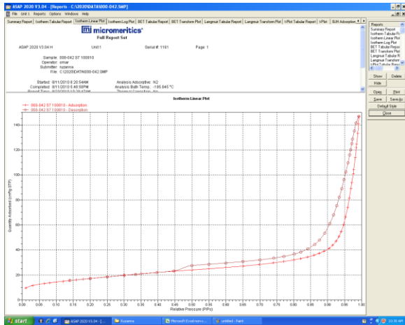
Figure A5: BET isotherm for MA 3 -60
