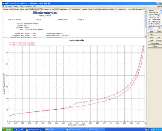
Figure A6: BET isotherm for NiMA 1:2:1
