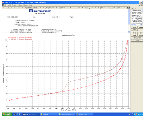
Figure A1: BET isotherm for MA 2
