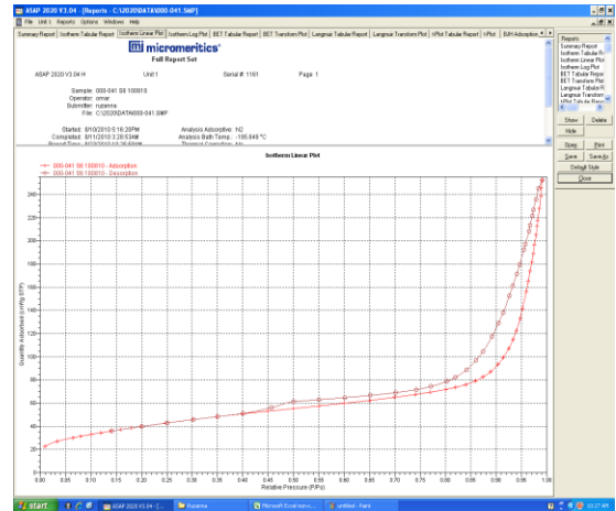
Figure A4: BET isotherm for MA 3 - 450
