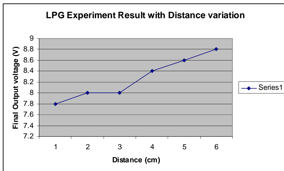
Figure 13: LPG Experiment Result with distance Variation
