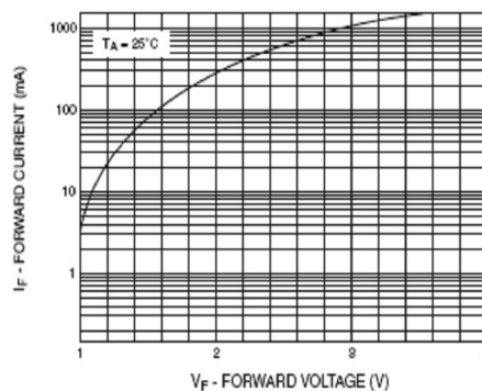
Fig. 5 Forward Current vs. Forward Voltage
