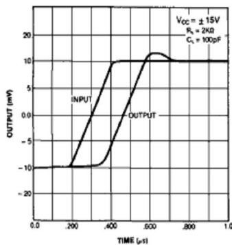
Figure 11. Transient Response
