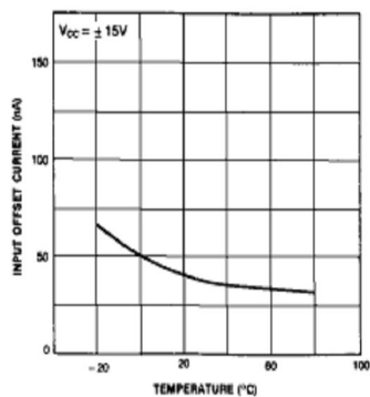
Figure 5. Input Offset Current vs Ambient Temperature
