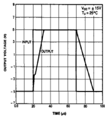
Figure 1. Voltage Follower Large Signal Pulse Response
