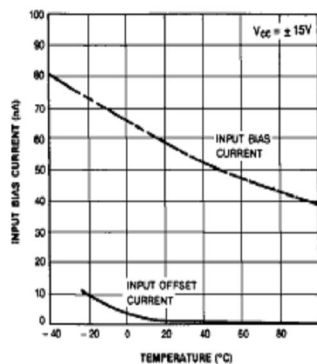
Figure 3. Input Bias Current vs Ambient Temperature
