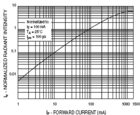
Fig. 1 Normalized Radiant Intensity vs. Forward Current
