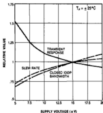
Figure 9. Frequency Characteristics vs Supply Voltage
