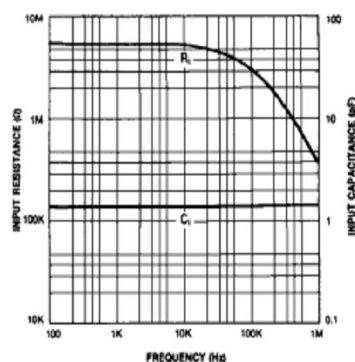
Figure 2. Input Resistance and Input Capacitance vs Frequency
