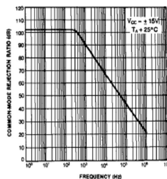
Figure 12. Common-Mode Rejection Ratio vs Frequency
