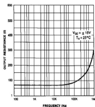
Figure 1. Output Resistance vs Frequency
