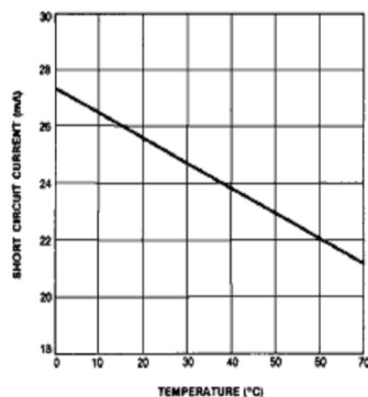
Figure 10. Output Short Circuit Current vs Ambient Temperature
