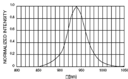
Fig. 3 Normalized Radiant Intensity vs. Wavelength
