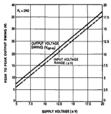
Figure 2. Output Swing and Input Range vs Supply Voltage
