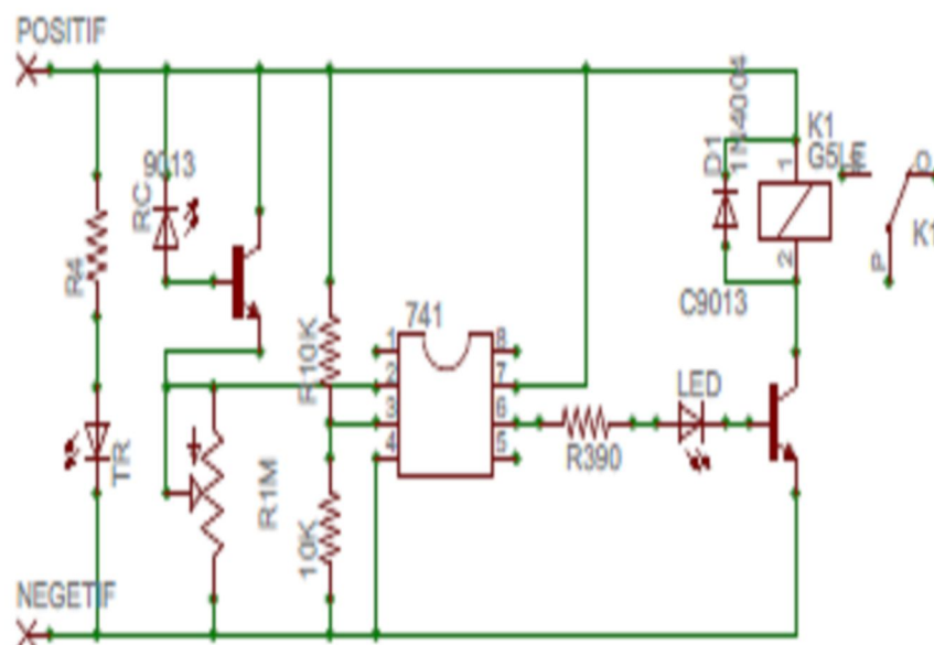
Figure 9: Infrared circuit (small view)
