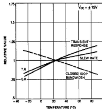
Figure 8. Frequency Characteristics vs Ambient Temperature
