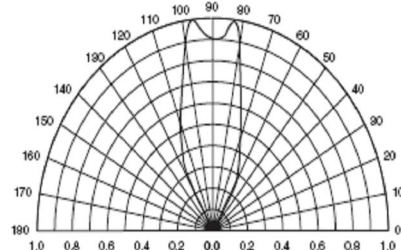
Fig. 4 Radiation Diagram
