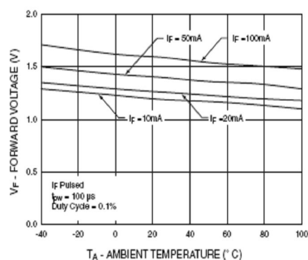
Fig. 2 Forward Voltage Vs. Ambient Temperature
