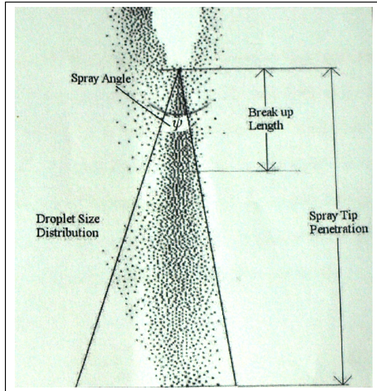
Figure 2.2 : Determination of Spray Cone Angle
