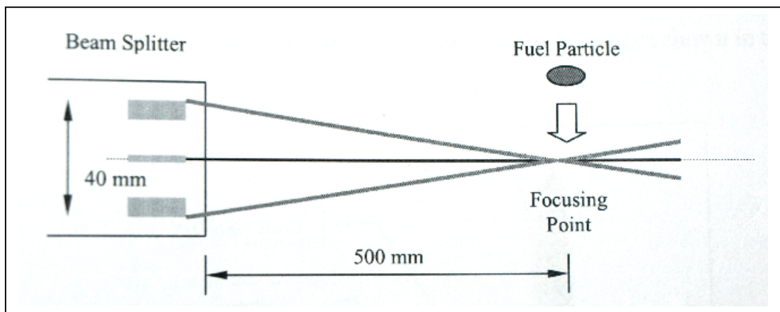
Figure 3.3 : Beam focusing point
