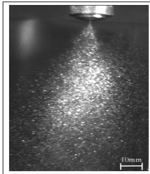
Figure 2.9 : Air atomizer at an air flow rate of 0.111/s
