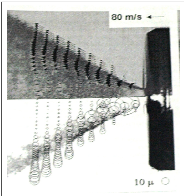
Figure 2.16: Spray Cone Collapse
