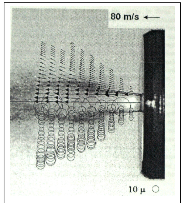
Figure 2.12: Pre-Swirl Spray
