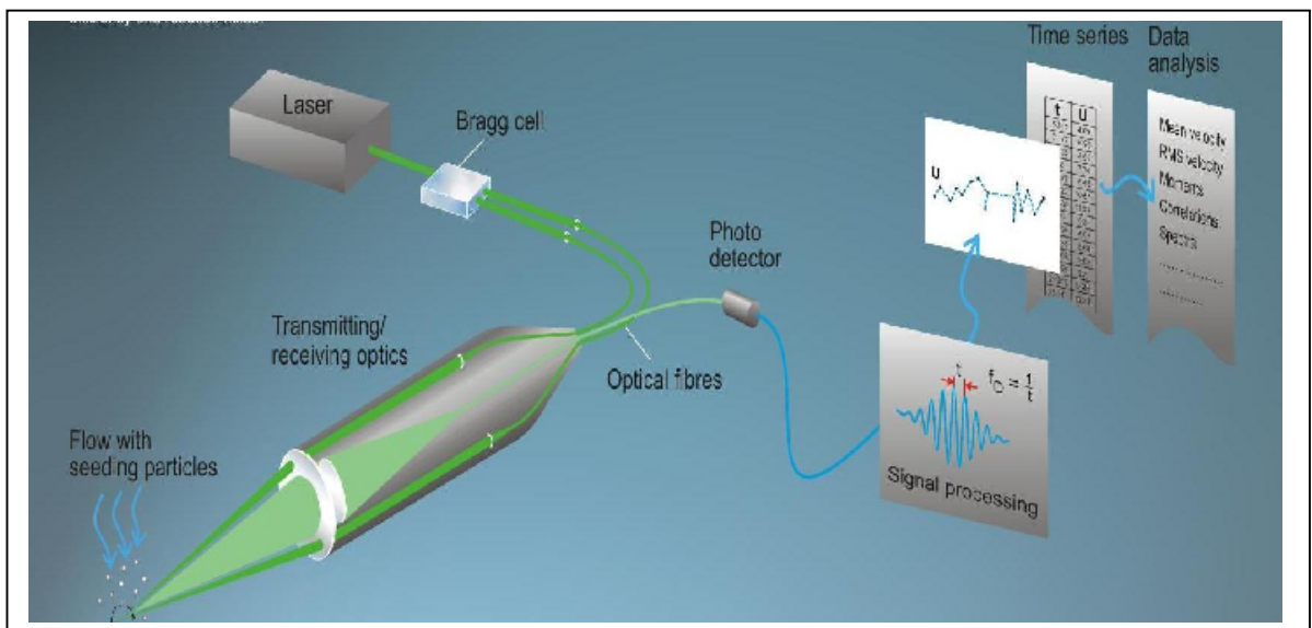
Figure 3.1 : Laser Doppler Velocimetry
