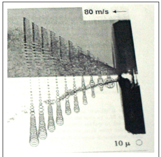
Figure 2.17: Spray Detaches from the Nozzle
