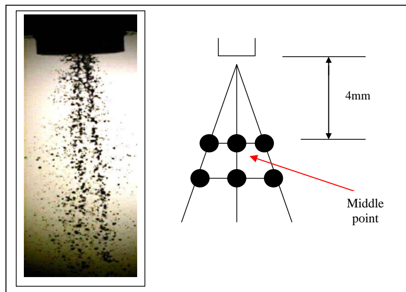
Figure 4.4 : Middle Point of Gasoline Spray
