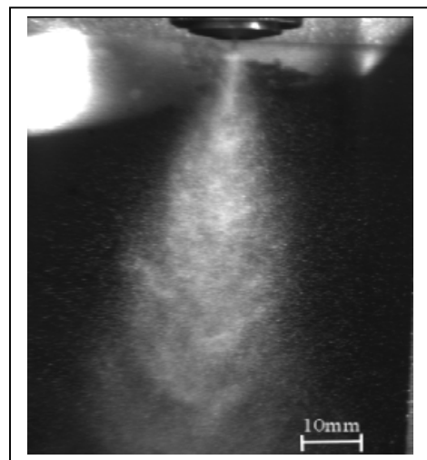
Figure 2.10 : Air atomizer at an air flow rate of 0.181/s
