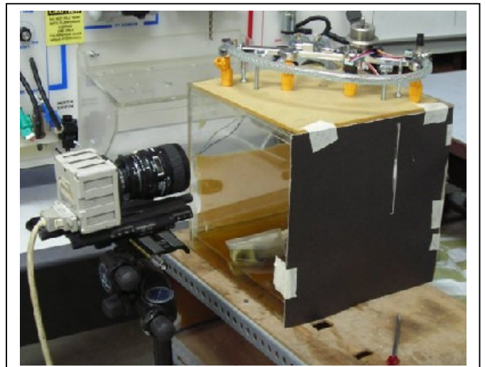
Test Chamber and High Speed Camera
