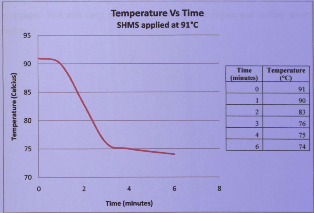
Figure 4.5 : Engine temperature when SHMS applie at 91°C
