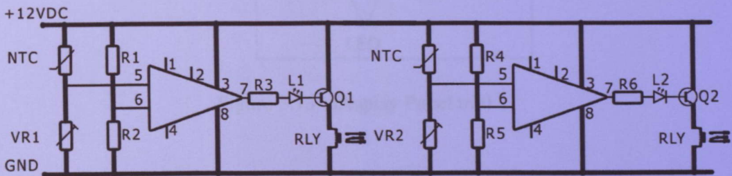
Figure 3.12 : Control Unit Trial 1
