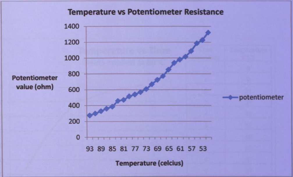
Figure 4.2 : Potentiometer vs Temperature
