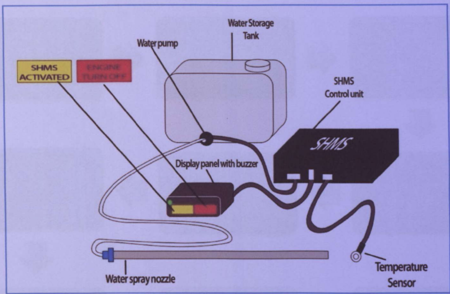
Figure 3.4: Drawing of Planned SHMS
