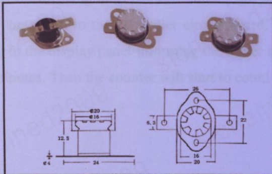
Figure 3.1: Thermostat switches
