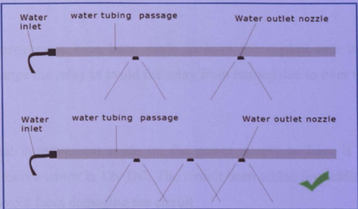
Figure 3.11 : Water Spray Trial 2
