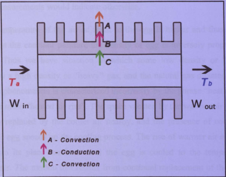
Figure 2.3: Heat Transfer Analogy ( Yunus A Cengel, 2006 )
