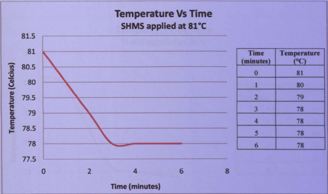
Figure 4.4 : Engine temperature when SHMS applie at 81°C
