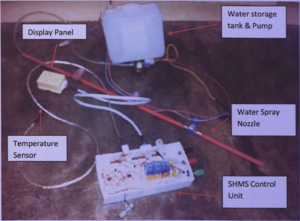
Figure 4.1 : The Complete SHMS Unit
