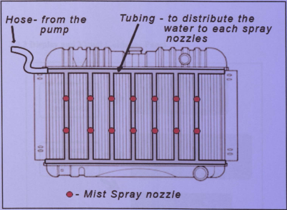
Figure 3.2: Spray Nozzles Arrangement.
