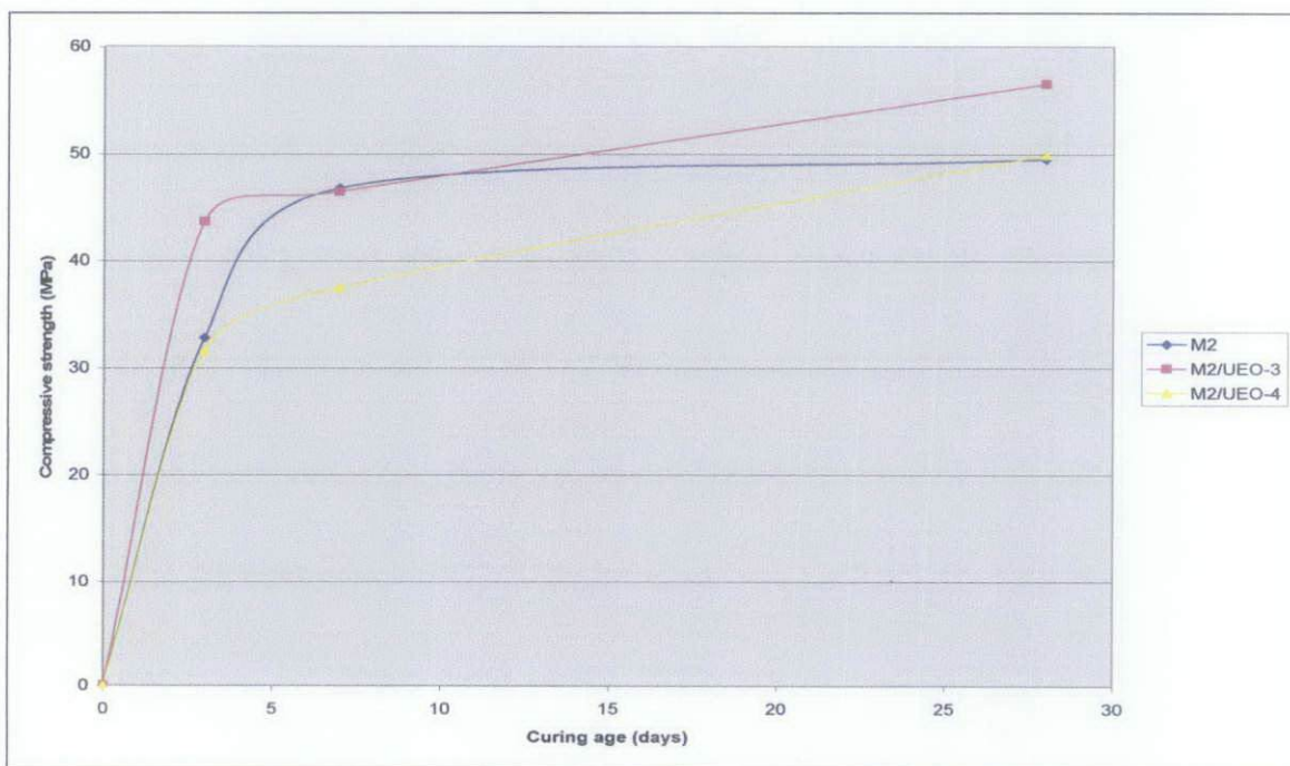
Figure 4.3: Compressive strength for 0.37% of w/b mix
