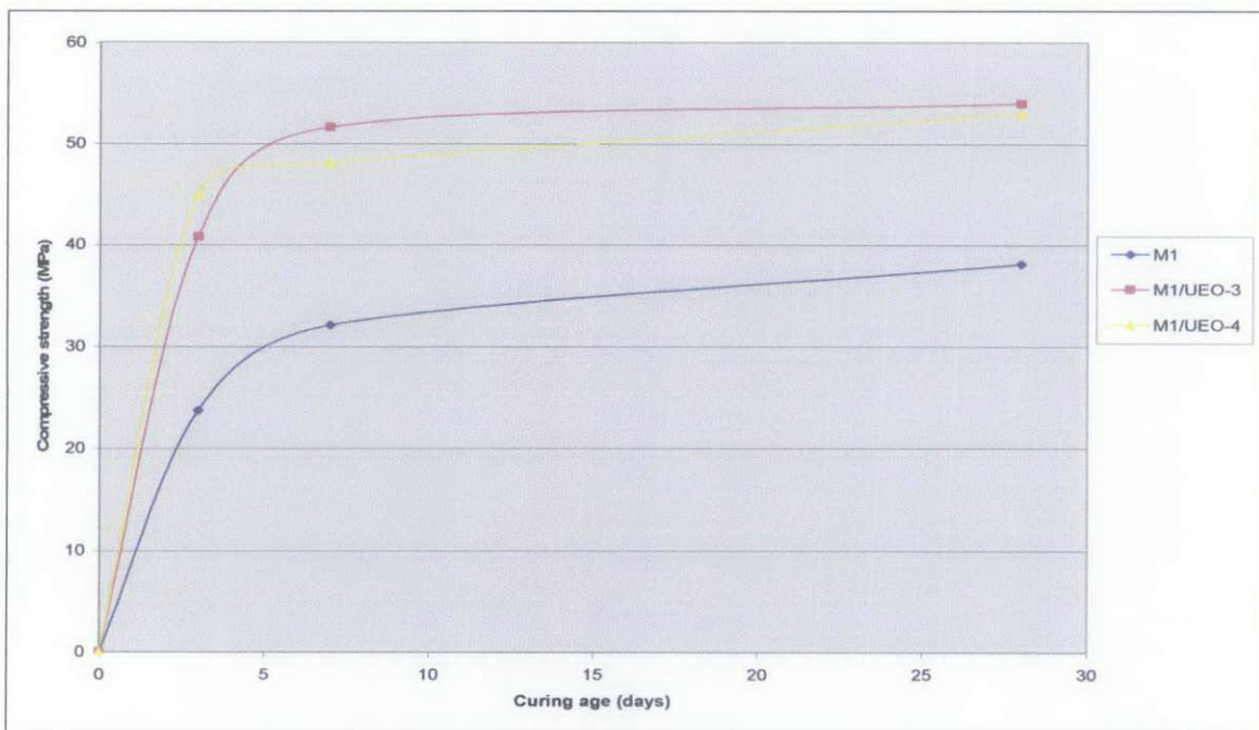
Figure 4.2: Compressive strength for 0.4 % of w/b mix
