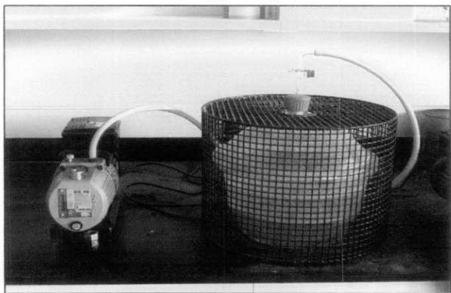
Figure 3.5: Vacuum saturation apparatus
