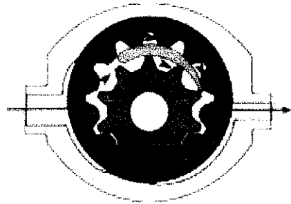
Gearpump with internal teeth
