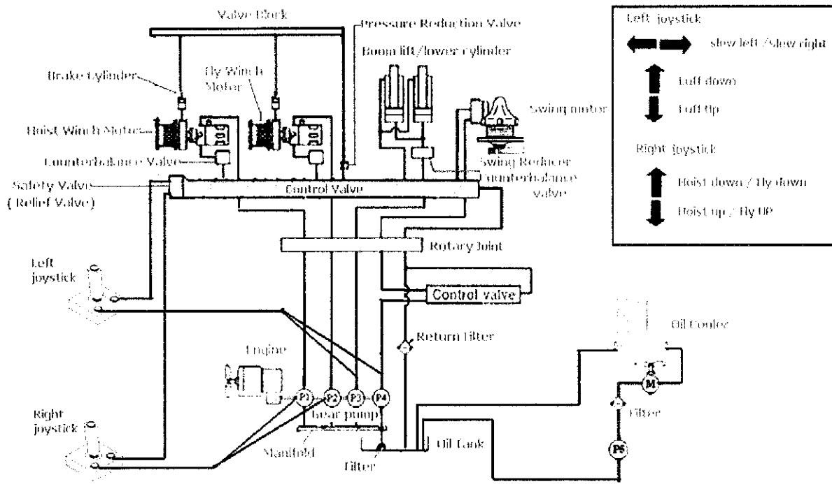
Figure 12: Hydraulic circuit for Ram Luffing Crane
