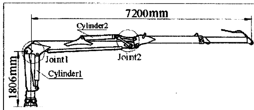
Figure 17: example of hydraulic crane [3]
