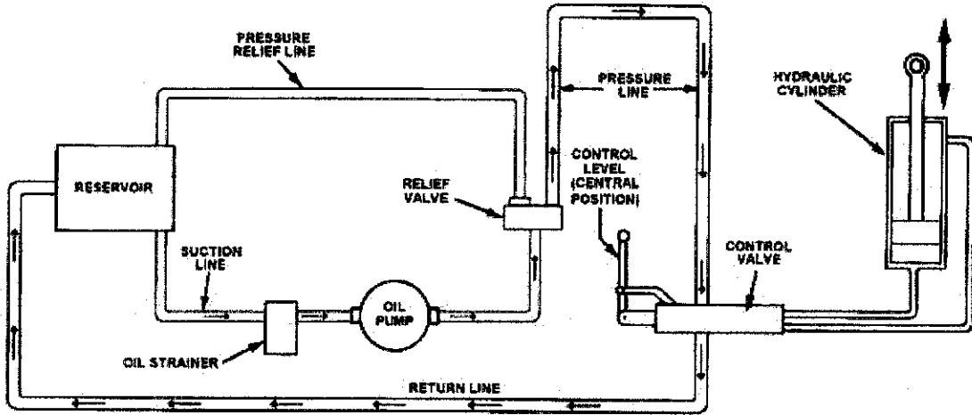
Figure 4: Reservoir piping
