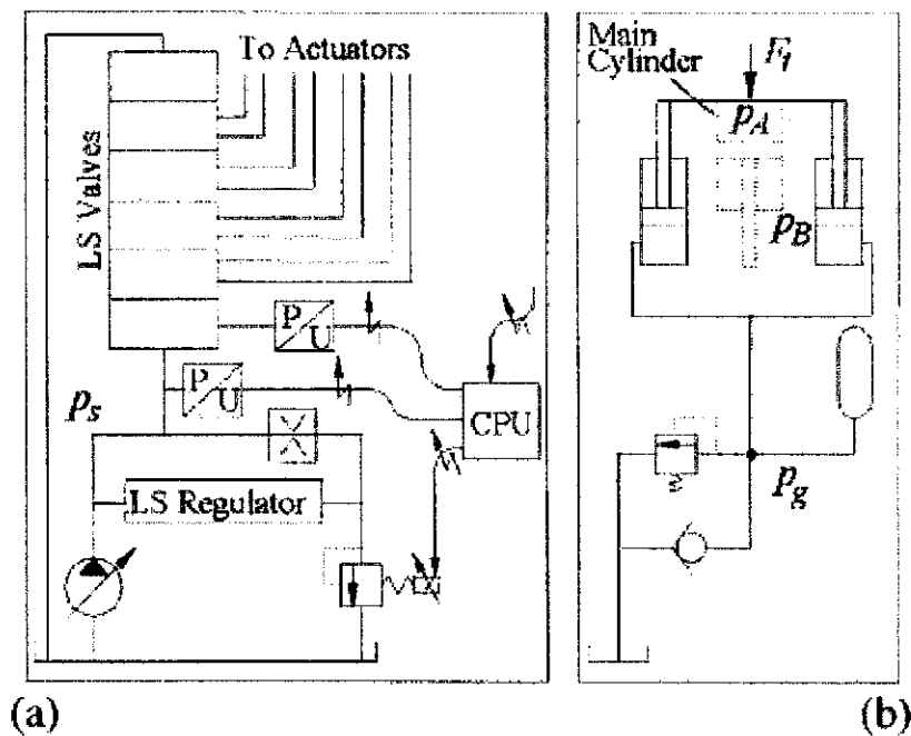
Figure 16: Main system and assistant system [3]
