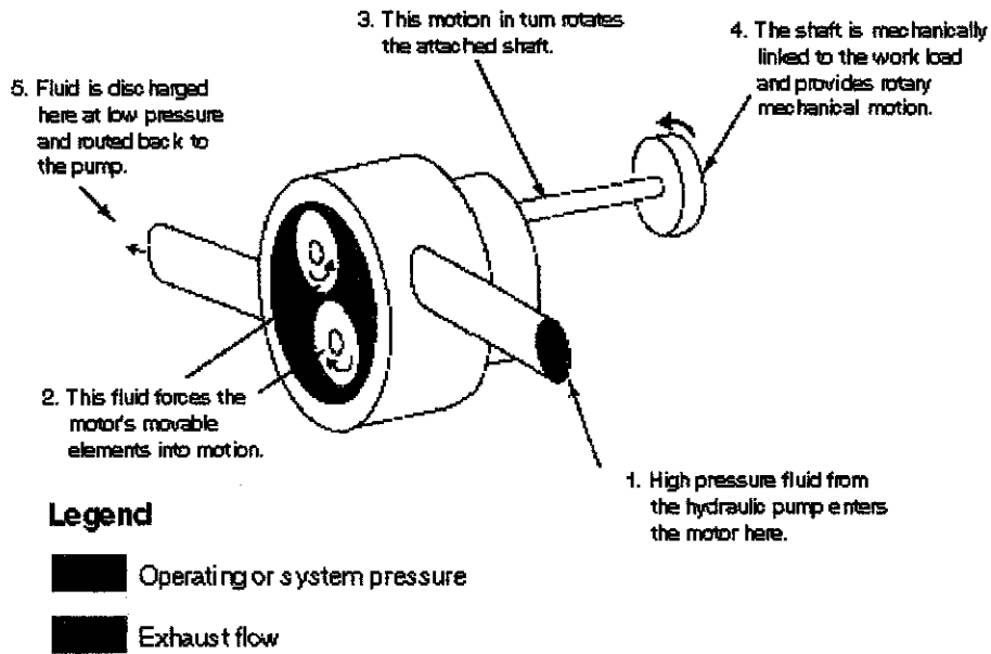
Figure 6: Basic Operation of Hydraulic Motor
