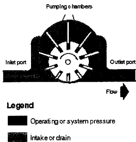
Figure 8: Positive displacement pump
