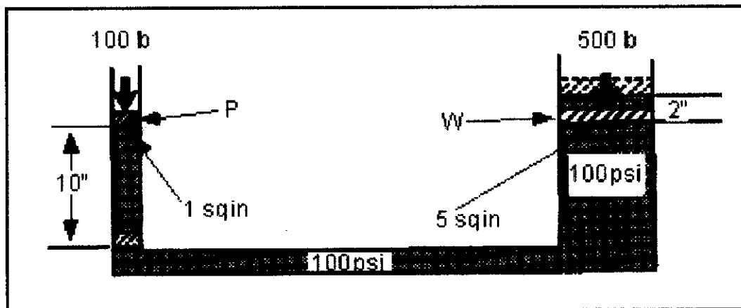
Figure 3: Pascal Law
