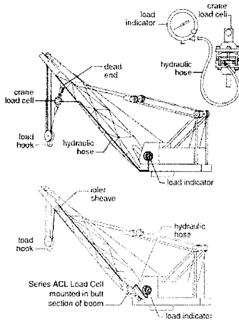
Figure 2: Crane load diagram [2]
