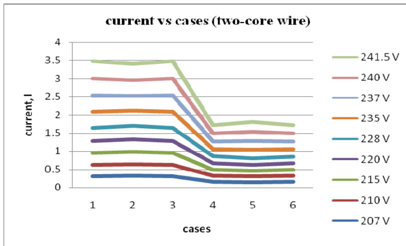
Figure 28 Current graph using two-core wire
