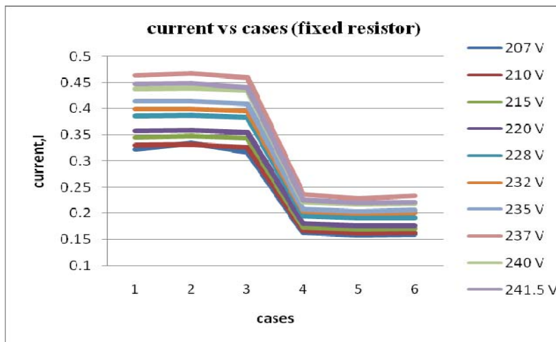
Figure 26 Current graph using fixed resistor
