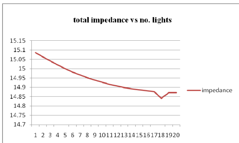
Figure 15 Graph for total impedance versus number of lights
