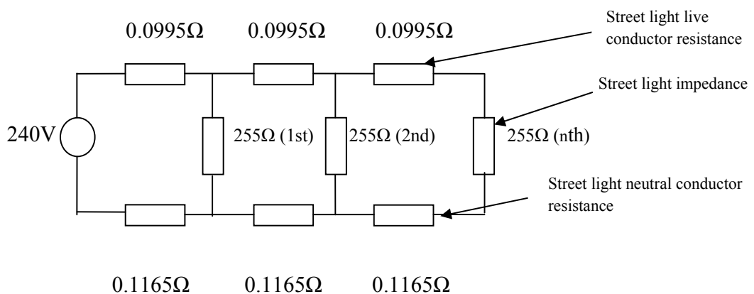
Figure 6 Circuit diagram for manual calculation
