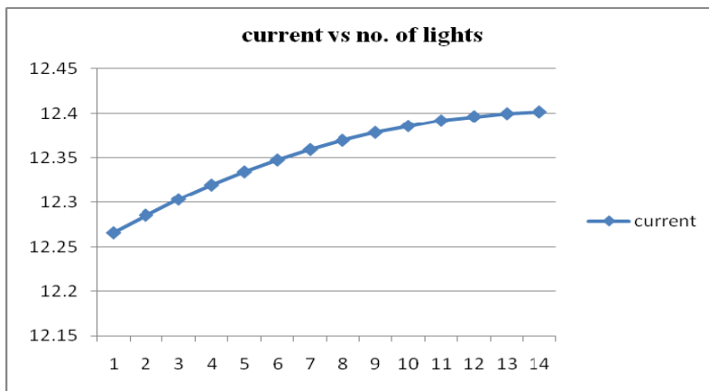
Figure 18 Graph for current versus number of lights
