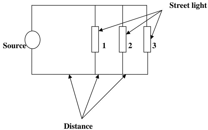
Figure 5 Circuit diagram for Impedance Base Algorithm
