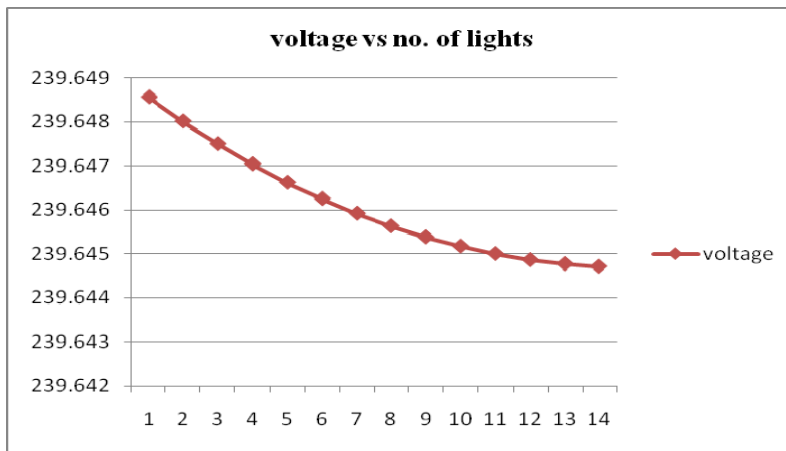
Figure 17 Graph for voltage versus number of lights
