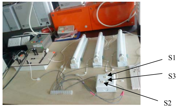
Figure 8 Street Lighting Conductor Prototype
