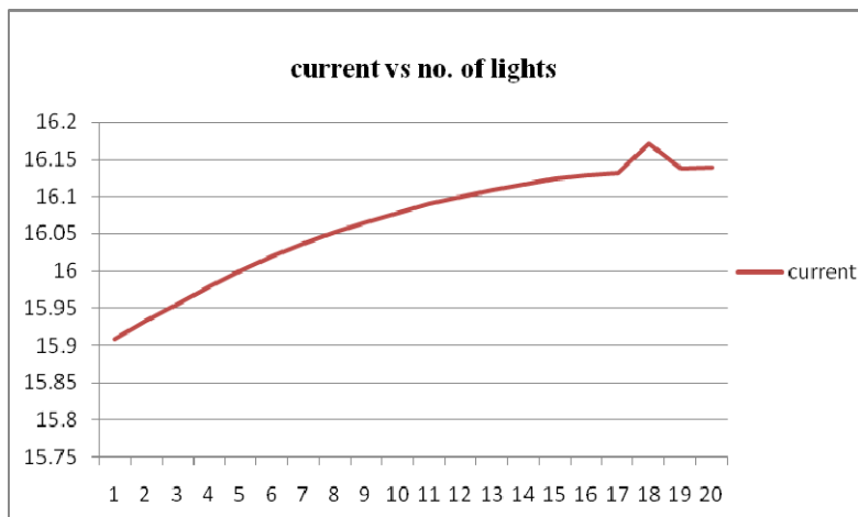
Figure 14 Graph for current versus number of lights
