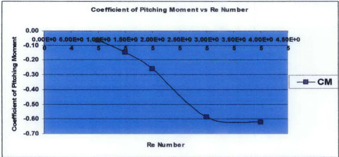
Figure 4.11: Graph of Re Number against Coefficient of Pitching Moment
