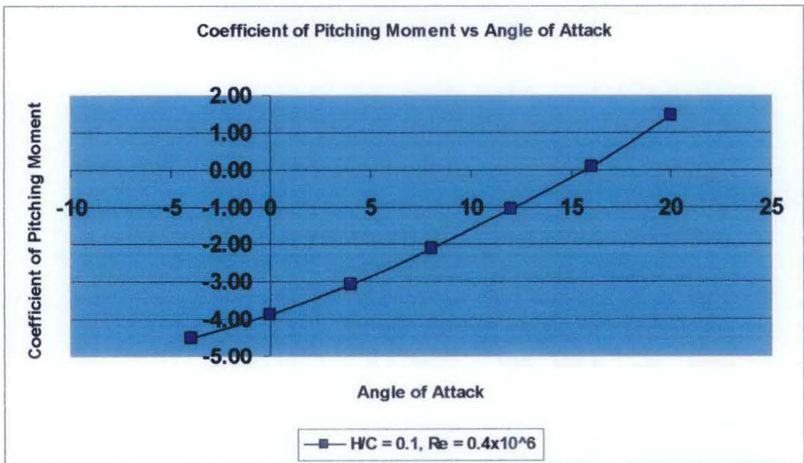
Figure 4.25: CM vs AOA at H/C = 0.1, Re = 0.4 \times 10^6
