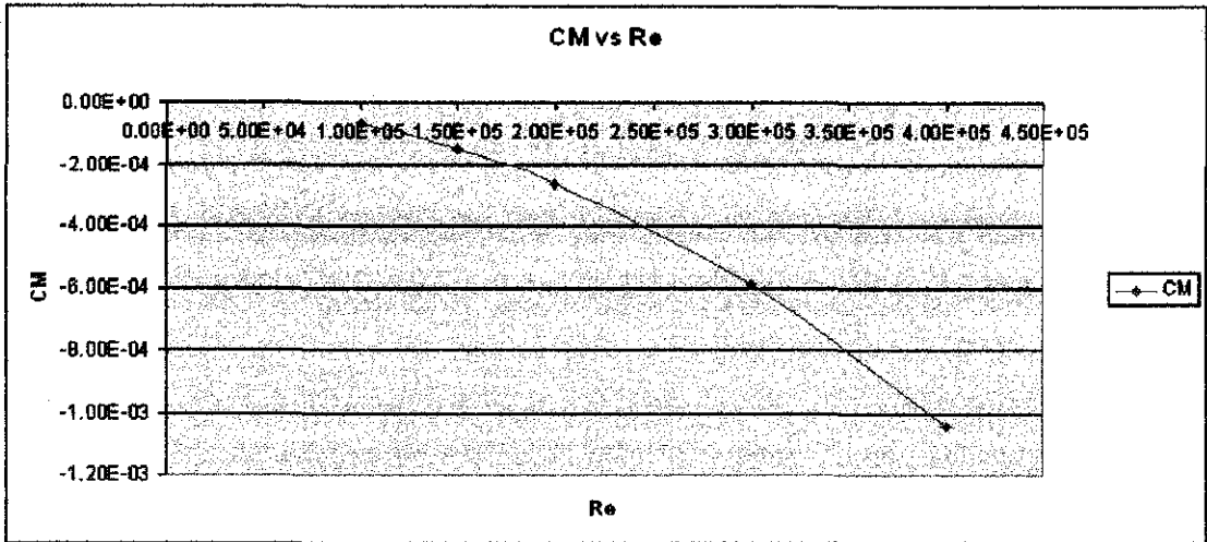
Figure 4.28: CM vs Re at AOA = 4, H/C = 0.1
