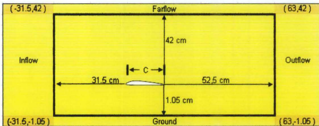
Figure 4.16: Boundary Model for H/C= 0.1 and angle of attack \alpha = 0^\circ
