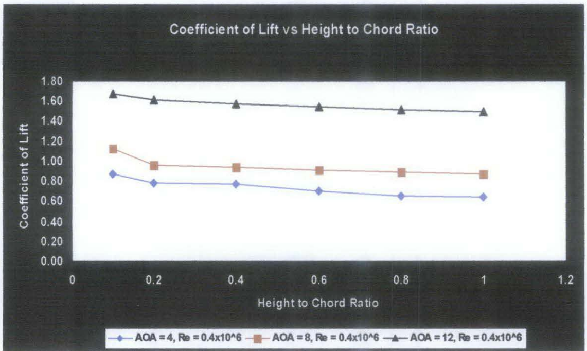
Figure 4.29: CL vs H/C Ratio at different Re and AOA
