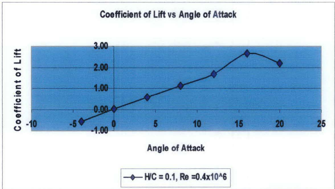
Figure 4.23: CL vs AOA at H/C = 0.1 , Re = 0.4 \times 10^6
