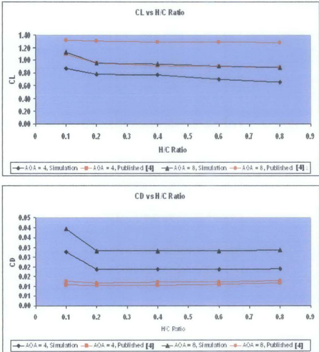
Figure 4.33: Comparison of Simulation work with previous work
