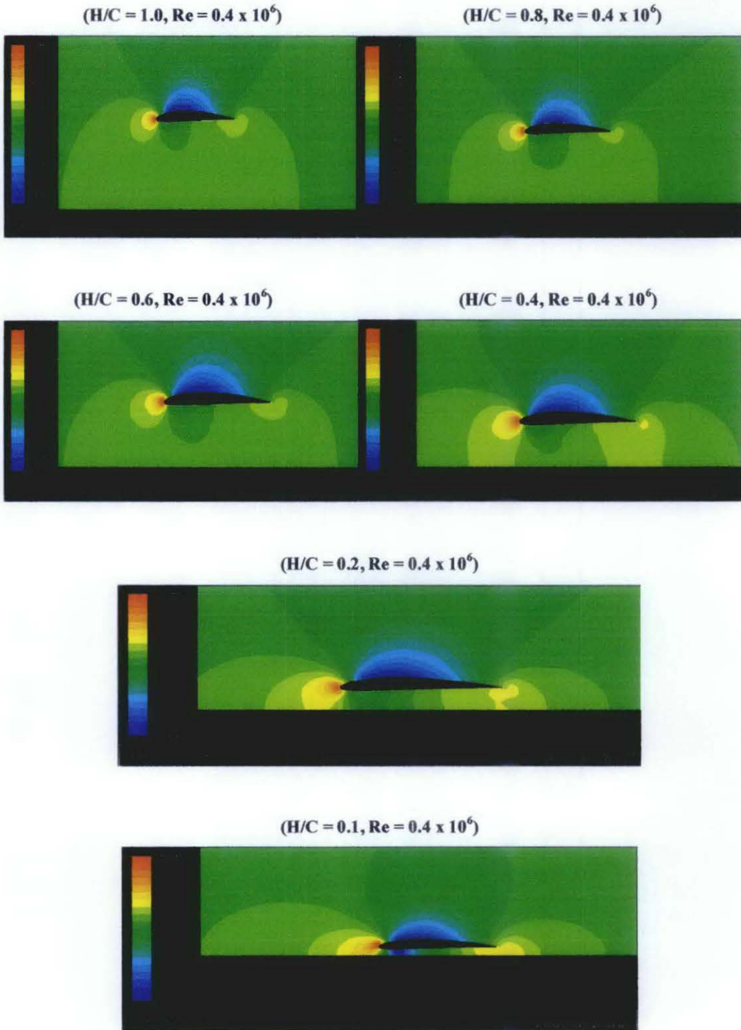
Figure 4.20: Contour of static pressure around the Airfoil
