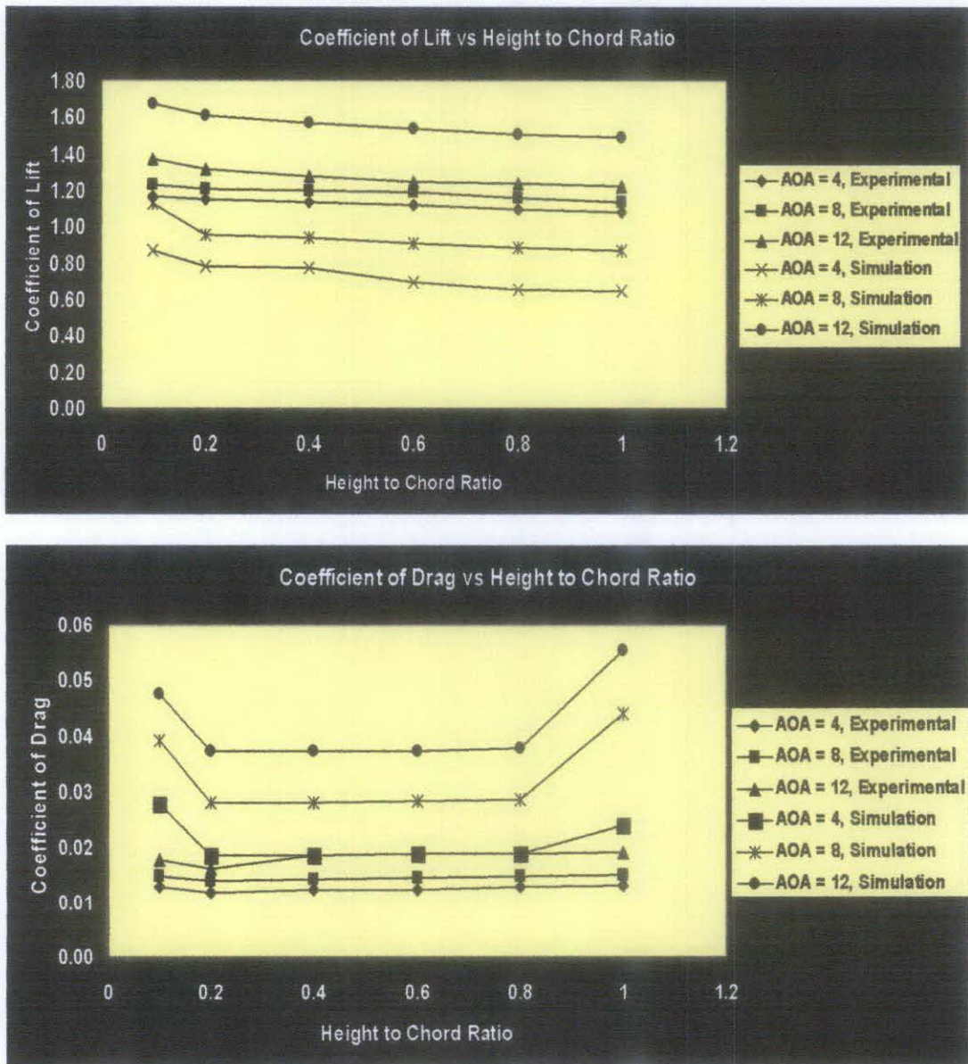
Figure 4.31: Comparison Graph of H/C Ratio against CL and CD
