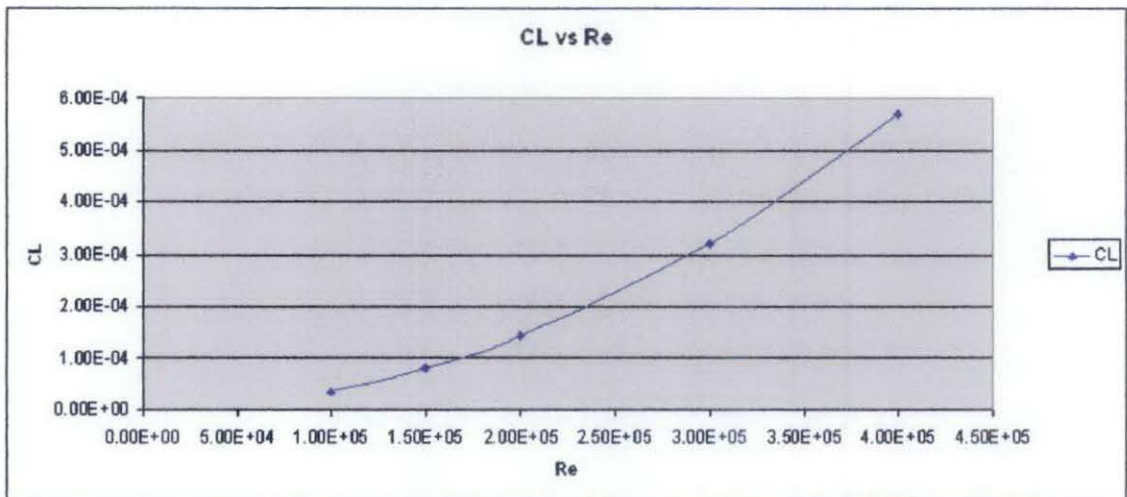
Figure 4.26: CL vs Re at AOA = 4, H/C = 0.1
