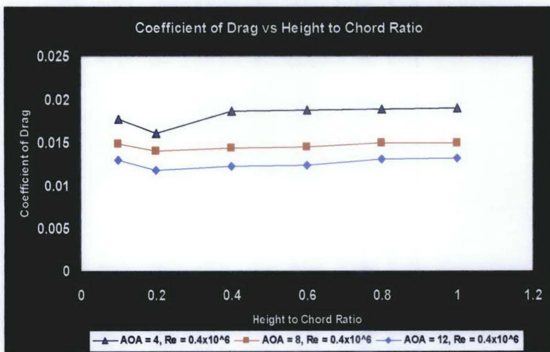
Figure 4.12: Graph of H/C Ratio against Coefficient of Lift and Drag
