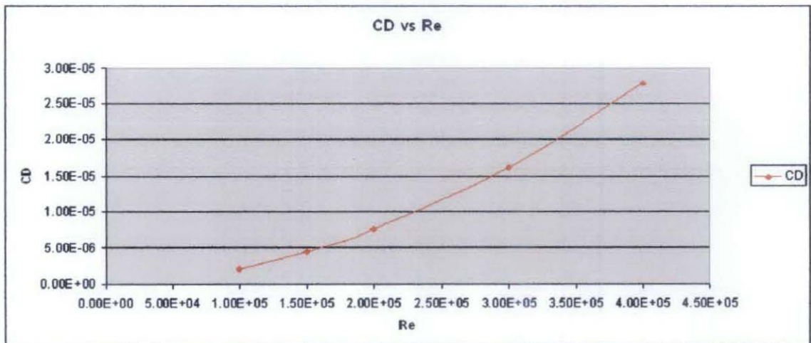
Figure 4.27: CD vs Re at AOA = 4, H/C = 0.1
