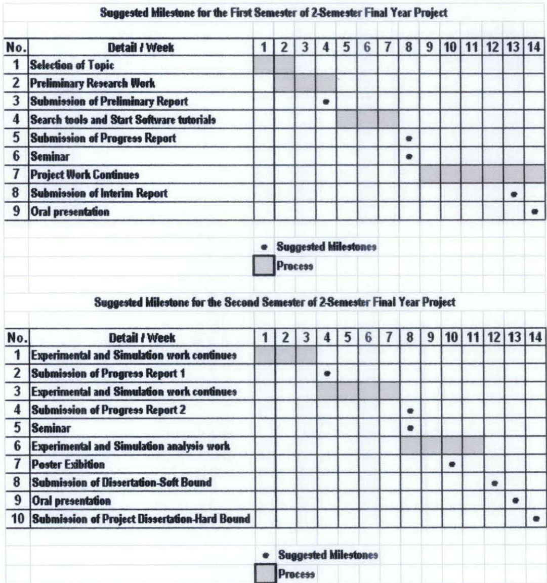
Figure 3.2: Gantt chart
