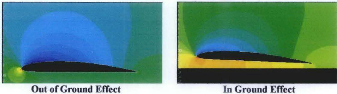
Figure 2.6: CFD Results [8]
