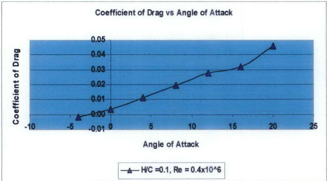
Figure 4.24: CD vs AOA at H/C = 0.1, Re = 0.4 \times 10^6
