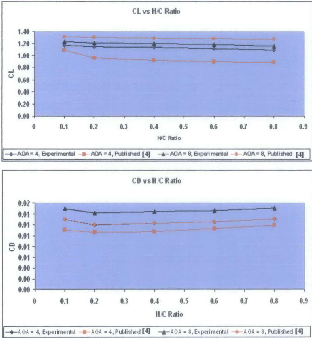
Figure 4.32: Comparison of Experimental work with previous work
