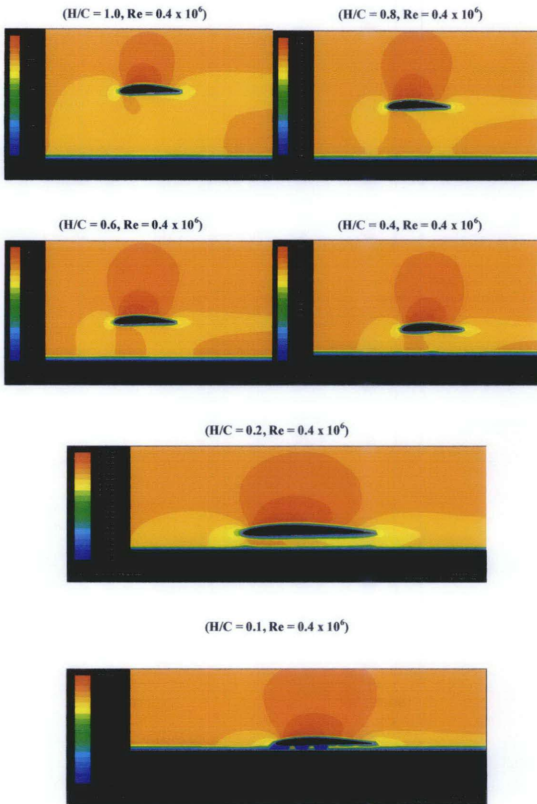
Figure 4.22: Contour of velocity magnitude around the Airfoil
