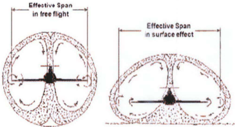
Figure 2.4: Effective Span [8]
