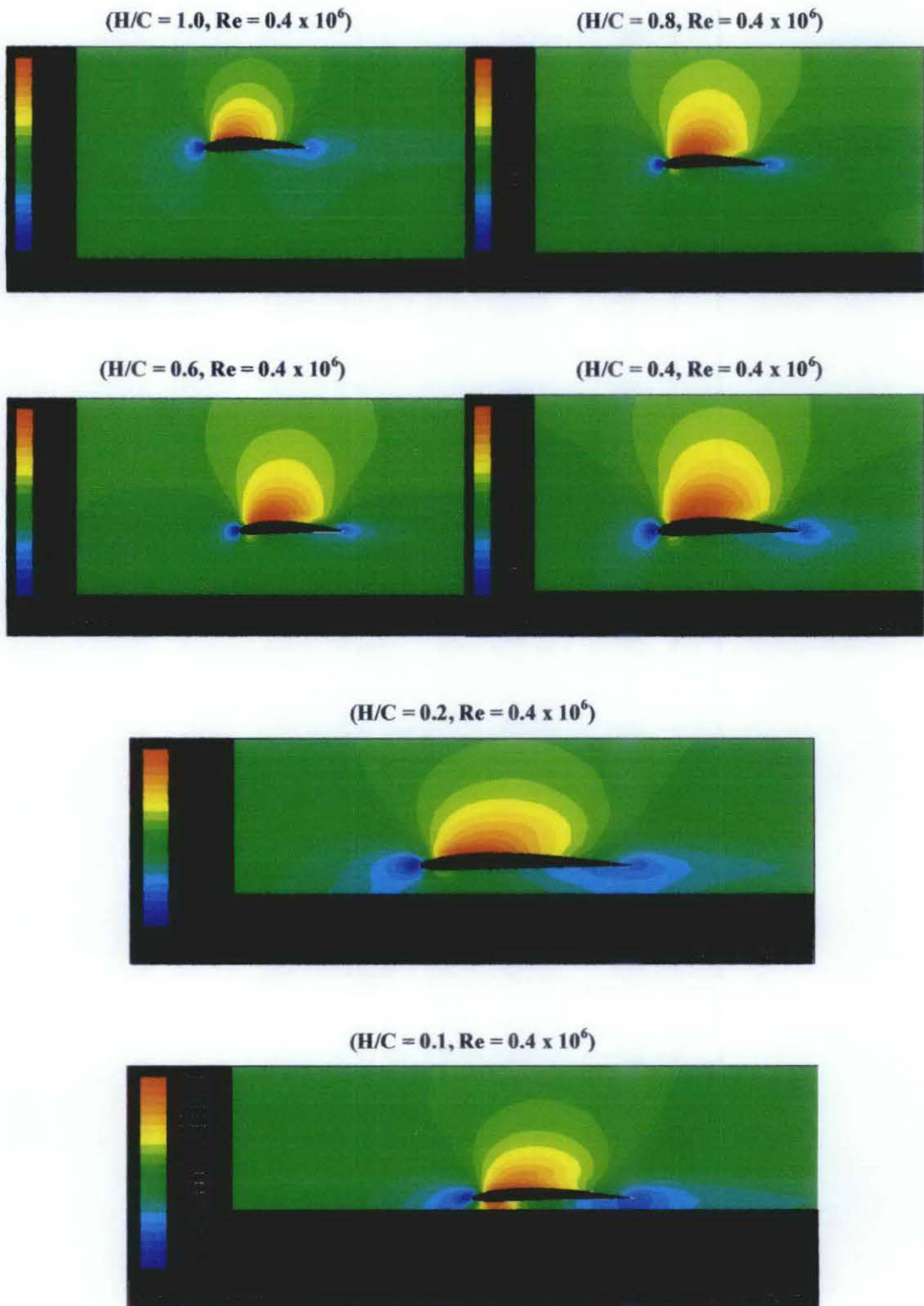
Figure 4.21: Contour of dynamic pressure around the Airfoil
