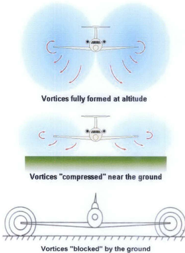
Figure 1.1: Phenomena of ground effect [7]
