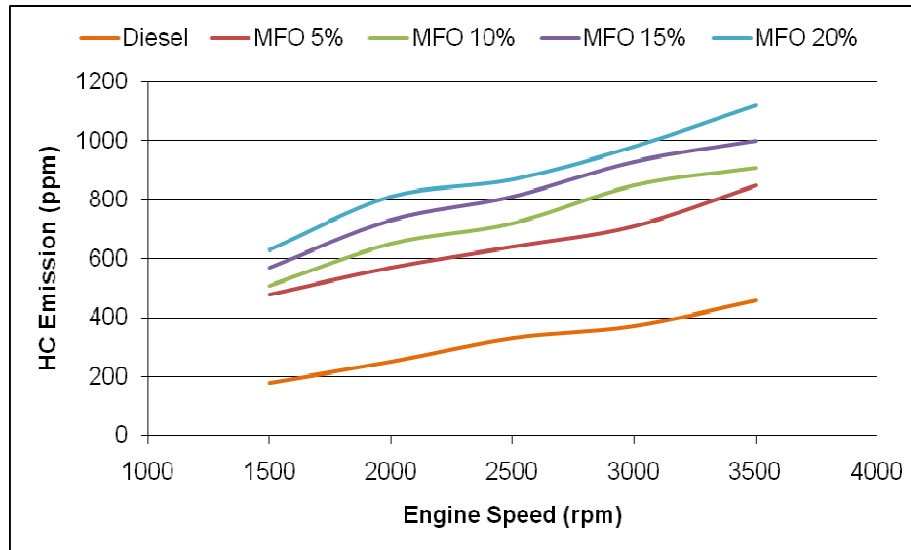
Figure 4.9: Unburned HC emission versus engine speed
