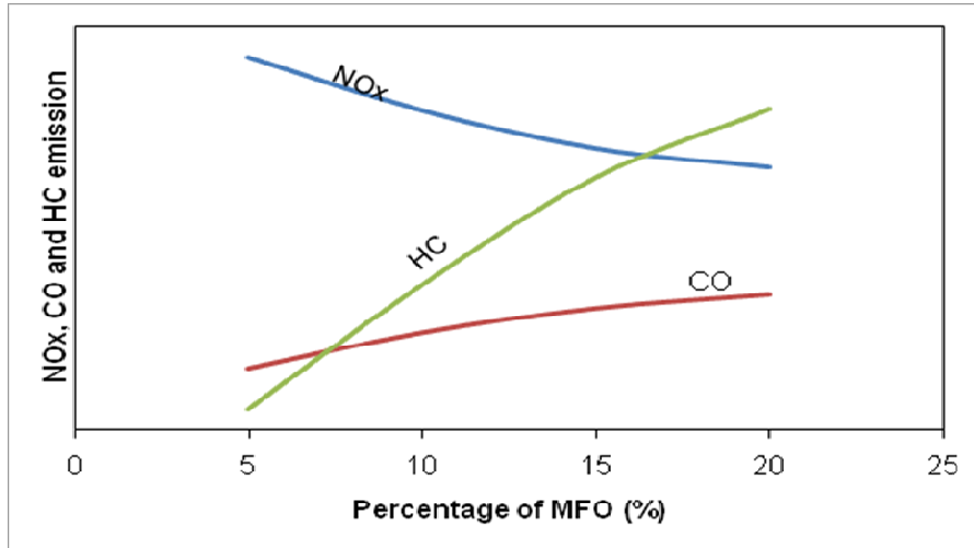
Figure 4.12: Relationship between exhaust emission and MFO percentage
