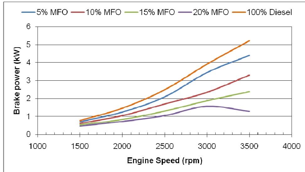
Figure 4.3: BHP versus engine speed
