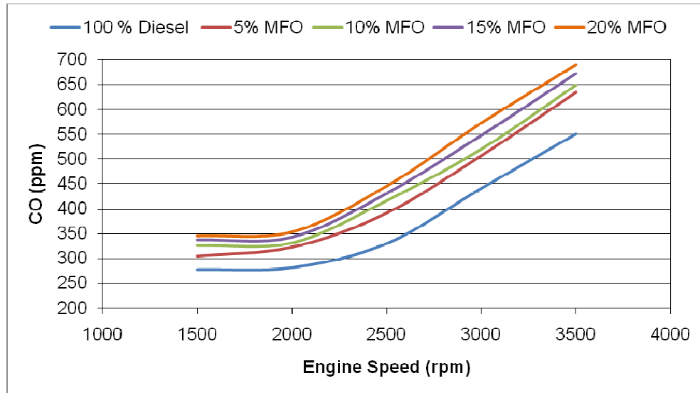
Figure 4.8: CO emission versus engine speed
