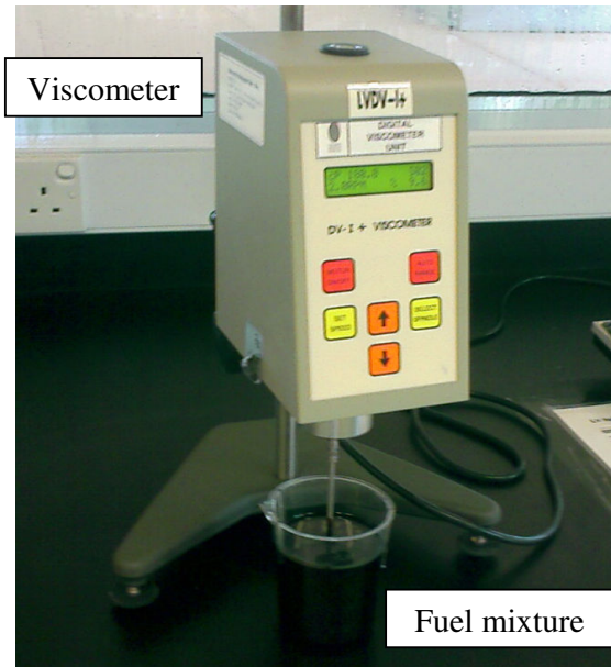
Figure 3.3: Viscometer used
