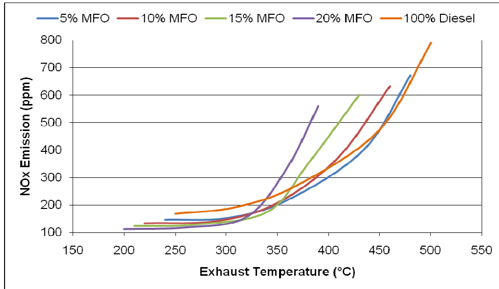
Figure 4.7: Exhaust temperature versus NOx emission
