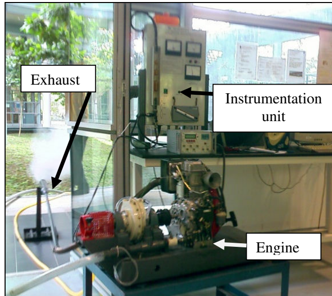
Figure 3.1: Engine test bed and instrumentation
