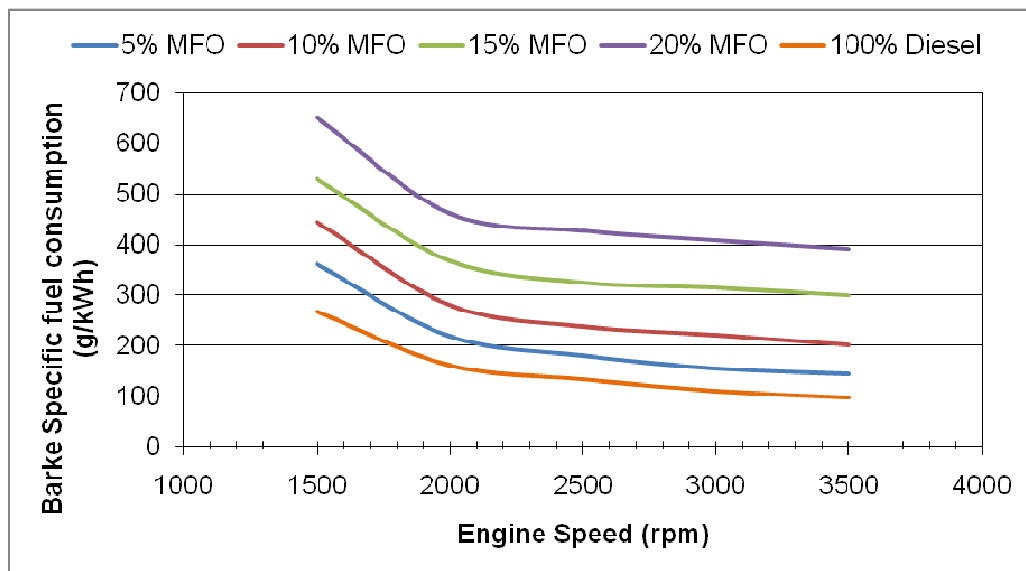
Figure 4.5: BSFC versus engine speed
