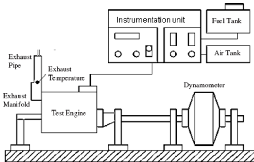
Figure 3.2: Schematic diagram of experimental setup
