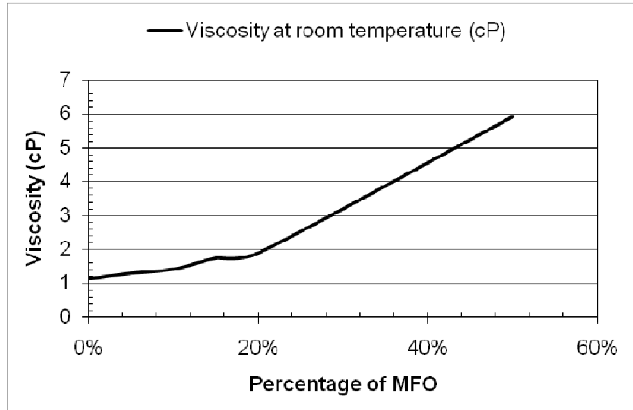
Figure 4.1: Viscosity versus fuel percentage
