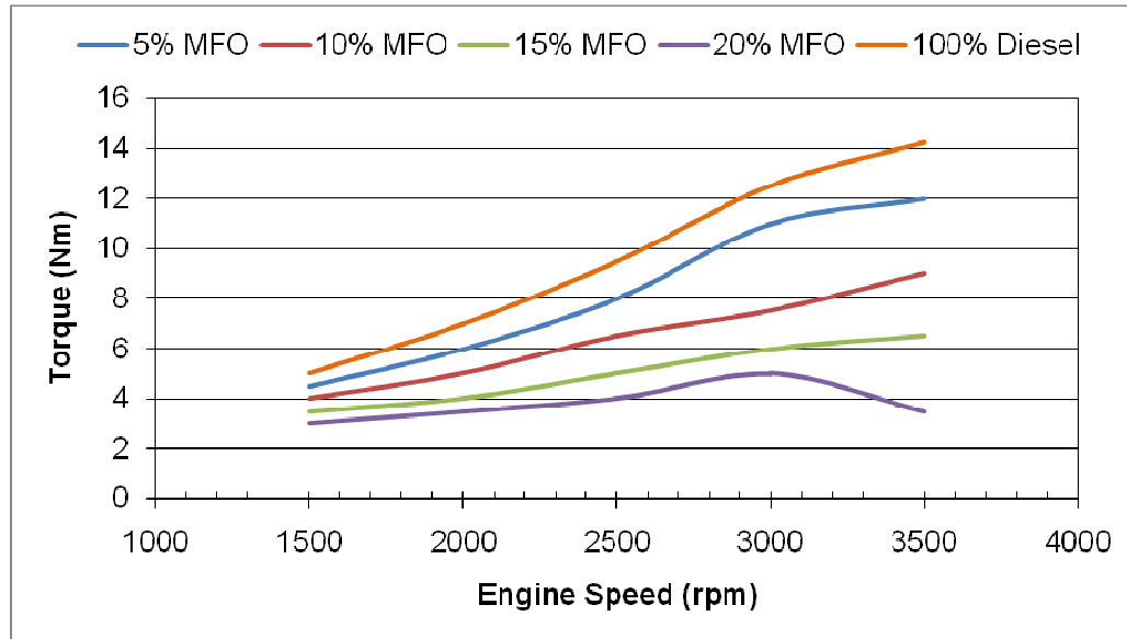
Figure 4.2: Torque versus engine speed
