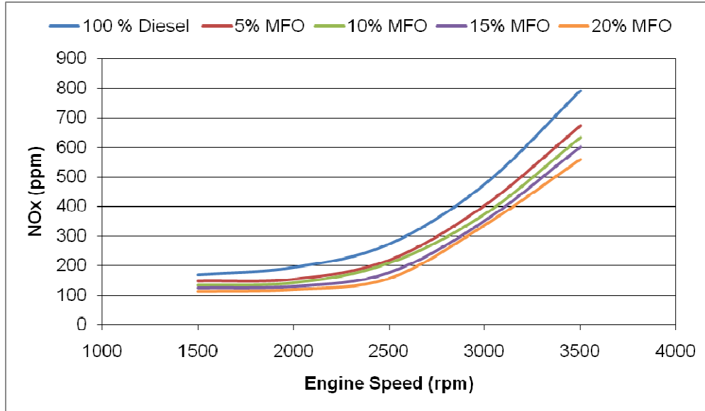
Figure 4.6: NOx emission versus engine speed
