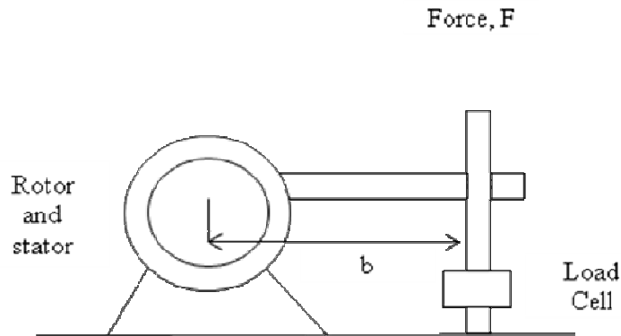
Figure 2.1: Schematic of principle of operation of dynamometer [19]
