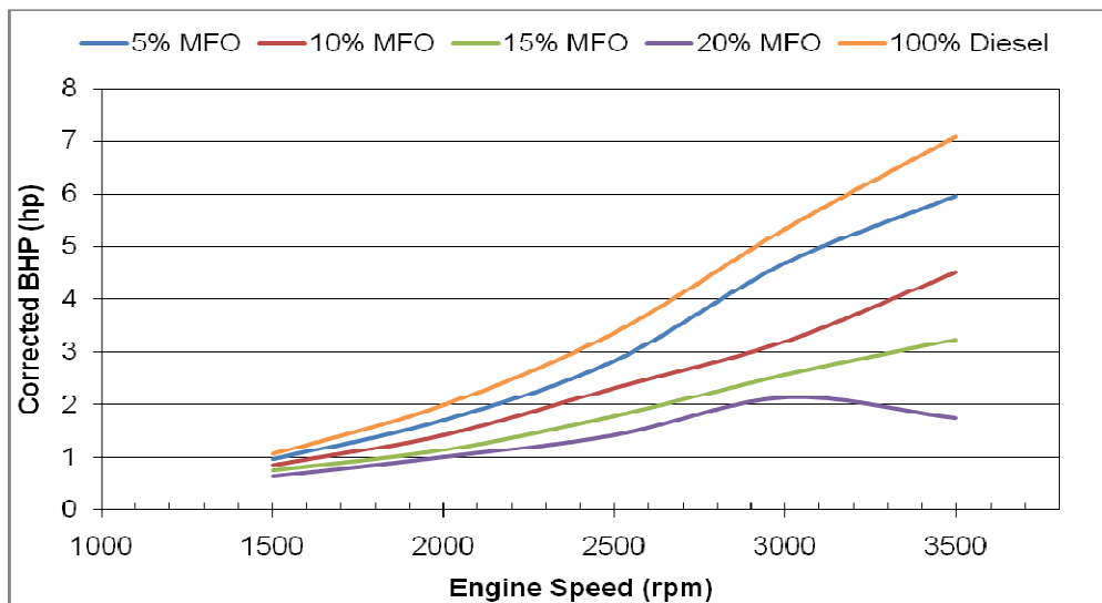
Figure 4.4: Corrected BHP versus engine speed
