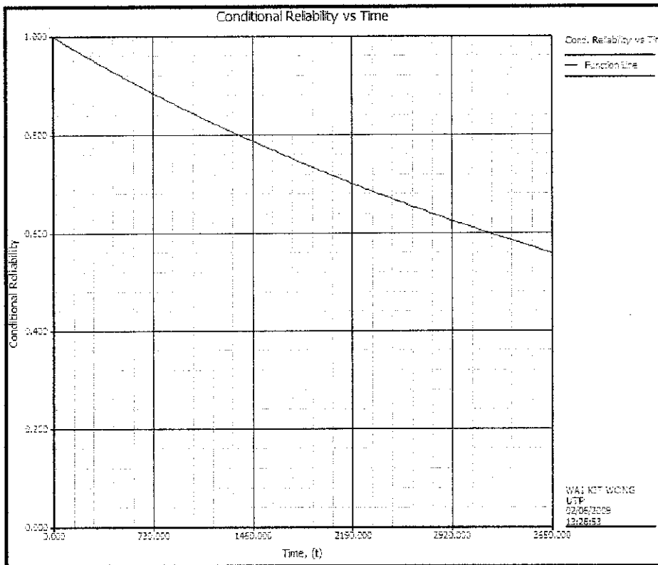
Figure 4.9: Conditional reliability vs. time of mechanical
