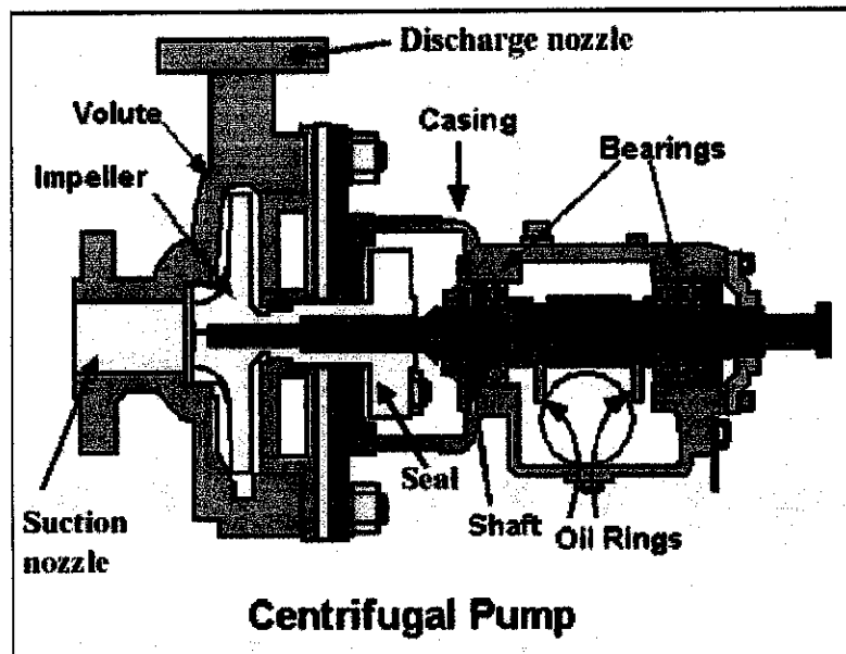
Figure 2.13: Centrifugal Pump [12]
