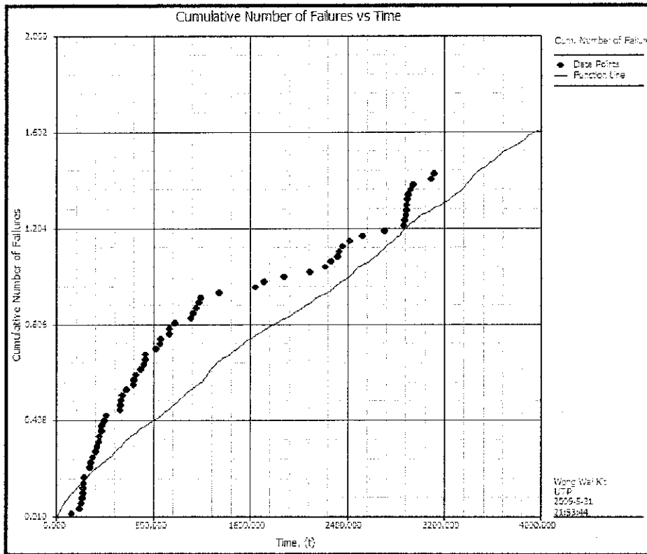
Figure 4.4: Cumulative number of failures vs. time of seal
