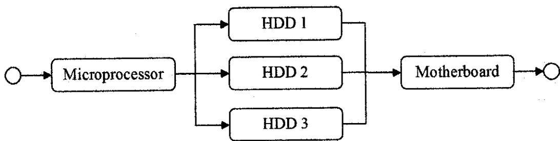
Figure 2.9: RBD of a CPU system in combination configuration
