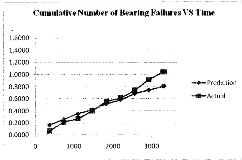
Figure 4.11: Prediction and actual cumulative number of failures for Bearing
