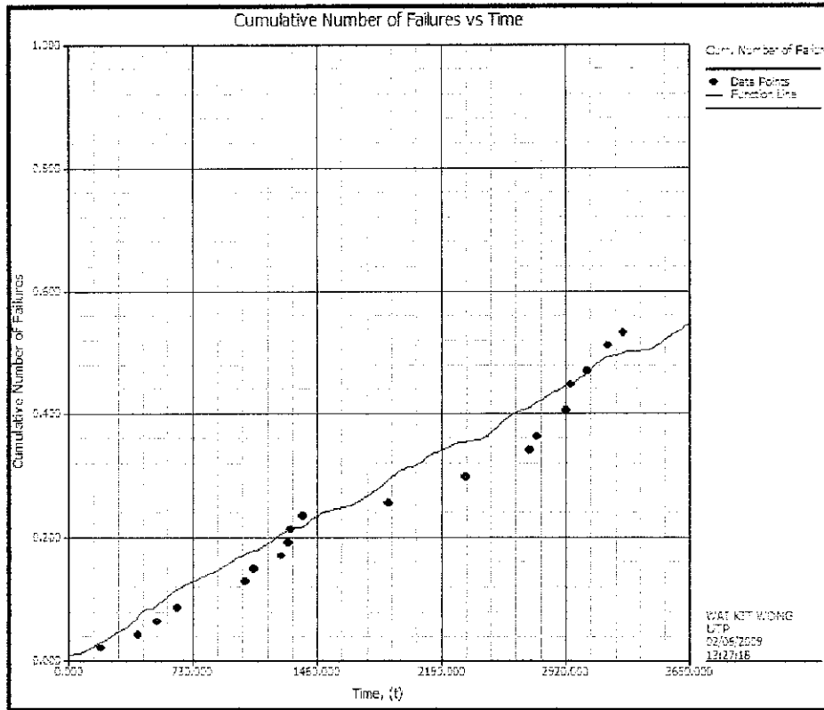
Figure 4.8: Cumulative number of failures vs. time of mechanical
