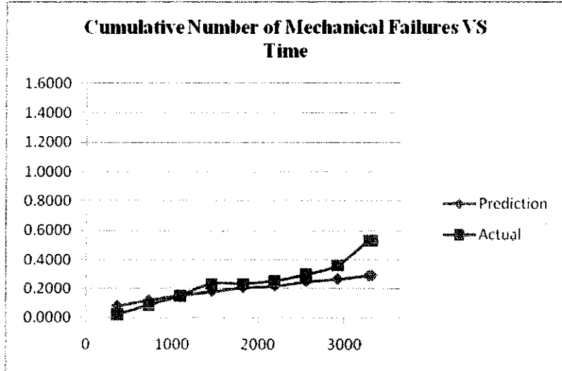
Figure 4.12: Prediction and actual cumulative number of failures for Mechanical
