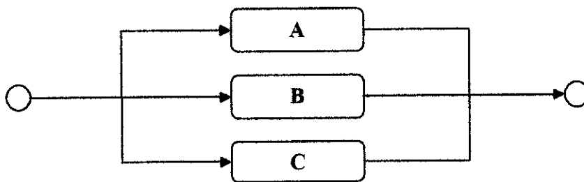
Figure 2.7: RBD in basic parallel configuration
