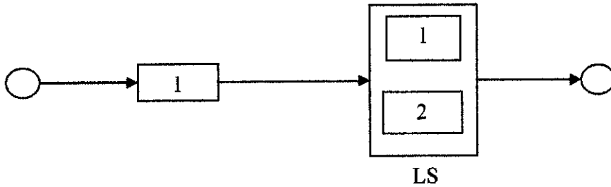
Figure 2.11: RBD of Load Sharing Container
