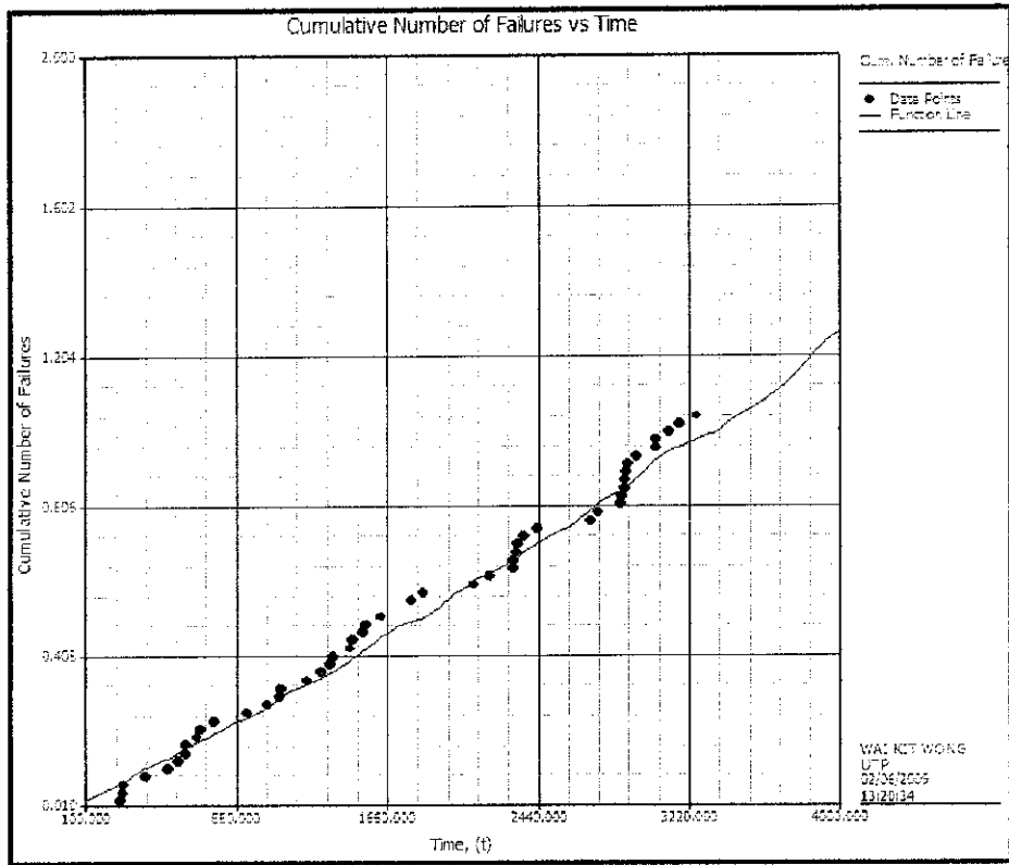
Figure 4.6: Cumulative number of failures vs. time of bearing
