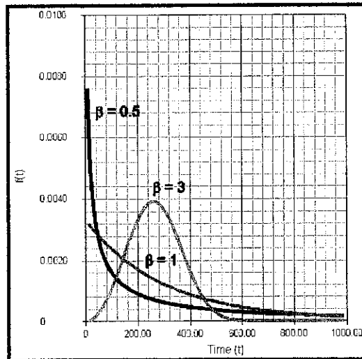
Figure 2.2: Effect of \beta to Weibull PDF
