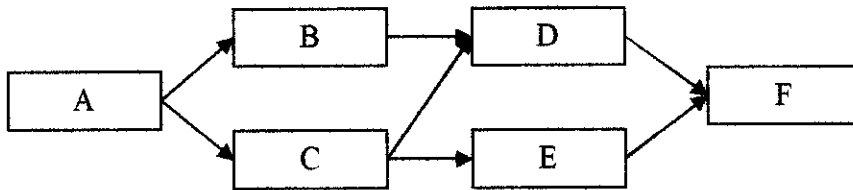
Figure 2.10: RBD of a complex system
