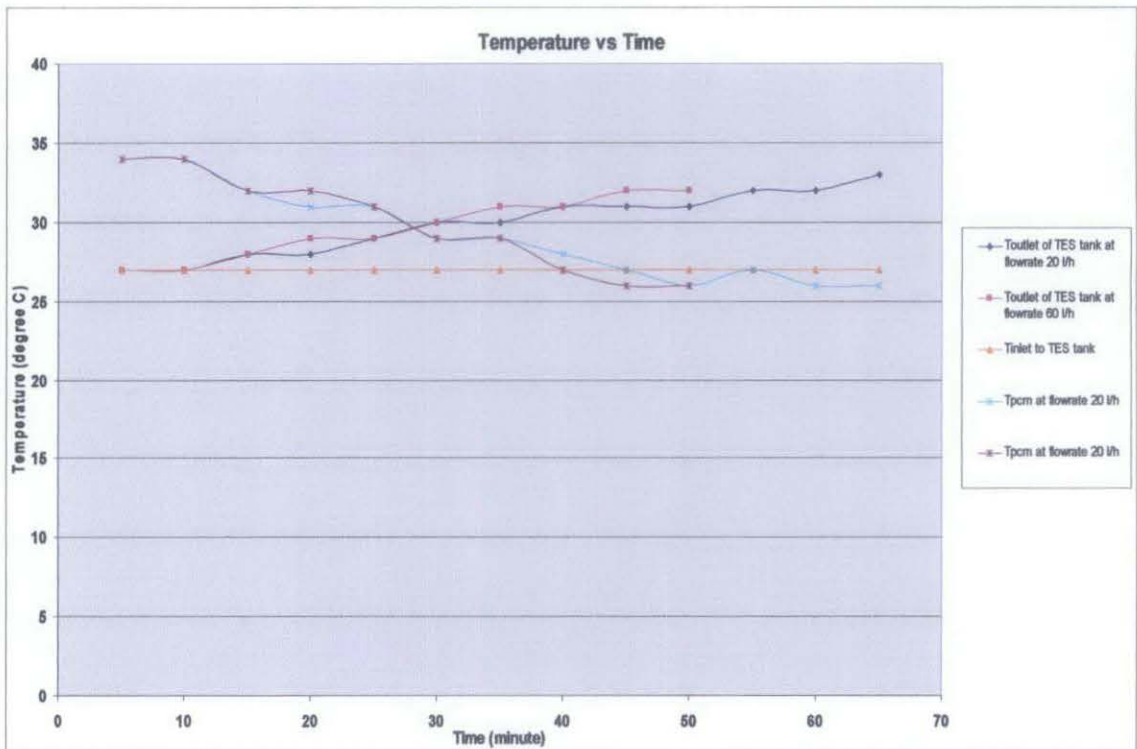
Figure 23: T_{inlet} of TES tank, T_{outlet} TES tank and T_{PCM} at flowrate 20 l/h and 60 l/h versus time
