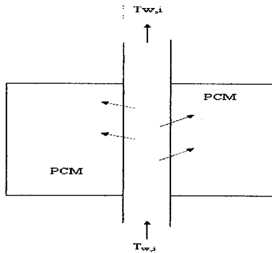
Figure 17: Diagram showing heat transfer form water to the PCM while charging
