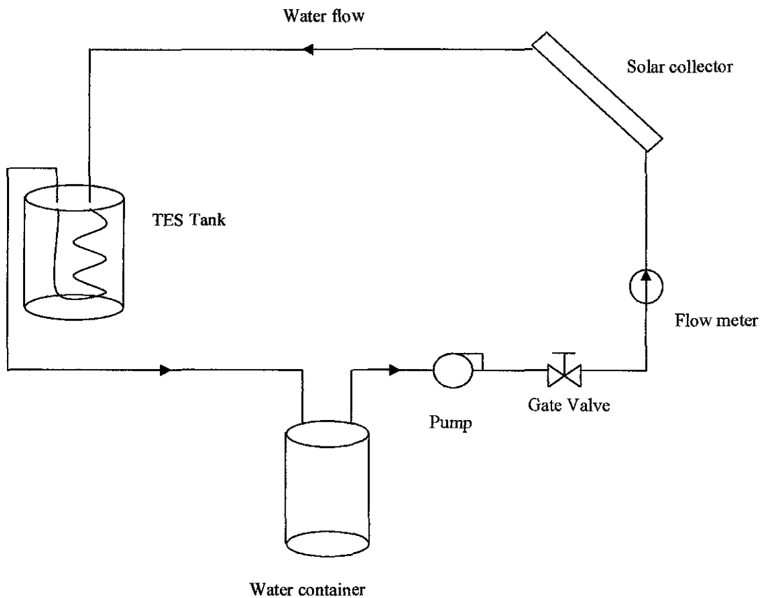
Figure 3: Schematic diagram of TES systems
