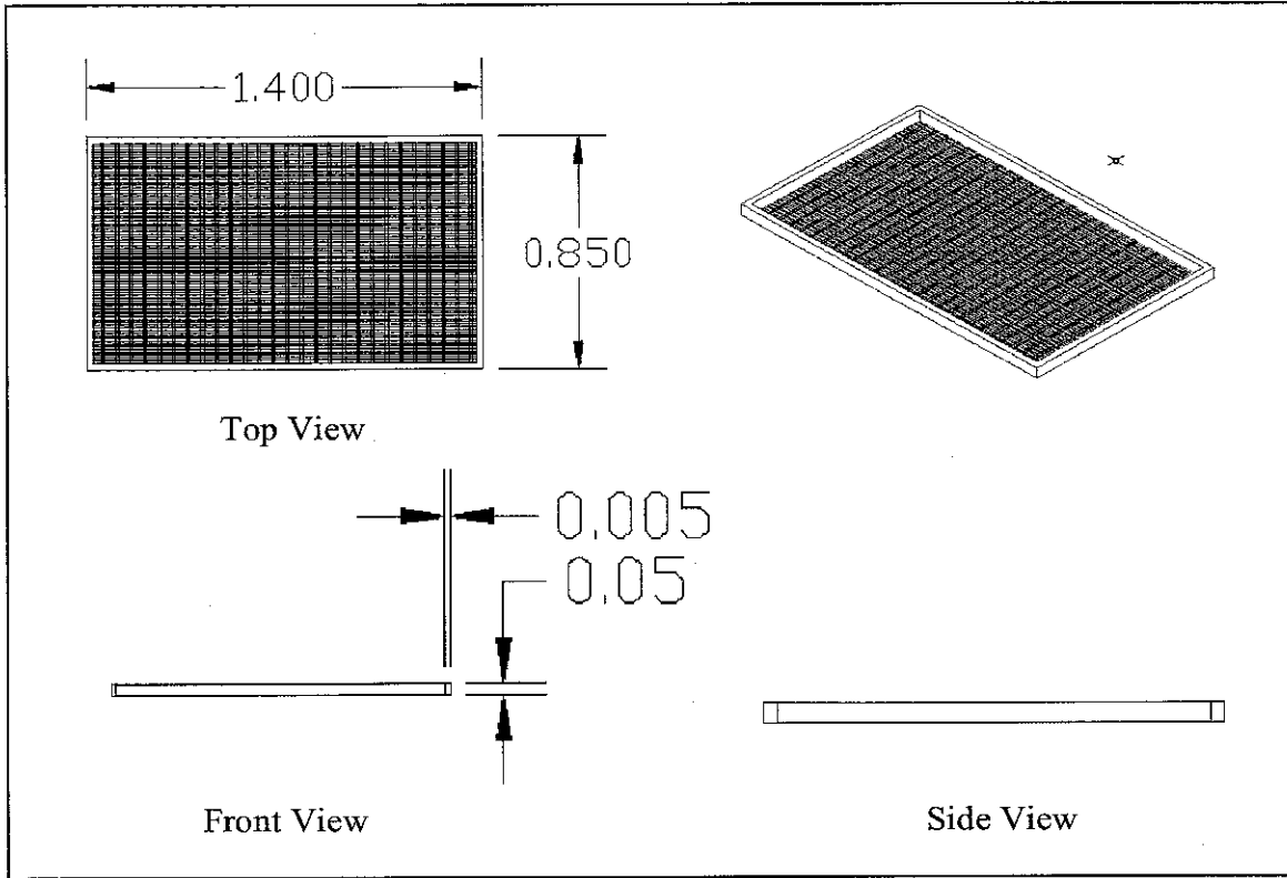
Figure 4.7: Orthographic View of Meshed Tray
