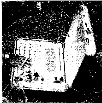
Figure 2.6: Electromagnetic SIROTEM
