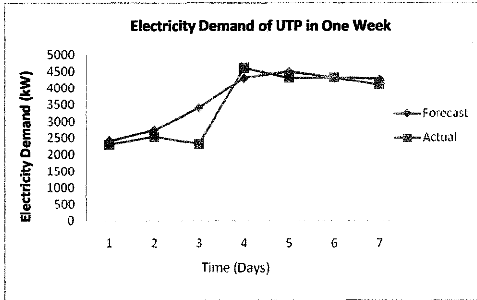
Figure 11: Comparison between Actual and Forecast Load for 11 Hidden Neurons
