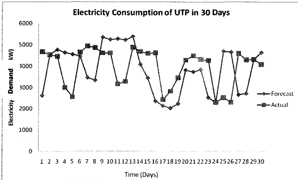
Figure 29: Comparison between Actual and Forecast Load for 11 Hidden Neurons
