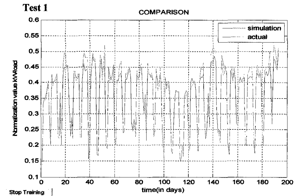
Figure 13: Test 1 Result using training data
