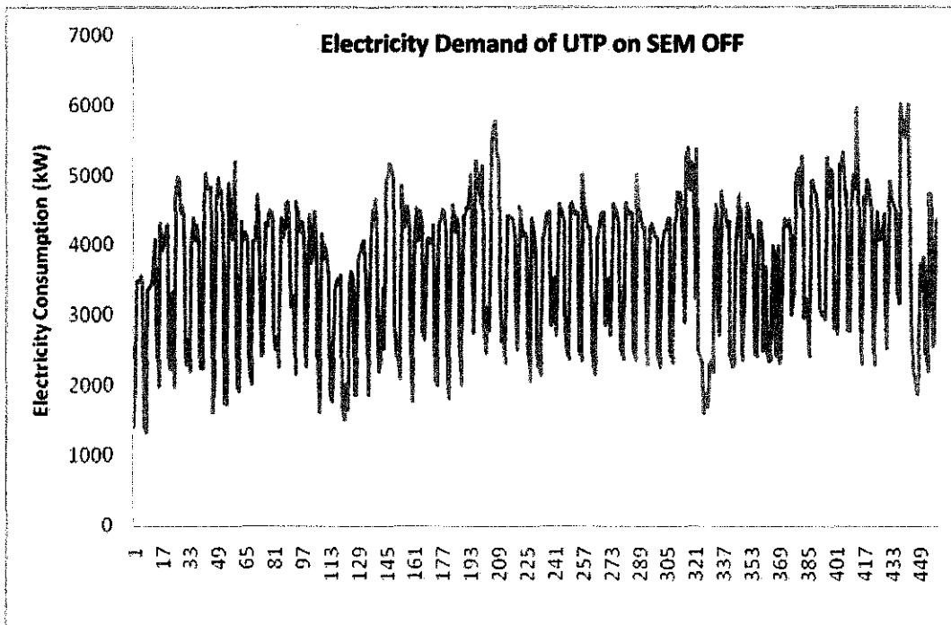
Figure 4: Graph of Electricity Demand of UTP on Semester OFF
