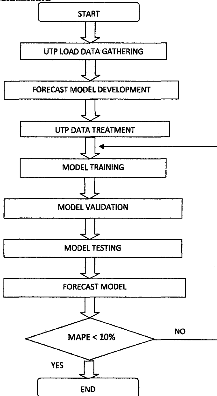
Figure 7: Project's Methodology
