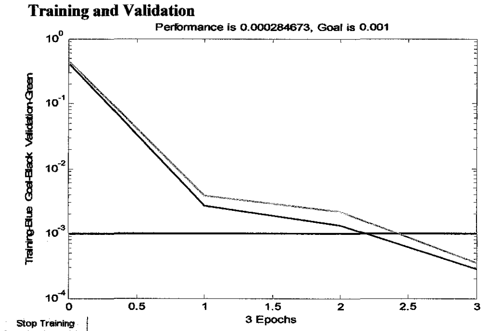
Figure 39: Training and Validation of Model 4 with 3 Neurons
