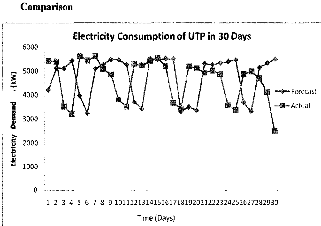
Figure 42: Comparison between Actual and Forecast Load for 3 Hidden Neurons
