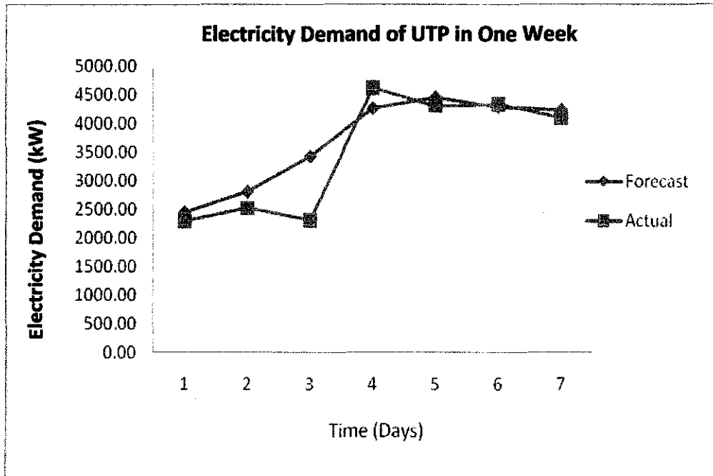
Figure 9: Comparison between Actual and Forecast Load for 7 Hidden Neurons
