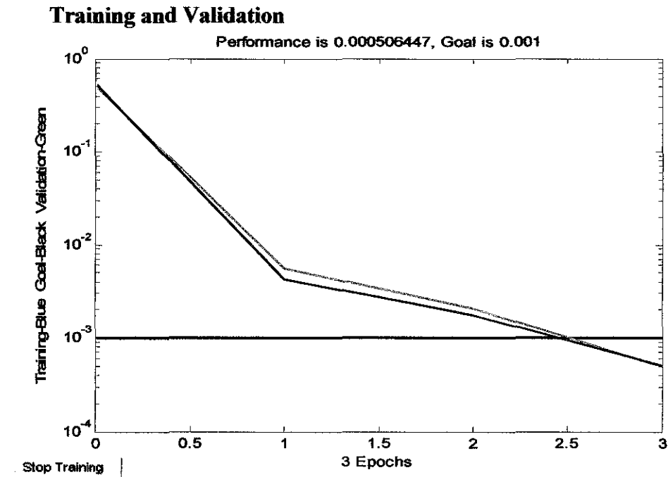
Figure 30: Training and Validation of Model 3 with 3 neurons
