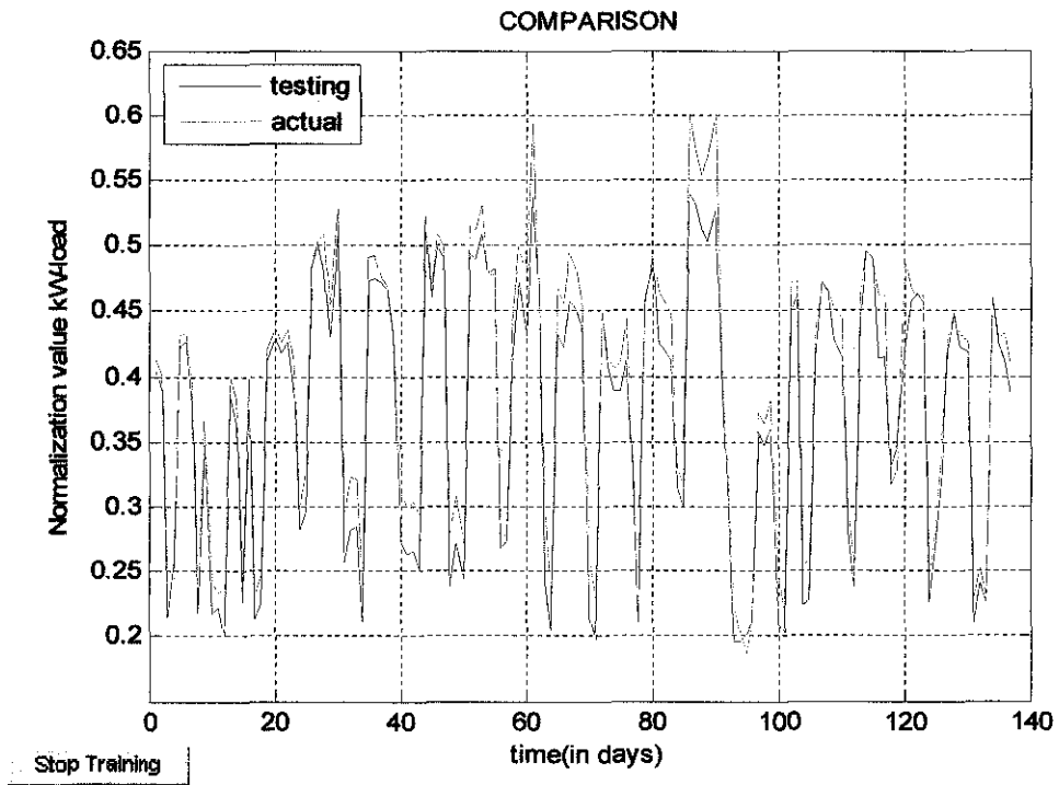
Figure 32: Test 2 result using testing data
