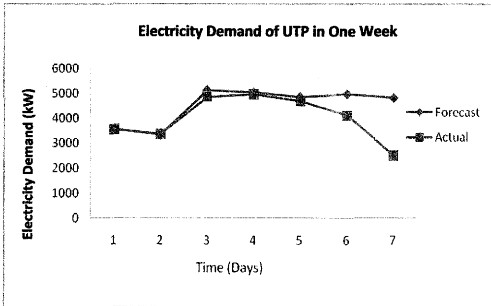
Figure 18: Comparison between Actual and Forecast Load for 7 Hidden Neurons
