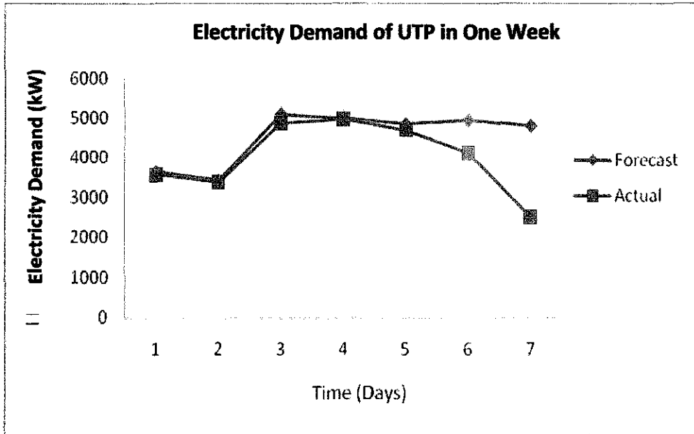
Figure 16: Comparison between Actual and Forecast Load for 3 Hidden Neurons
