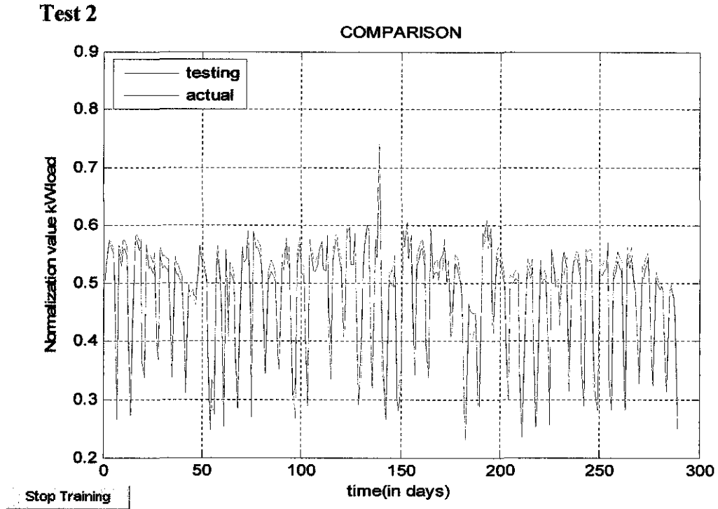
Figure 23: Test 2 result using testing data
