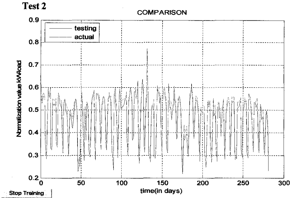
Figure 41: Test 2 result using testing data
