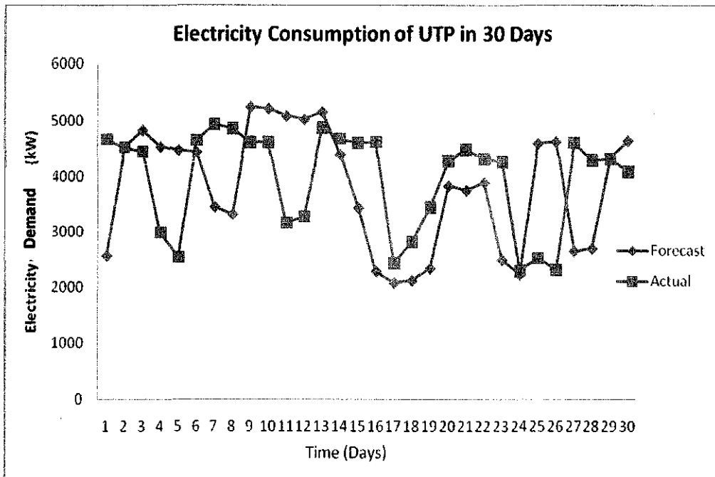
Figure 28: Comparison between Actual and Forecast Load for 9 Hidden Neurons
