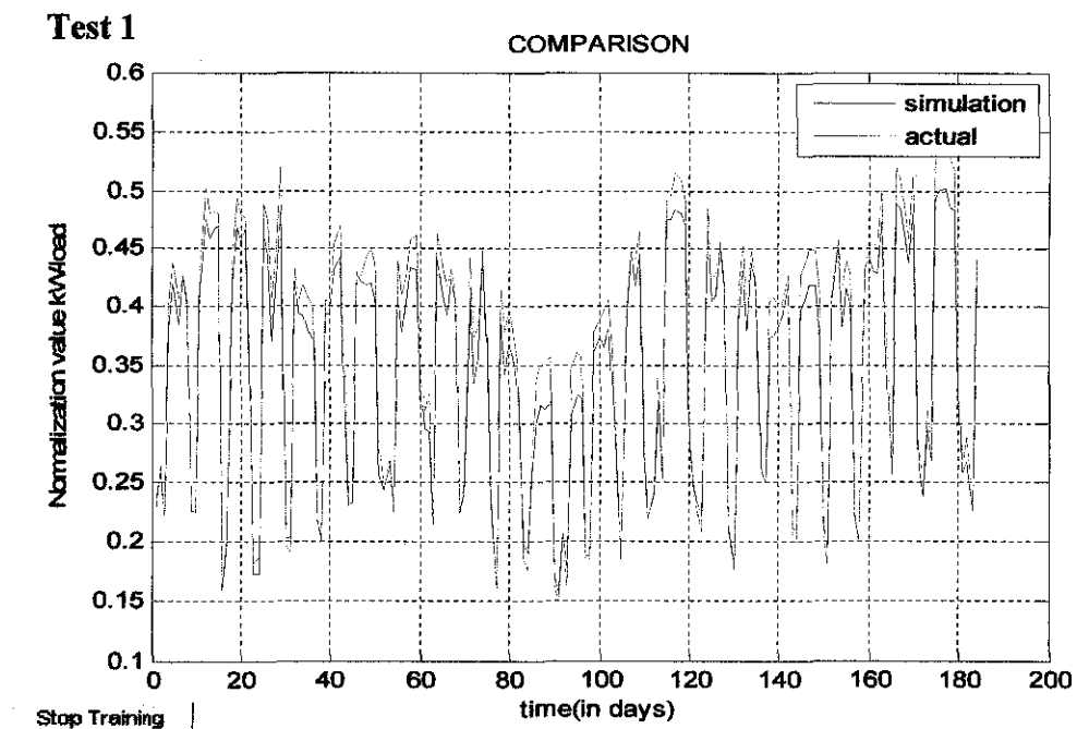
Figure 31: Test 1 result using training data
