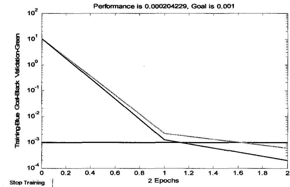
Figure 12: Training and Validation of Model 1 with 3 neurons
