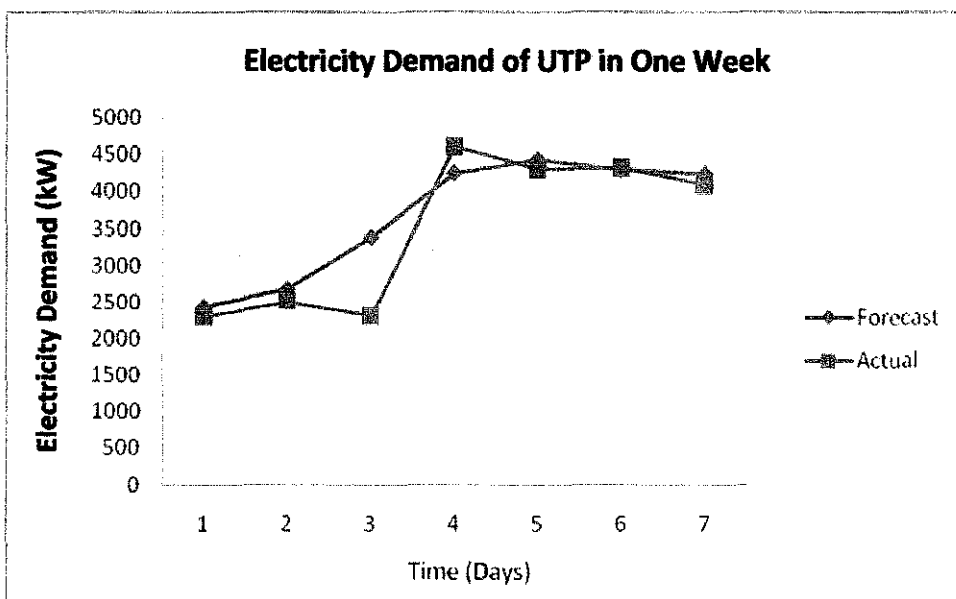
Figure 8: Comparison between Actual and Forecast Load for 5 Hidden Neurons
