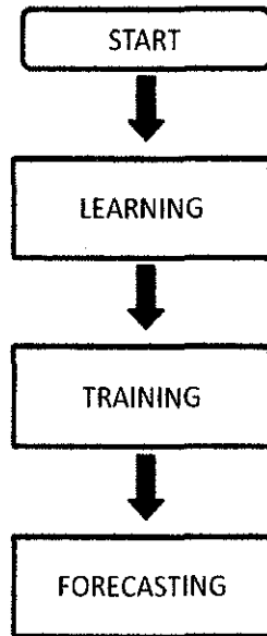
Figure 2: ANN Process
