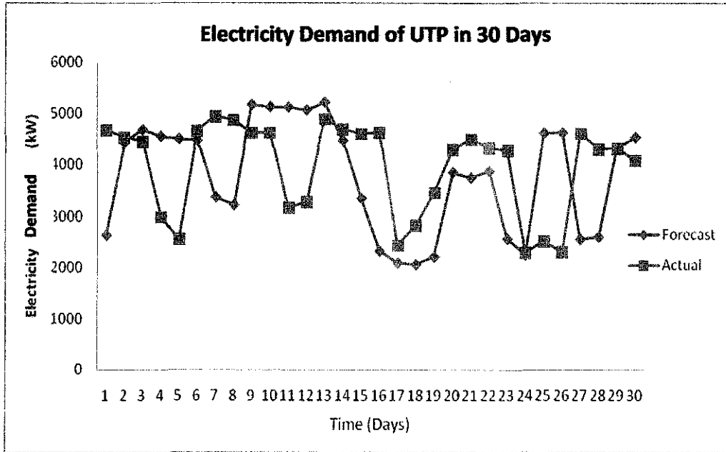
Figure 27: Comparison between Actual and Forecast Load for 7 Hidden Neurons
