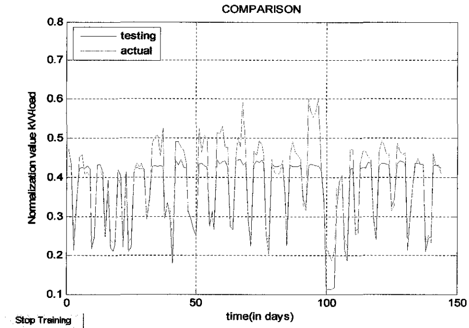
Figure 14: Test 2 result using testing data
