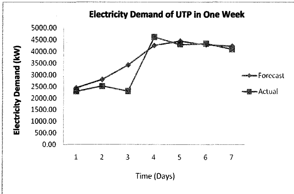
Figure 15: Comparison between Actual and Forecast Load for 7 Hidden Neurons
