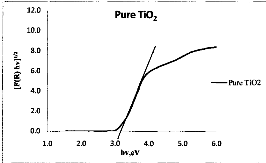
Figure C.1: DR-UV-Vis spectra for TiO 2
