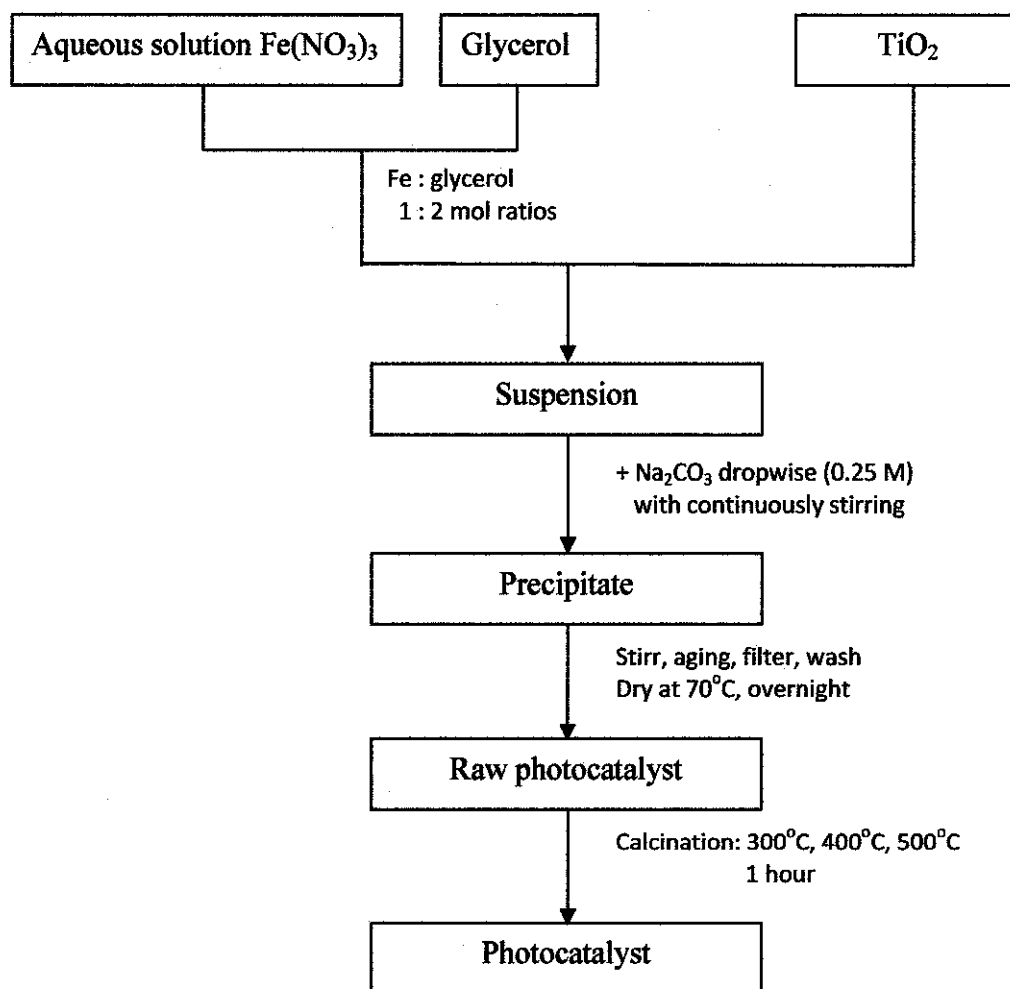
Figure 3.1: Process flow for catalyst preparation and pretreatment
