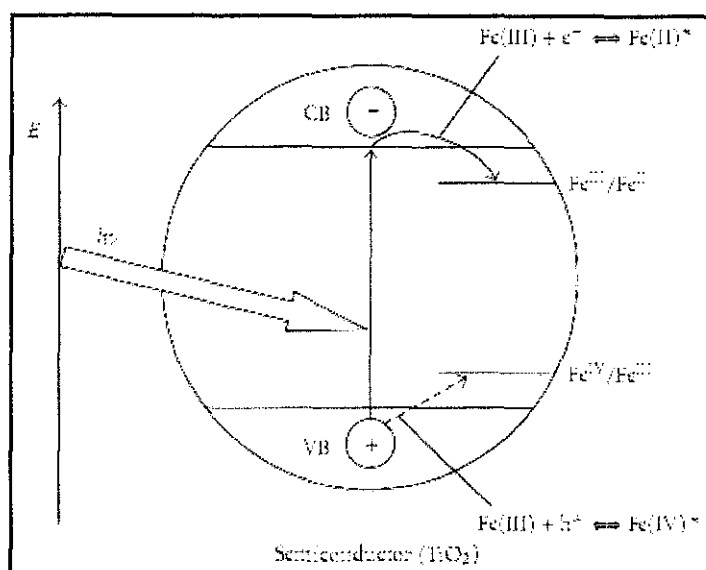
Figure 2.3: Scheme of mechanism of TiO 2 photocatalysis with modification by Fe (III) ion doping
