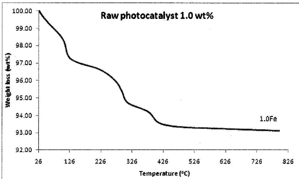
Figure 4.3: Thermal decomposition of 1.0 wt% Fe/TiO 2 raw photocatalyst
