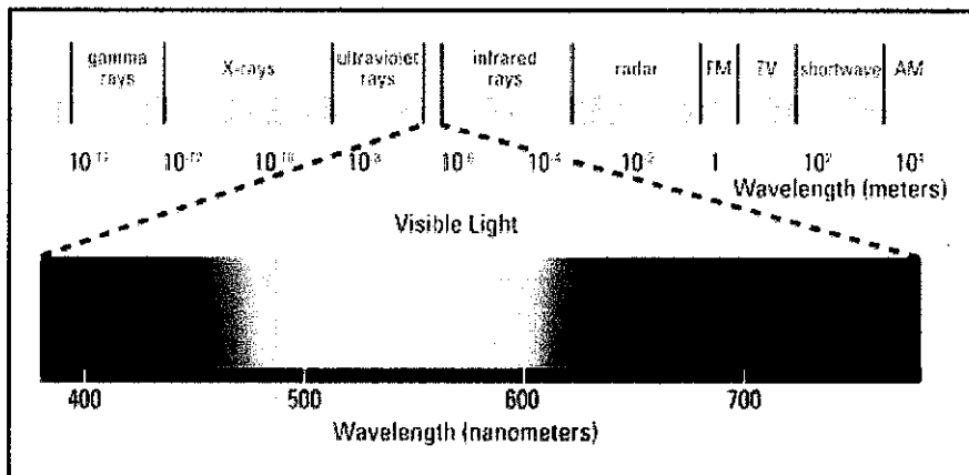
Figure 2.1: Electromagnetic Spectrum
