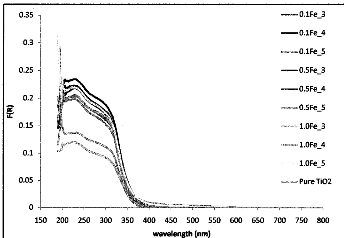
Figure 4.4: DR-UV-Vis spectra of pure \text{TiO}_2 and \text{Fe}/\text{TiO}_2
