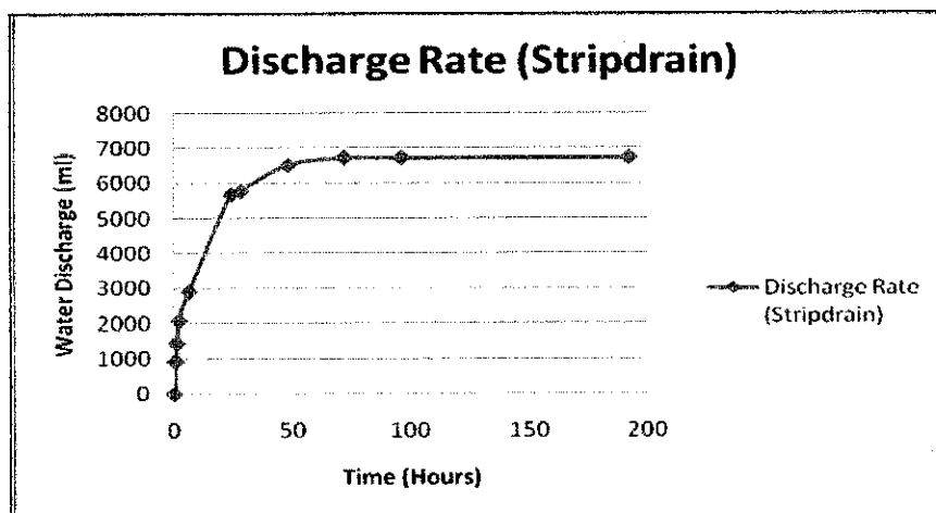
Figure 4.1: Discharge Capacity Graph (Stripdrain™)
