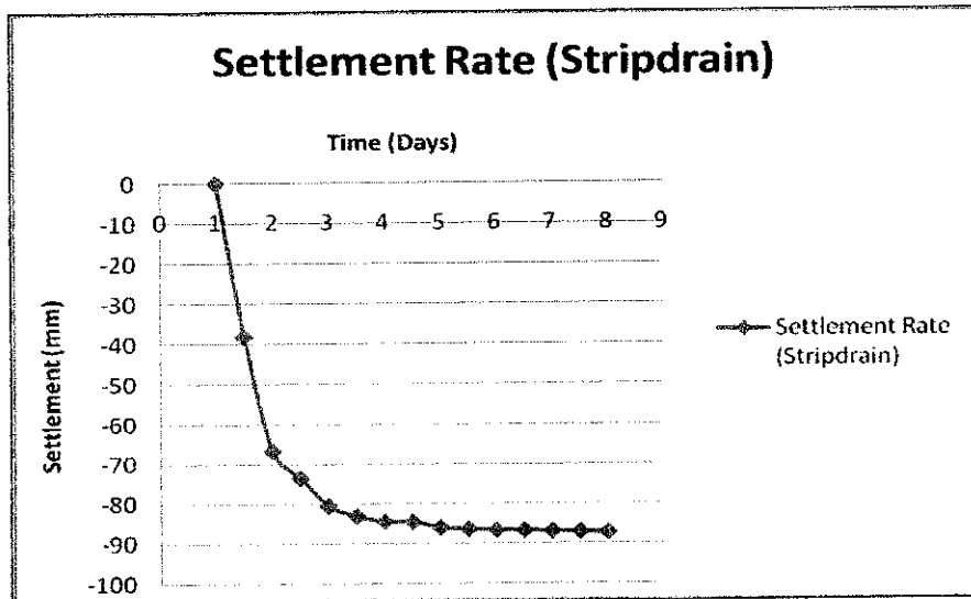
Figure 4.2: Settlement Rate (Stripdrain tm )
