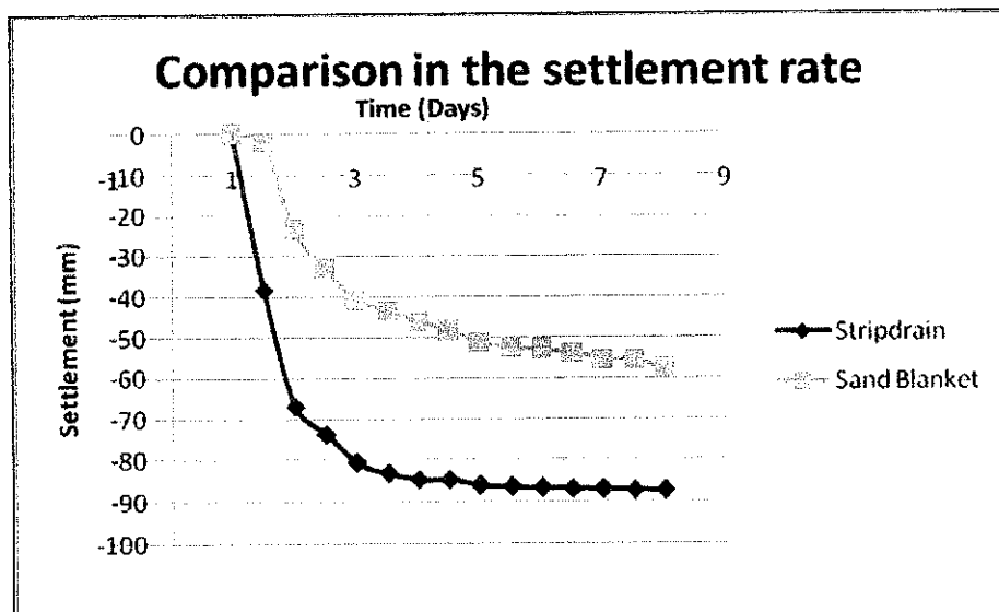
Figure 4.6: Comparison in the settlement rate
