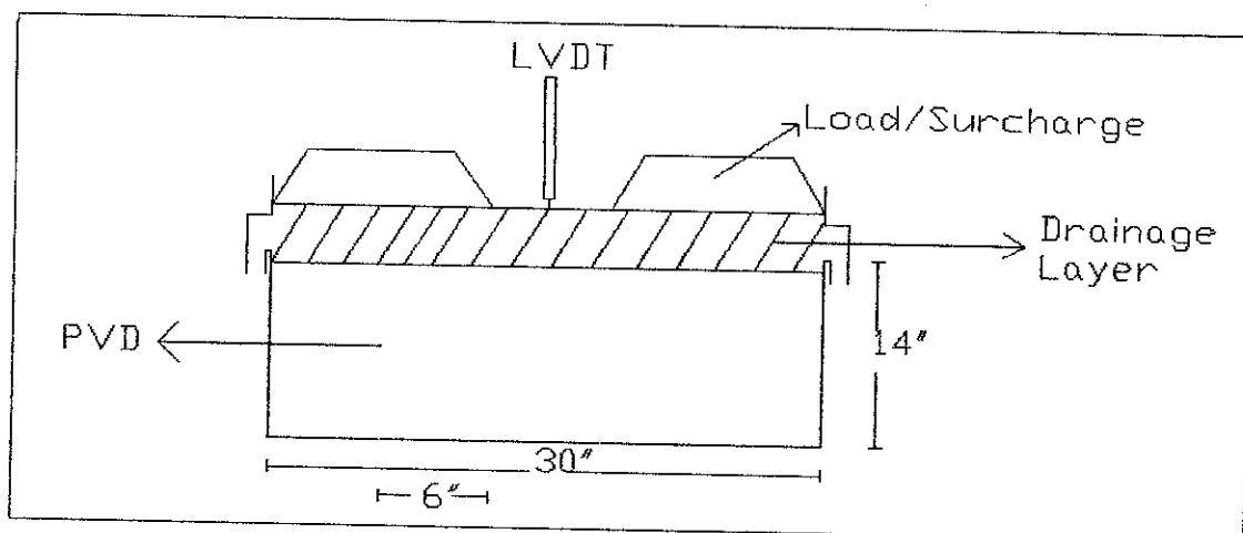
Figure 3.3 : Schematic Diagram of the Experiment
