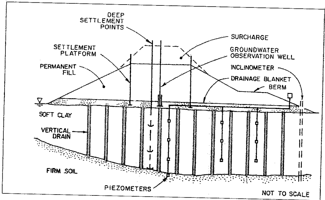
Figure 2.1: Typical vertical drain installation for a highway embankment ( after Rixner et al. 1986)
