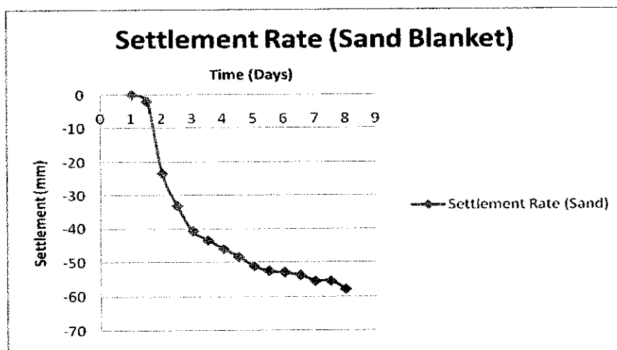
Figure 4.4: Settlement Rate (Sand Blanket)
