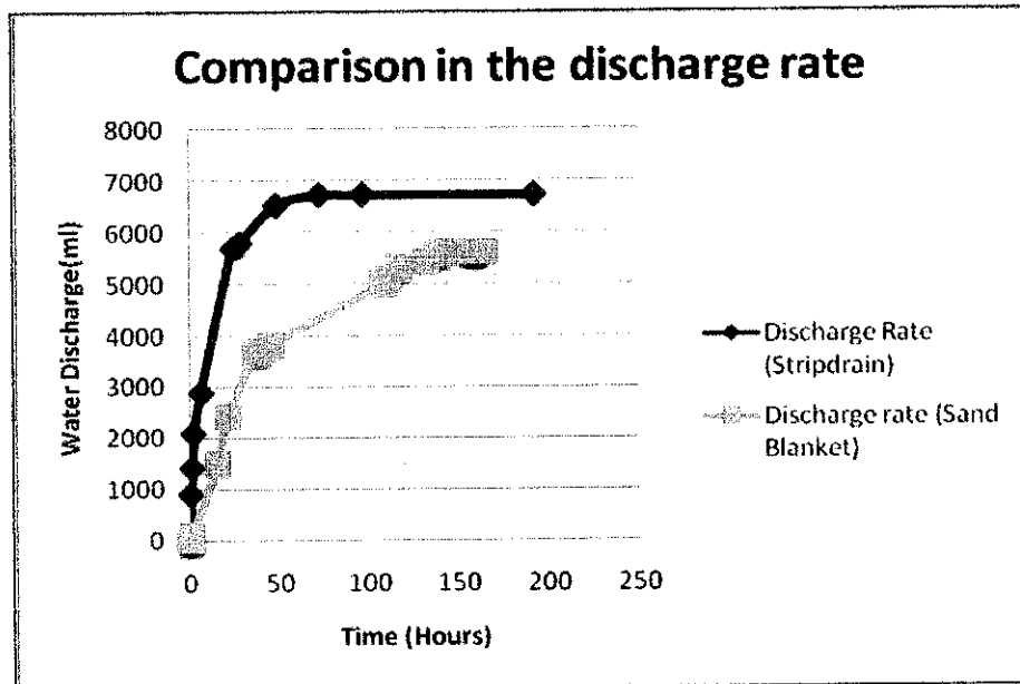
Figure 4.5: Comparison in the discharge rate
