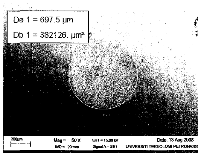
FIGURE 4.9: 85% Palm Oil + 15% Petronas Mach 5 wear scar diameter
