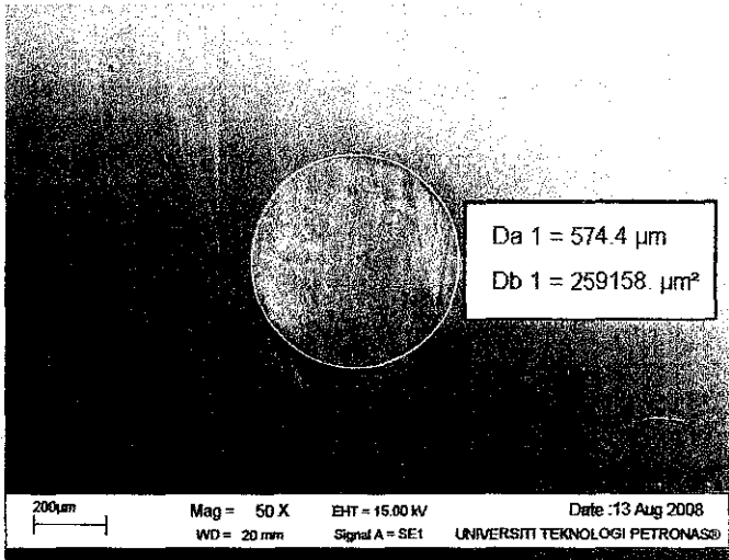
FIGURE 4.5: 100% Petronas Mach 5 wear scar diameter
