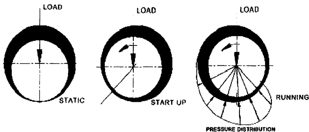
FIGURE 2.2: The picture illustrated the operation of the hydrodynamic lubrication in the journal bearing.
