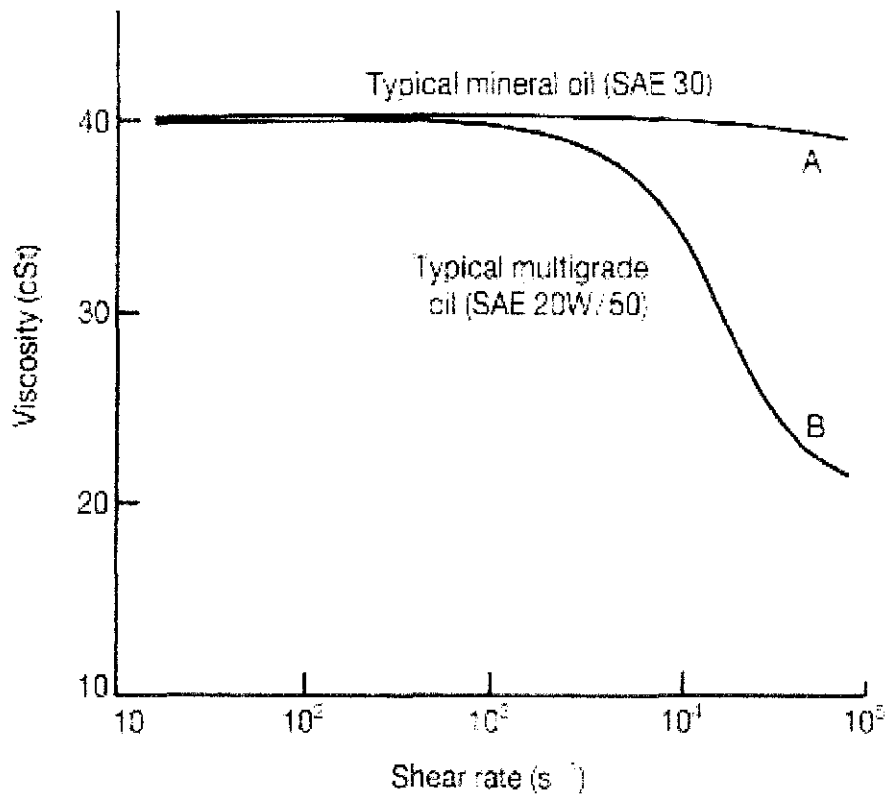
FIGURE 2.6: The variation of viscosity with shear rate for two mineral oils with the same viscosity at low shear rates. Oil A is a plain mineral oil, while oil B contains viscosity index improvers which lose their effectiveness at high shear rates.
