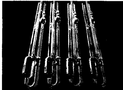
FIGURE 3.2: Pictures of the Tamson Viscometer Unit and the Ubbelohde.
