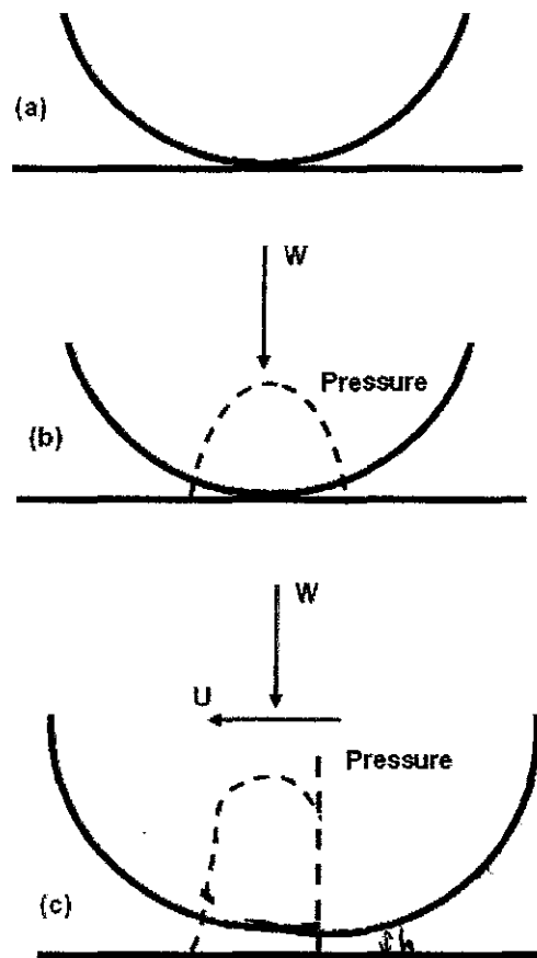
FIGURE 2.3: The picture illustrated the contact between a sphere and a plane under condition of elastohydrodynamic lubrication.
