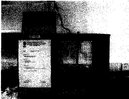
FIGURE 3.2: Pictures of the Tamson Viscometer Unit and the Ubbelohde.
