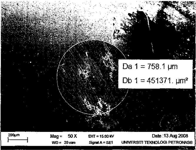
FIGURE 4.8: 90% Palm Oil + 10% Petronas Mach 5 wear scar diameter
