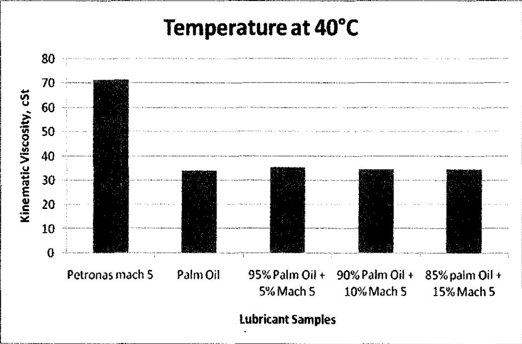
FIGURE 4.1: Experiment result at temperature 40°C
