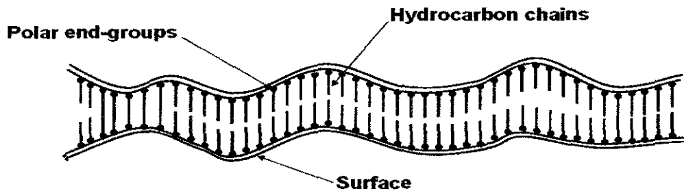
FIGURE 2.4: The mechanism of operation of a boundary lubricant. Polar end-groups on the Hydrocarbon chains bond to the surfaces, providing layers of lubricant molecules which reduce direct contact between the asperities.
