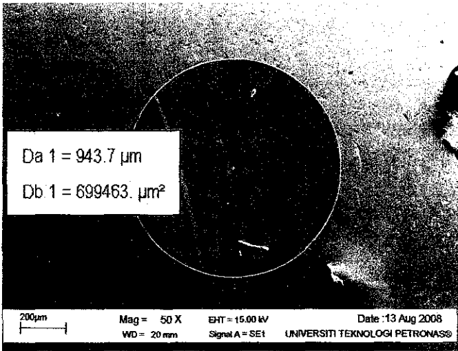
FIGURE 4.6: 100% Palm Oil wear scar diameter
