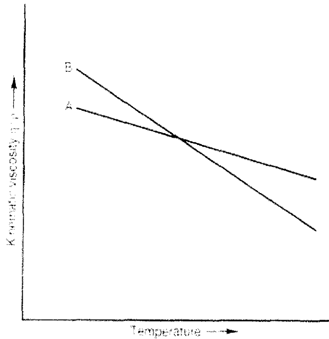
FIGURE 2.5: The graph shown the variation of kinematic viscosity with temperature for two mineral oils. Oil A has a higher viscosity index than oil B.
