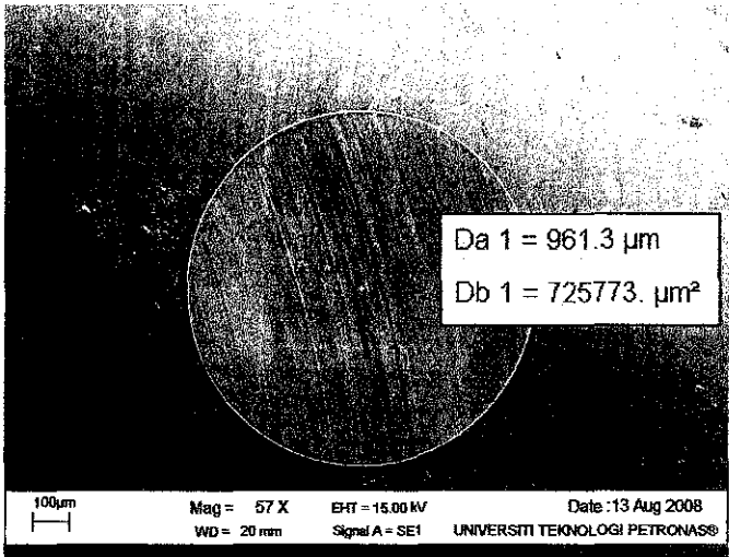
FIGURE 4.7: 95% Palm Oil + 5% Petronas Mach 5 wear scar diameter
