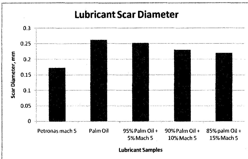
FIGURE 4.4: Lubricants scar diameter
