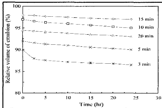
Figure 11: Effect of mixing time on emulsification
