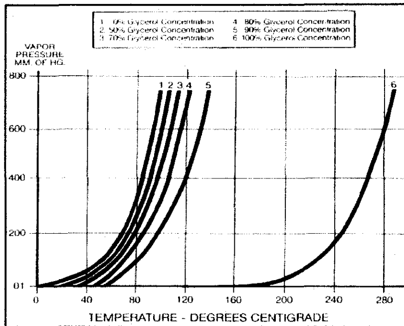
Figure 3: Graph of aqueous solution of glycerol versus temperature
