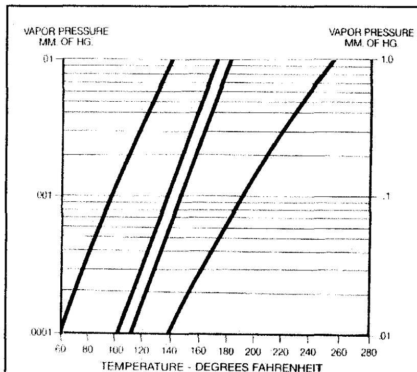
Figure 2: Graph of vapor pressure of 100% glycerol versus temperature
