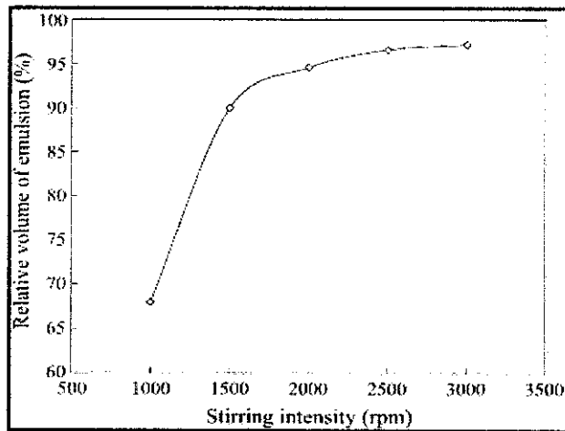
Figure 10: The relationship between stirring intensity and relative emulsion volume after 24 h.
