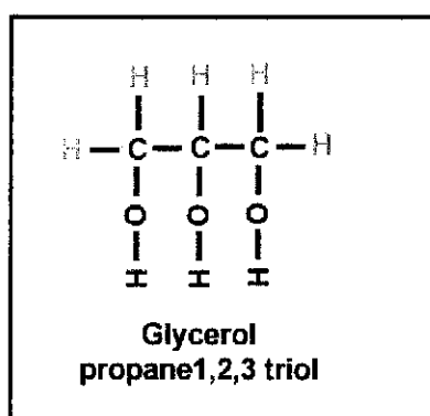
Figure 1: Molecular Structure of Glycerol
