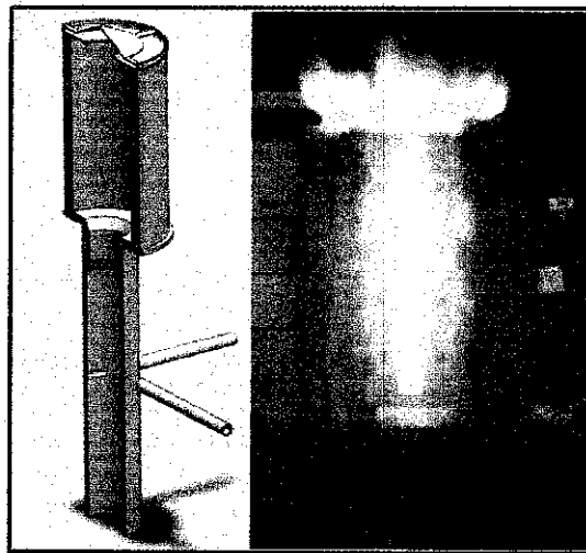
Figure 13: Refractory burner for glycerol combustion
