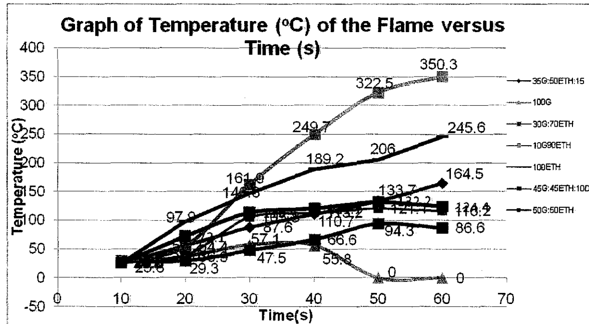
Figure 20: Graph of temperature of the flame versus time
