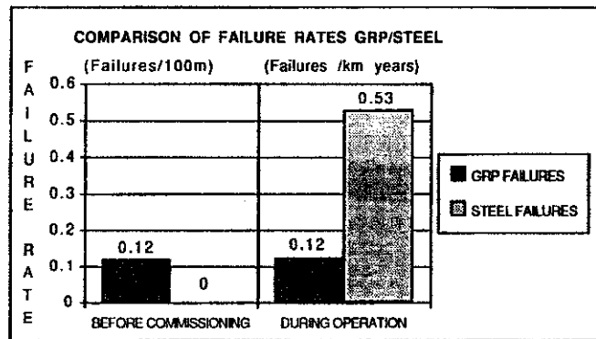
Figure 2.6: The performance of GFRP piping system in sea water conditions compared to the steel [2]
