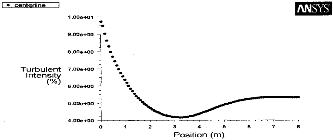
Figure 13: GFRP pipe, turbulent intensity vs. pipe length
