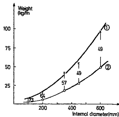
Figure 2.6.1: Dimension vs. Weight for the GFRP (2) and the steel pipe (1) [3]
