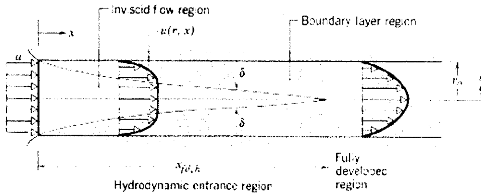
Figure 2.5: hydrodynamic entrance region
