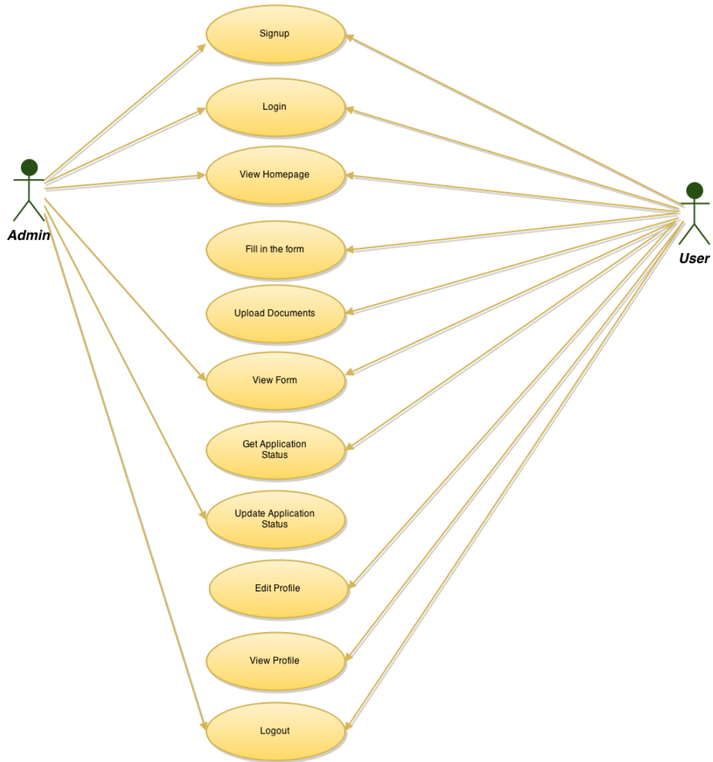
Figure 13: TAZUTP Use Case
