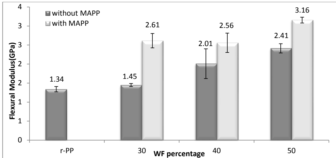
Figure 4.3: The effects of WF percentage and MAPP on flexural modulus.
