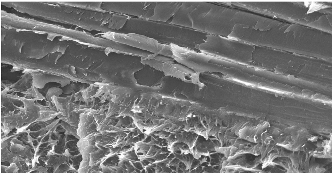
Figure 4.8: Composite microstructure with coupling agent
