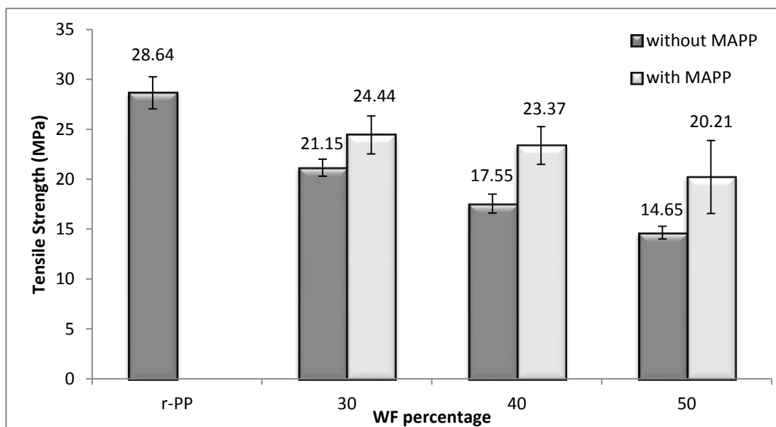
Figure 4.1: The effects of WF percentage and MAPP on tensile strength.
