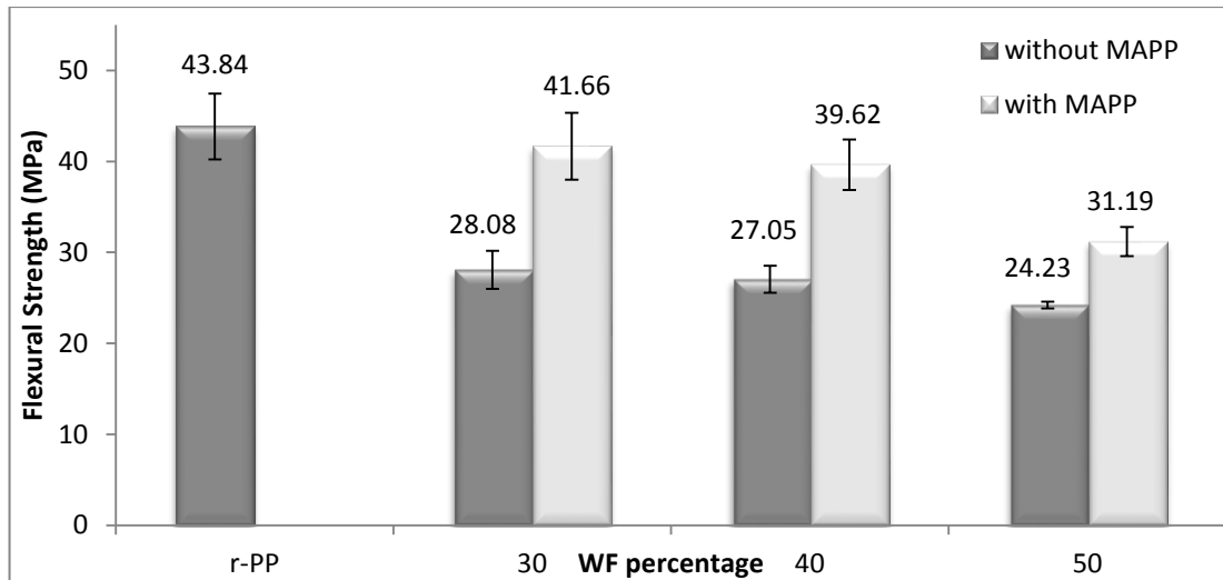
Figure 4.2: The effects of WF percentage and MAPP on flexural strength.
