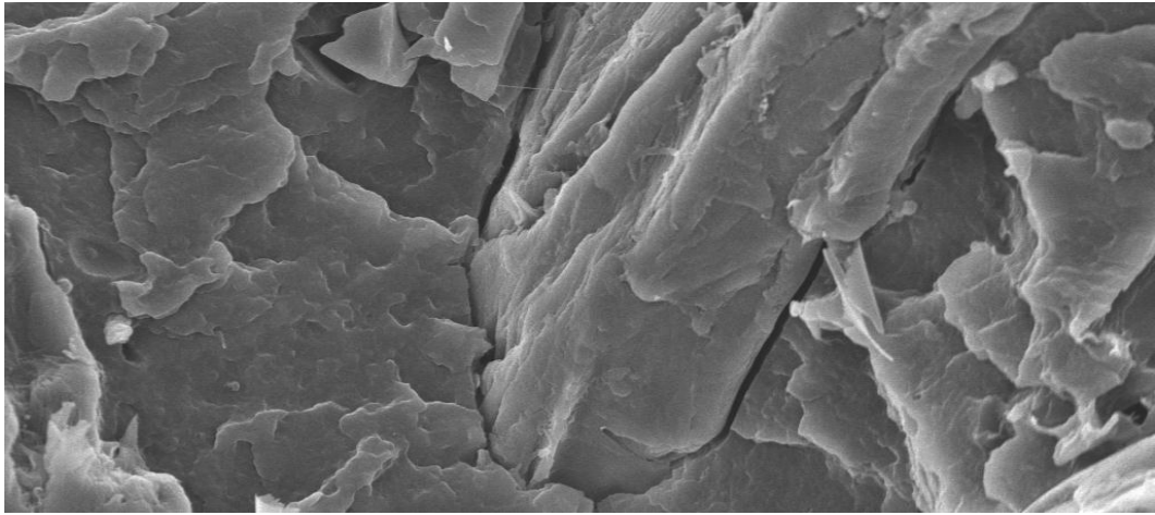
Figure 4.7: Composite microstructure without coupling agent
