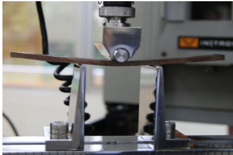
Figure 3.10: Three-point Bending Flexural testing.
