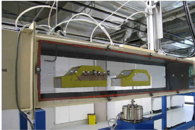
Figure A1: Real Wind Tunnel
