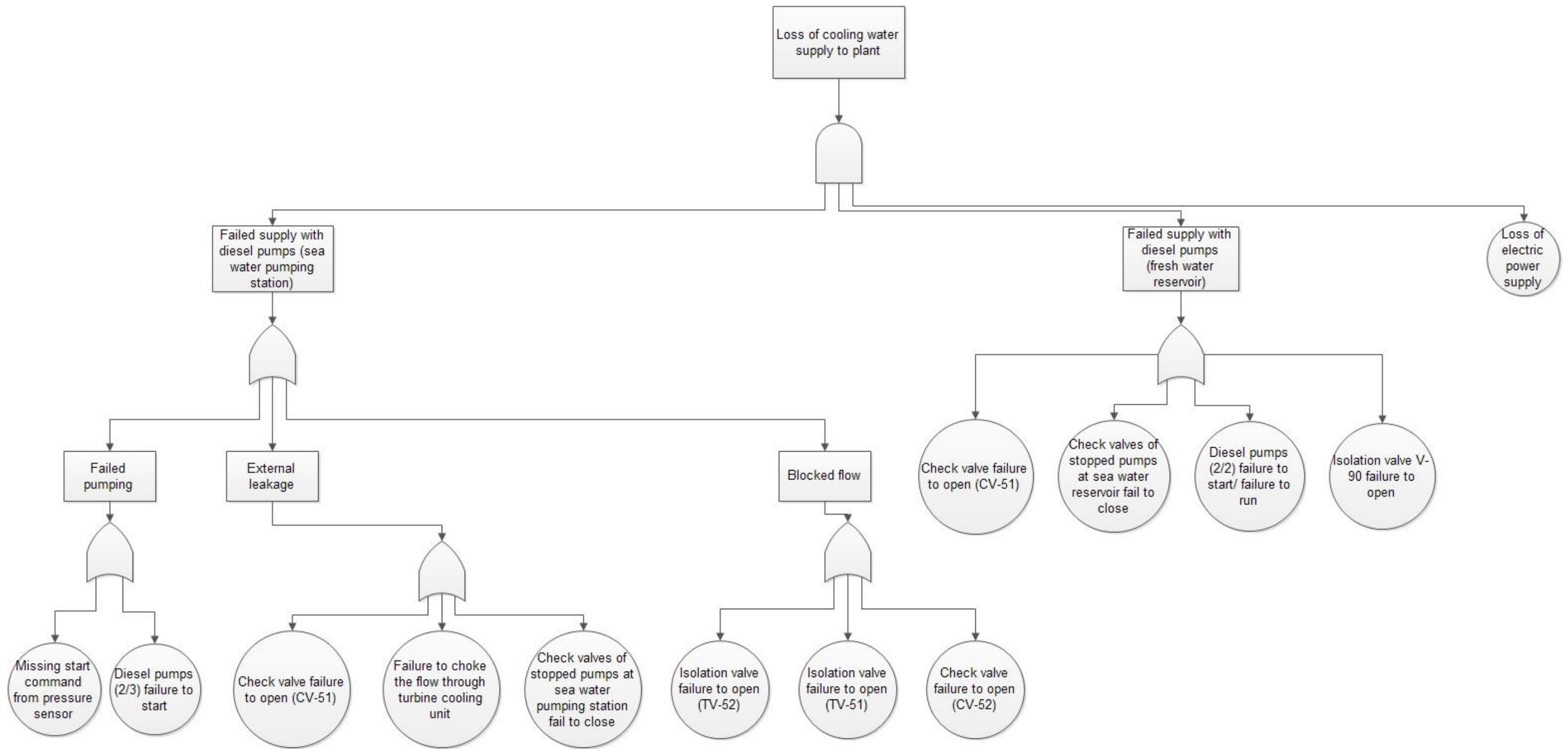
Figure 4.9 : Fault Tree Analysis of cooling water system failure due to power outage
