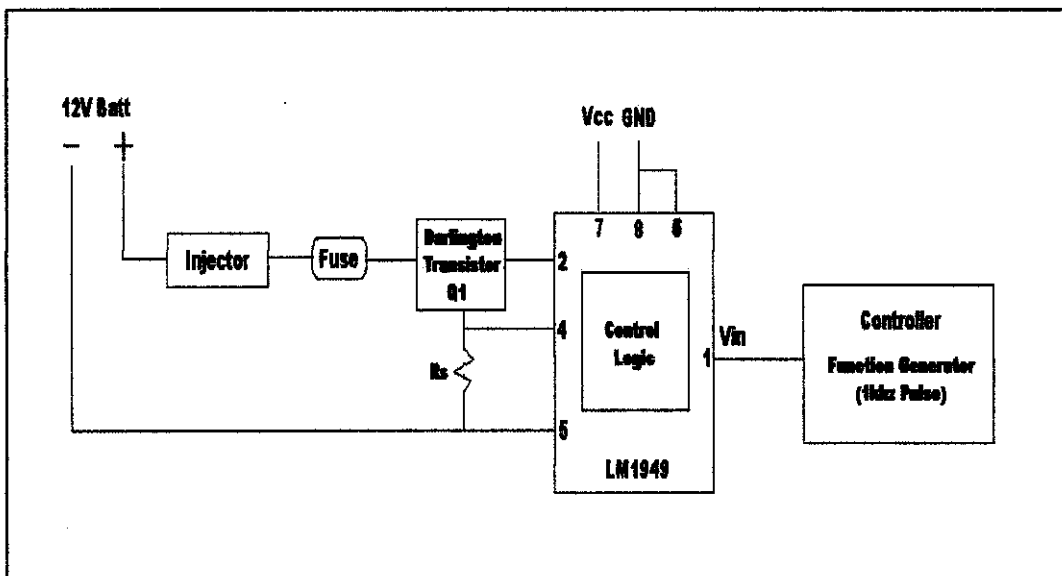
Figure 7: Equipments setup
