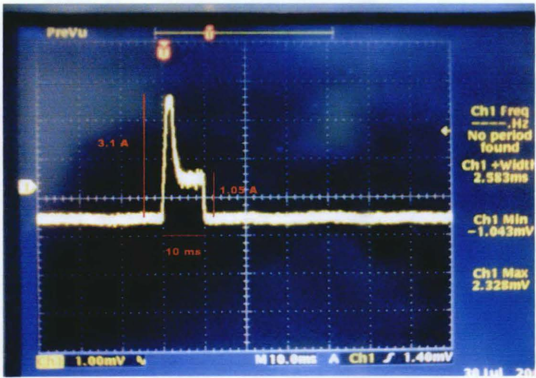
Figure 16: Injector current for 10ms pulse duration
