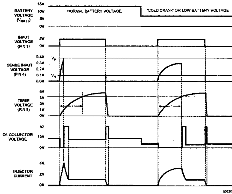
Figure 4: Typical circuit waveforms [1]
