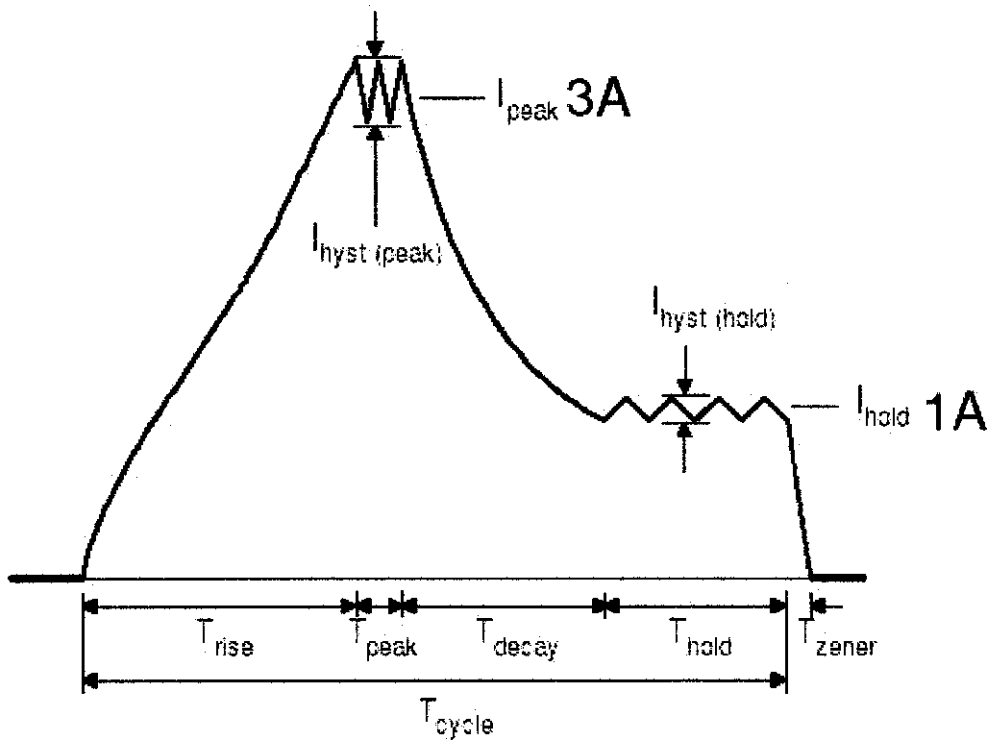
Figure 5: Closed up peak and hold waveform (Source image: Orbital documentation)
