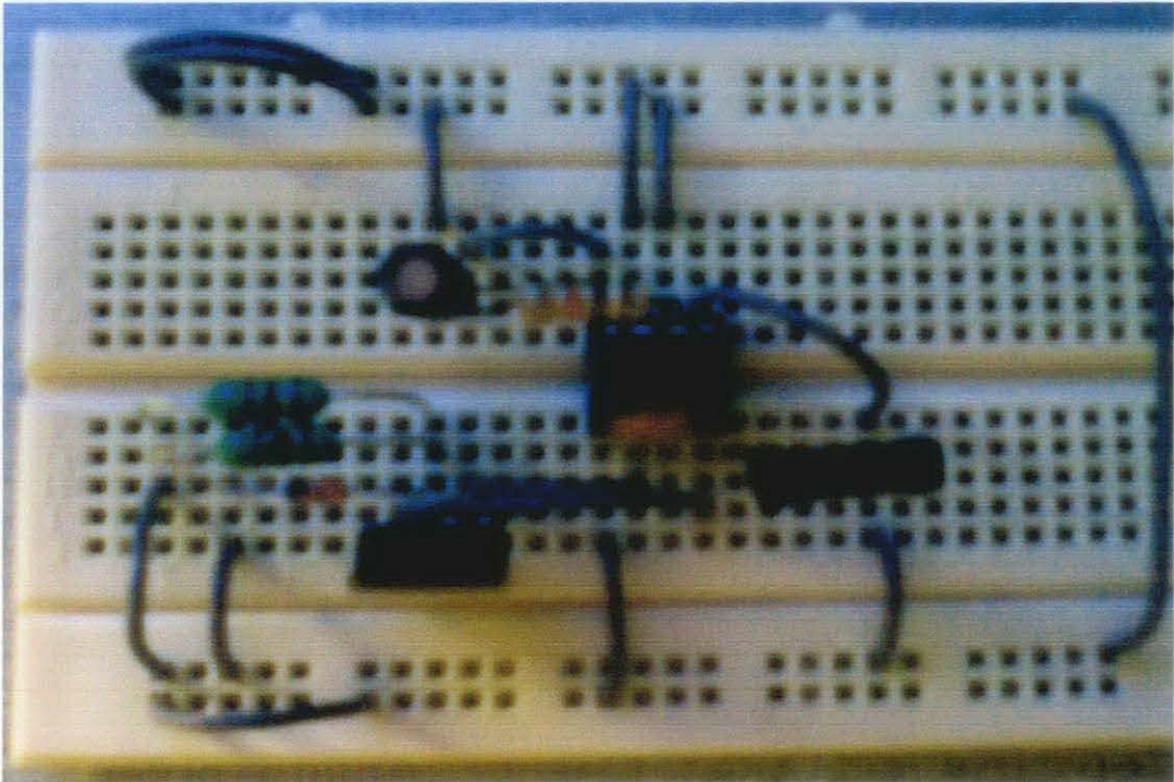
Figure 8: Circuit connection
