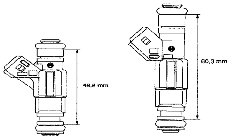
Figure 1: Different length of fuel injector [7]
