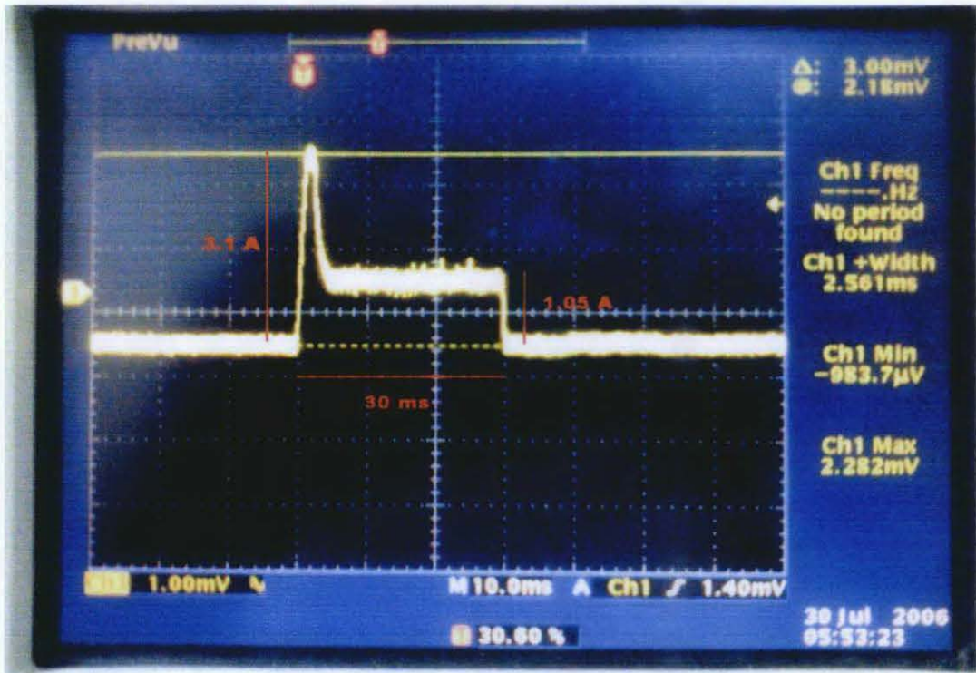
Figure 15: Injector current for 30ms pulse duration
