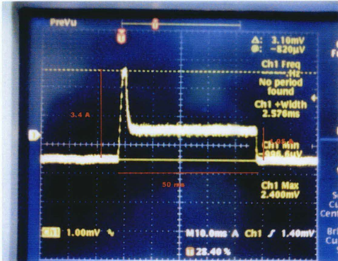
Figure 14: Injector current for 50ms pulse duration
