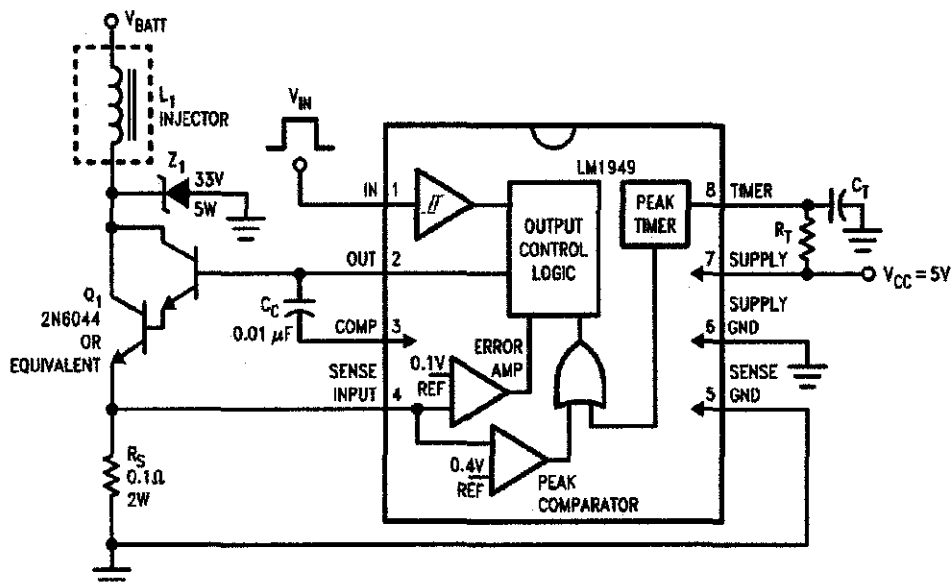
Figure 2: Typical application and test circuit [1]
