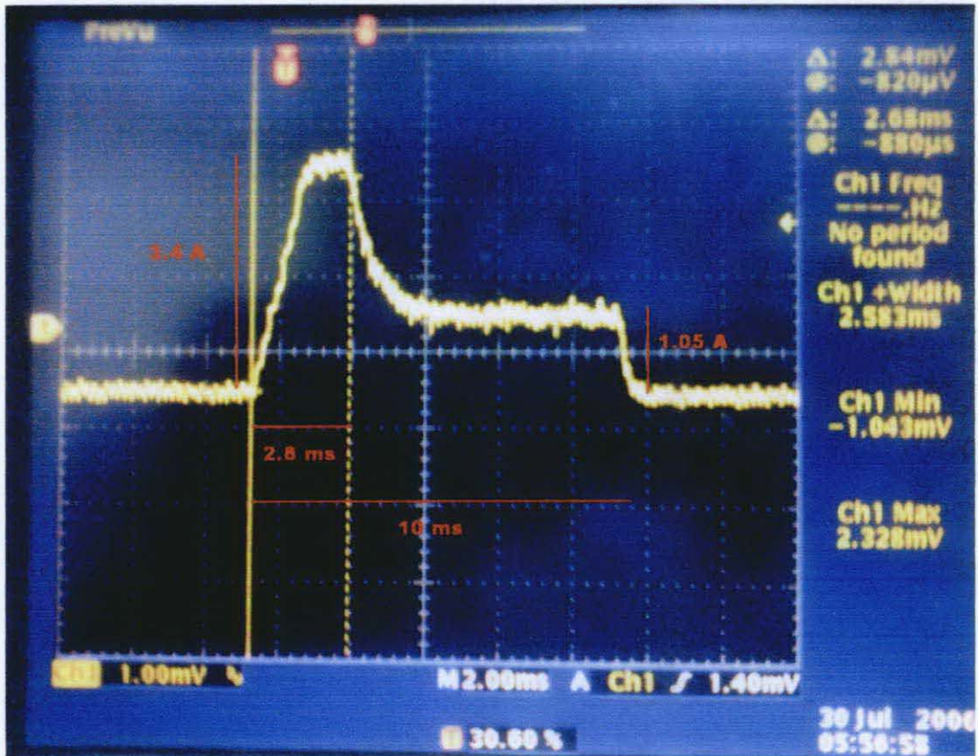
Figure 17: Close up for 10ms pulse duration
