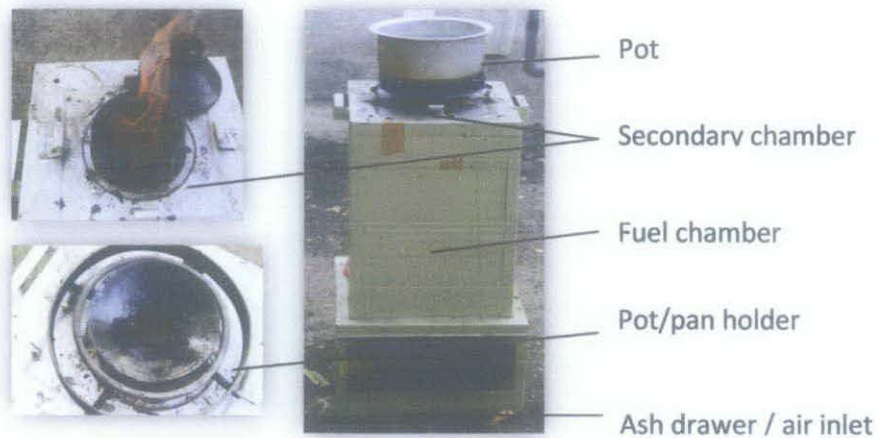
Figure 4.5: Operating Chemaco biomass cookstove
