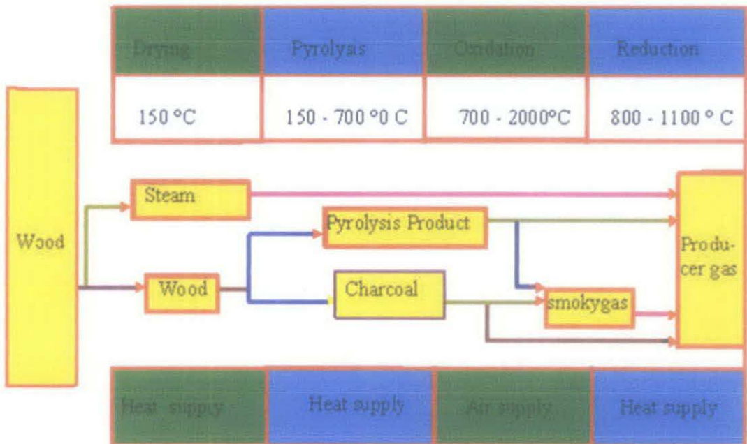
Figure 2.4: Conversion processes of biomass into producer gas (Basu, 2010)
