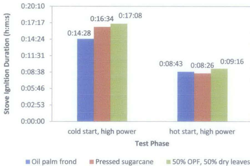
Figure 4.4: Stove ignition duration
