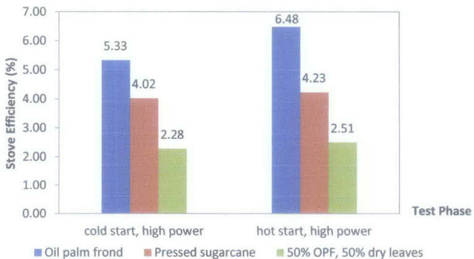
Figure 4.3: Stove efficiency with different types of fuel
