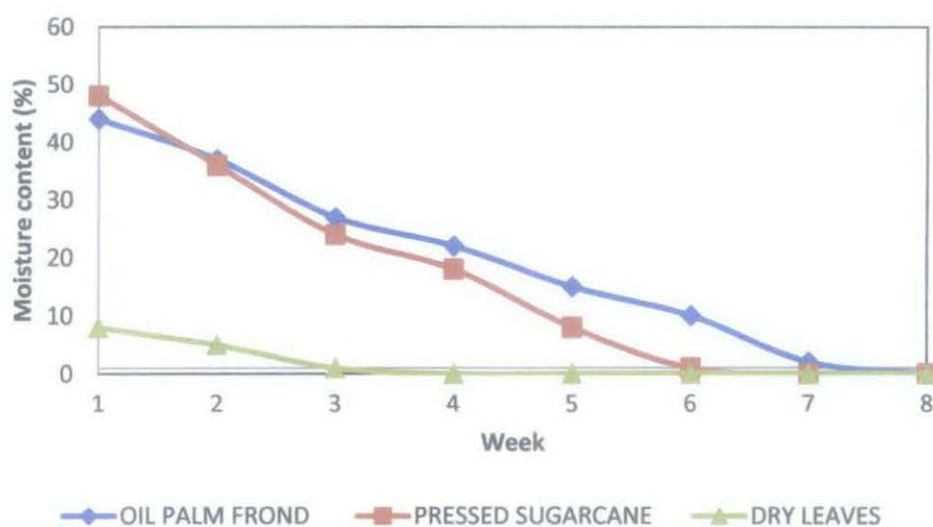
Figure 3.10: Fuels drying duration
