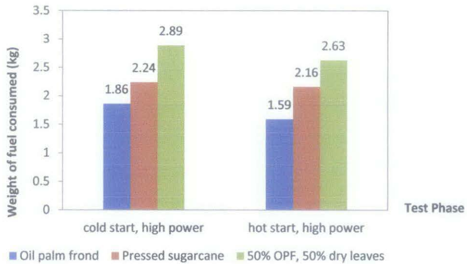
Figure 4.2 Weight of fuel consumed to boil 2.5 kg of water
