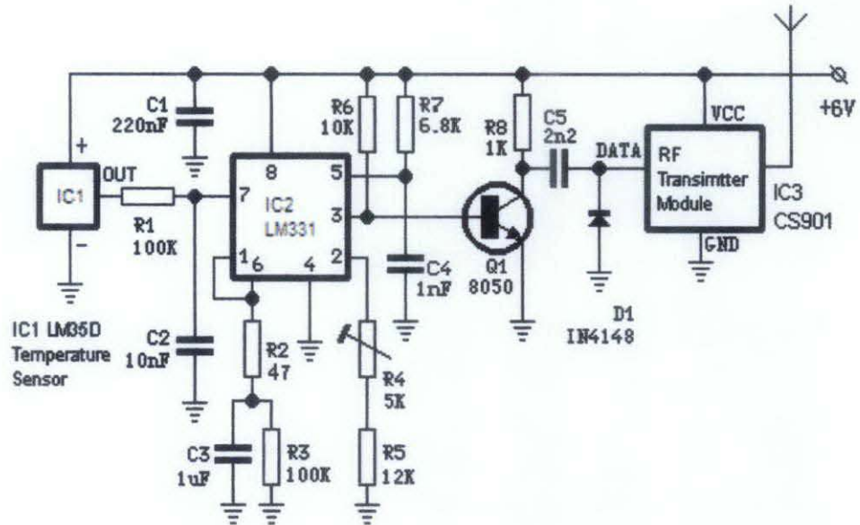
Figure 10: Transmitter (433MHz)
