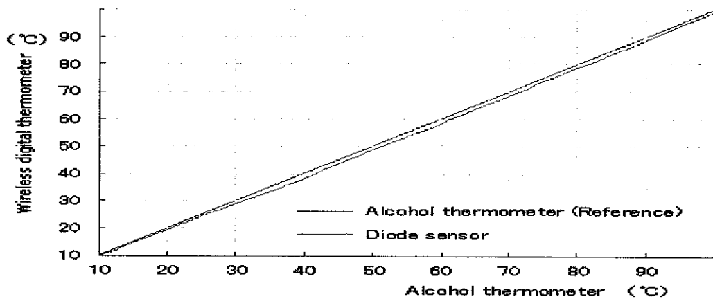
Figure 14: Comparison between the prototype and alcohol thermometer as reference temperature
