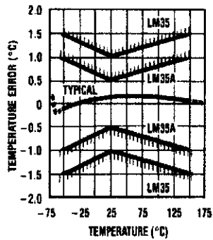
Accuracy vs. Temperature (Guaranteed)
