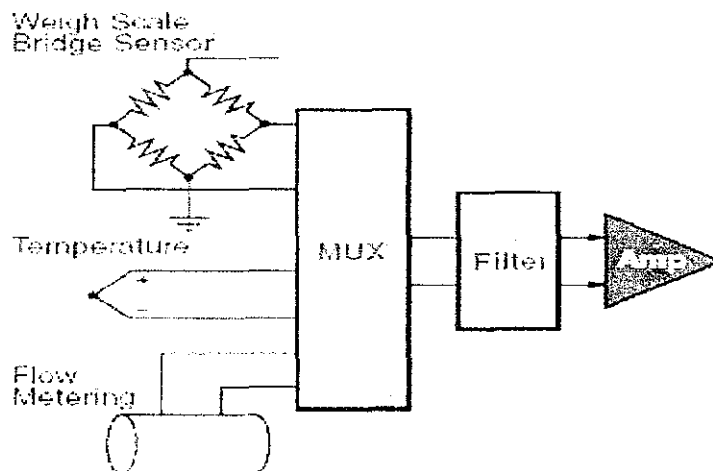
Figure 1: Simple Circuit on Temperature Controller
