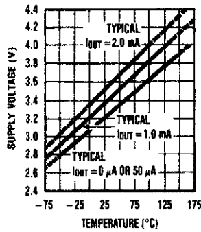
Minimum Supply Voltage vs. Temperature
