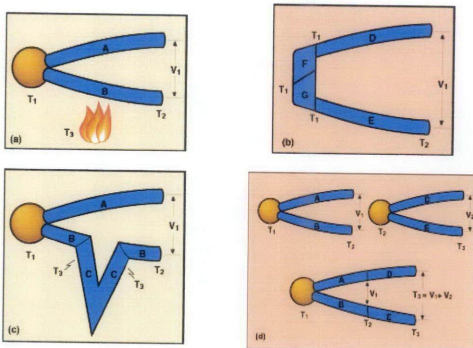
Figure 2: Thermocouple concept
