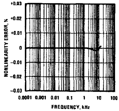
Nonlinearity Error
