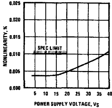
Nonlinearity Error vs. Power Supply Voltage
