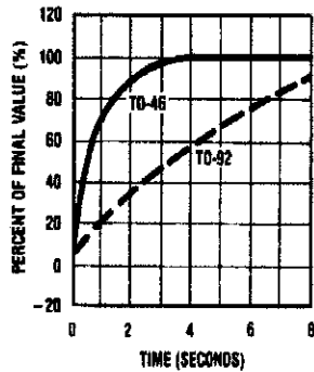
Thermal Response in Stirred Oil Bath
