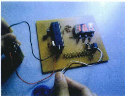
Figure 9: Circuit Operation when LM35 touched ice and hot water
