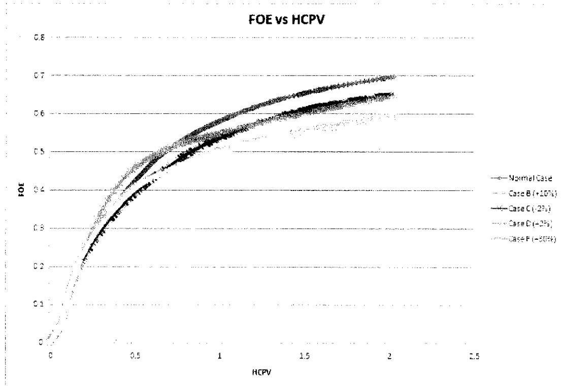
Figure 4.6 FOE vs HCPV
