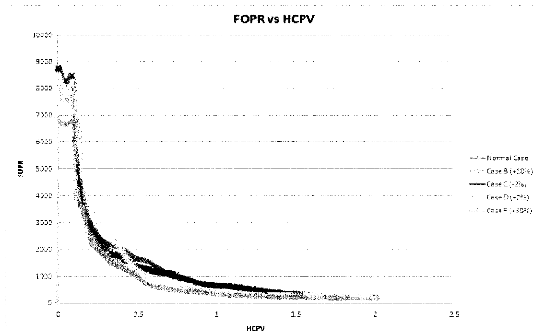
Figure 4.5 FOPR vs HCPV
