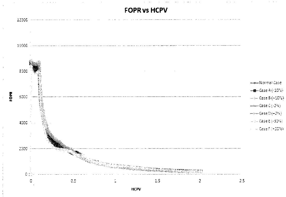
Figure 4.8 FOPR vs HCPV
