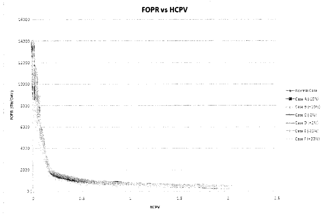
Figure 4.13 FOPR vs HCPV
