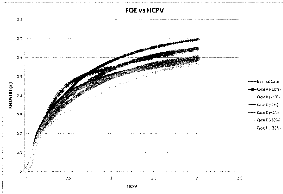
Figure 4.3 FOE vs HCPV
