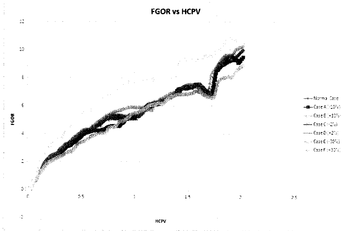
Figure 4.15 FGOR vs HCPV
