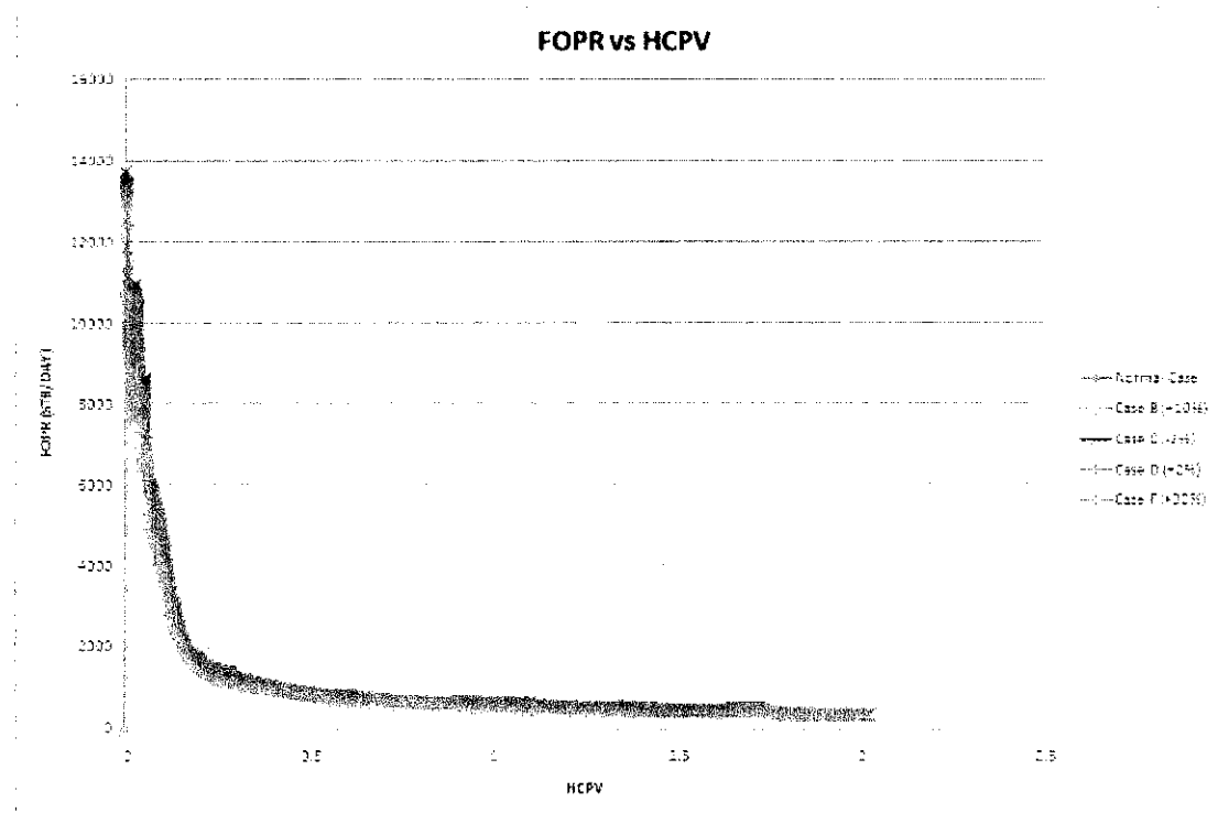
Figure 4.16 FOPR vs HCPV
