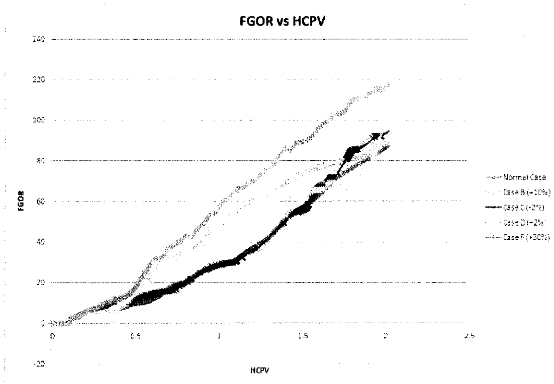
Figure 4.7 FGOR vs HCPV
