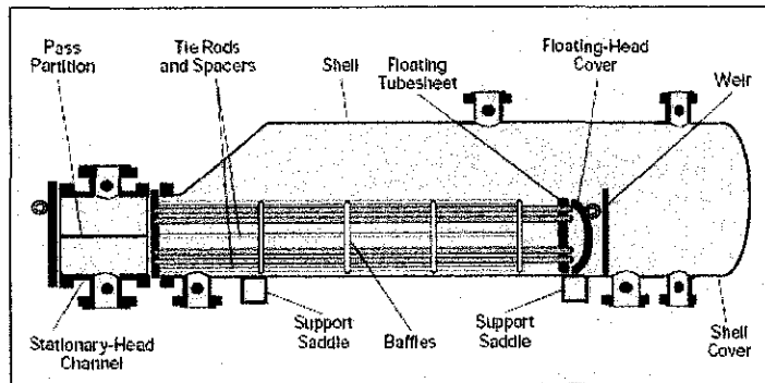
Figure C. Pull-through floating-head exchanger
