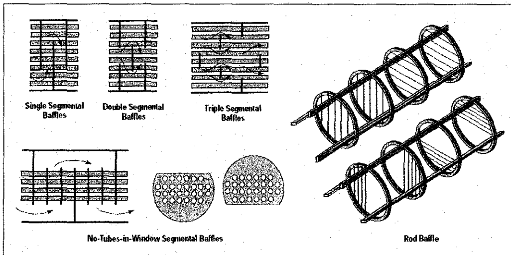
Figure 4 : Types of baffles [3].
