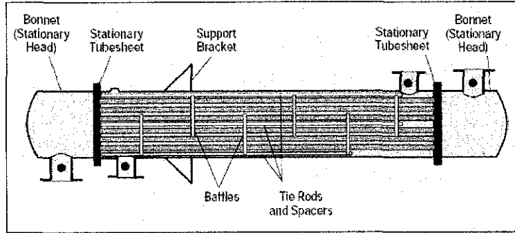
Figure A. Fixed-tubesheet heat exchanger.
