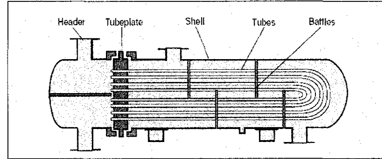
Figure B. U-tube heat exchanger.
