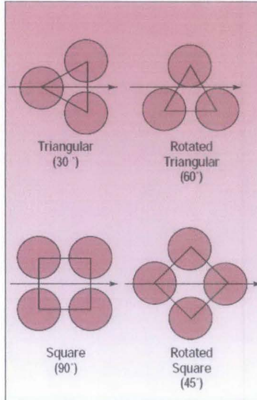
Figure 3 : Tube layout patterns [3]
