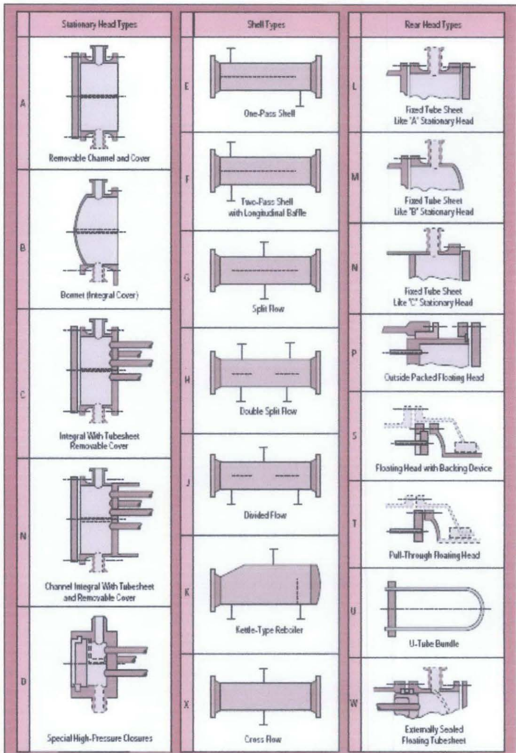
Figure 2 : TEMA designations for shell-and-tube heat exchangers [3].
